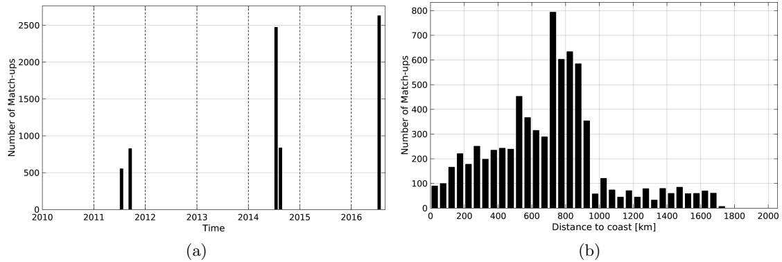
Figure 1: Number of match-ups between TSG-GOSUD-Research-vessel and SMOS-L3-ICDC-V3-MONTHLY-0.5DEG SSS as a function of time (a) and as function of the distance to coast (b) over the Gulf Stream Pi-MEP region and for the full satellite product period.
