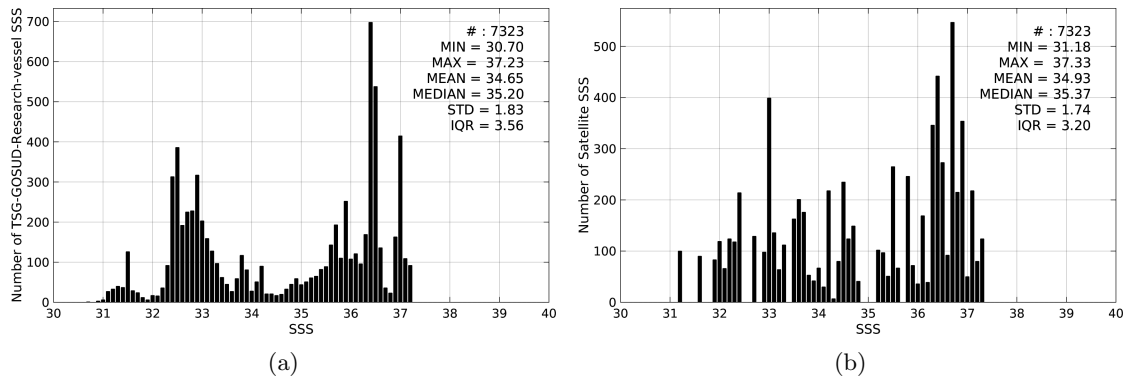
Figure 2: Histograms of SSS from TSG-GOSUD-Research-vessel (a) and SMOS-L3-ICDC-V3-MONTHLY-0.5DEG (b) considering all match-up pairs per bins of 0.1 over the Gulf Stream Pi-MEP region and for the full satellite product period.
