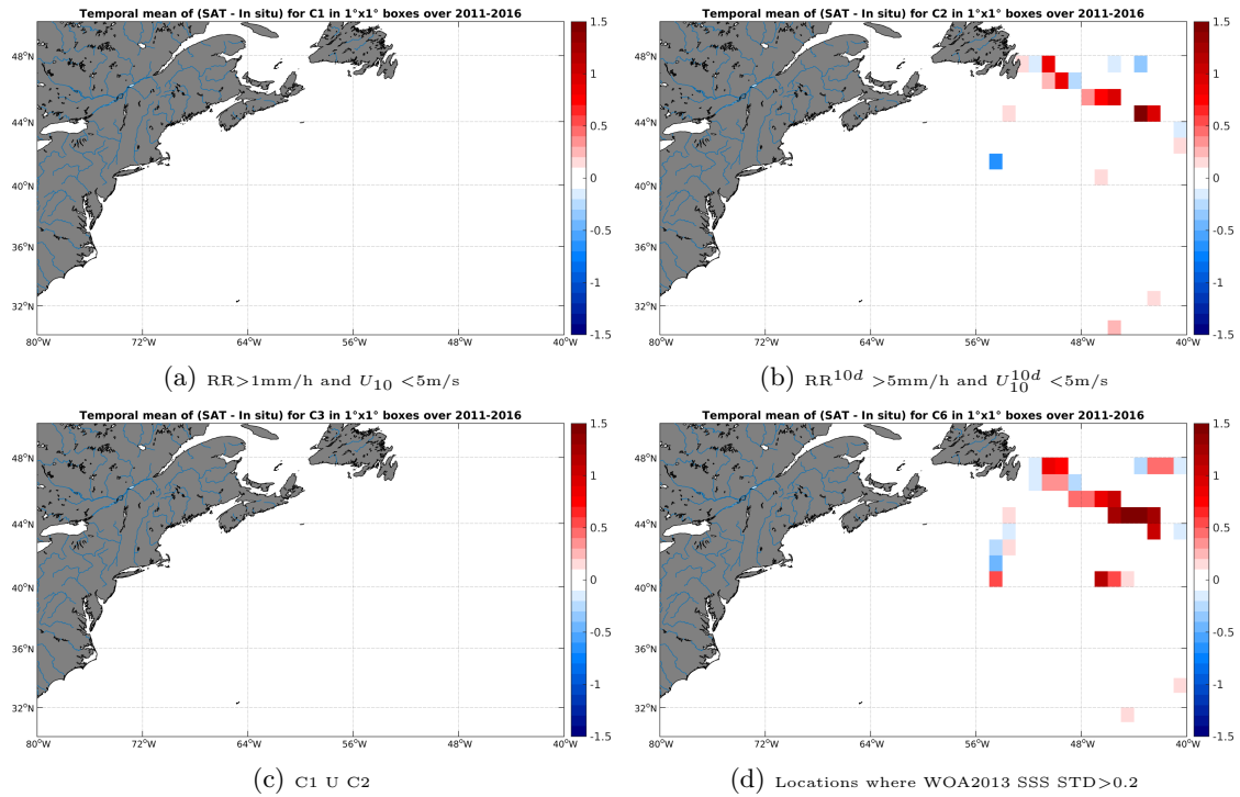
Figure 12: Temporal mean gridded over spatial boxes of size 1°x1° of \Delta SSS (SMOS-L3-ICDC-V3-MONTHLY-0.5DEG - TSG-GOSUD-Research-vessel) for 4 different subdatasets corresponding to: RR > 1mm/h and U_{10} < 5m/s (a), RR 10d > 5mm/h and U_{10}^{10d} < 5m/s (b), C1 U C2 (c), Locations where WOA2013 SSS STD > 0.2 (d).
