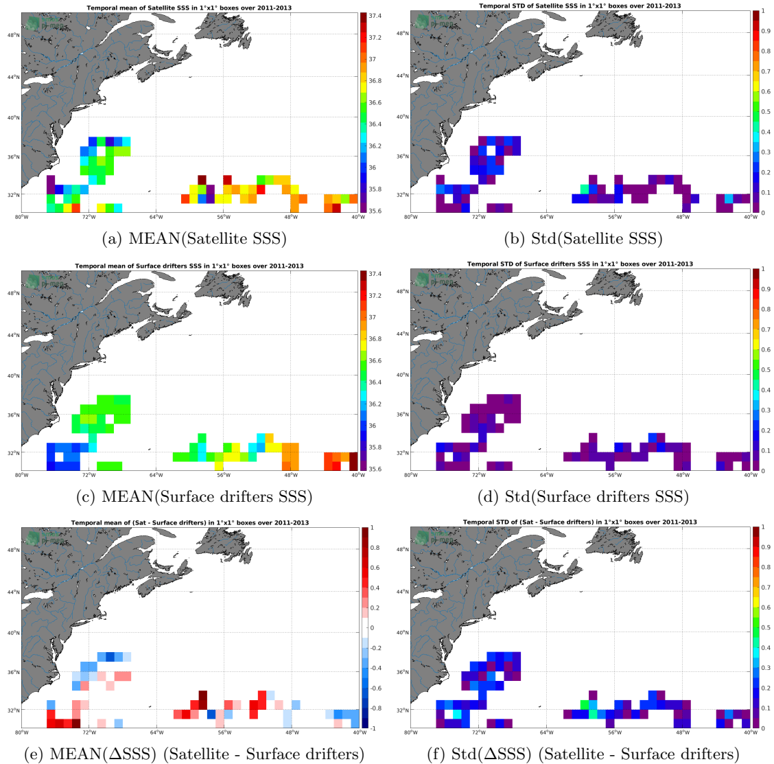
Figure 5: Temporal mean (left) and Std (right) of SSS from SMOS SSS L3 v3 Monthly (ICDC) (top), Surface drifters (middle), and of \Delta SSS (Satellite - Surface drifters). Only match-up pairs are used to generate these maps.
