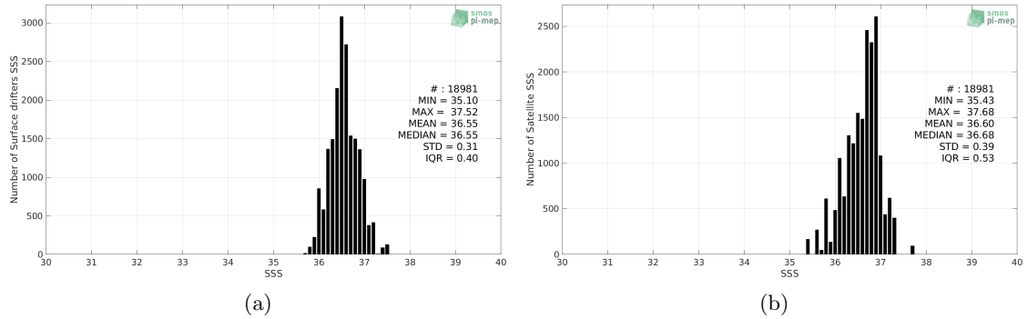
Figure 2: Histograms of SSS from Surface drifters (a) and SMOS SSS L3 v3 Monthly (ICDC) (b) considering all match-up pairs per bins of 0.1 over the Gulf Stream Pi-MEP region and for the full satellite product period.
