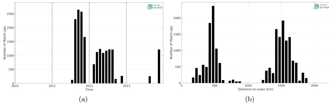
Figure 1: Number of match-ups between Surface drifters and SMOS SSS L3 v3 Monthly (ICDC) SSS as a function of time (a) and as function of the distance to coast (b) over the Gulf Stream Pi-MEP region and for the full satellite product period.
