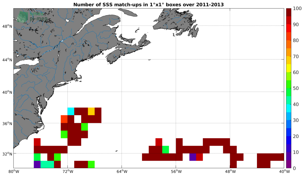
Figure 3: Number of SSS match-ups between Surface drifters SSS and the SMOS SSS L3 v3 Monthly (ICDC) SSS product for the Gulf Stream Pi-MEP region over 1^\circ \times 1^\circ boxes and for the full satellite product period.
