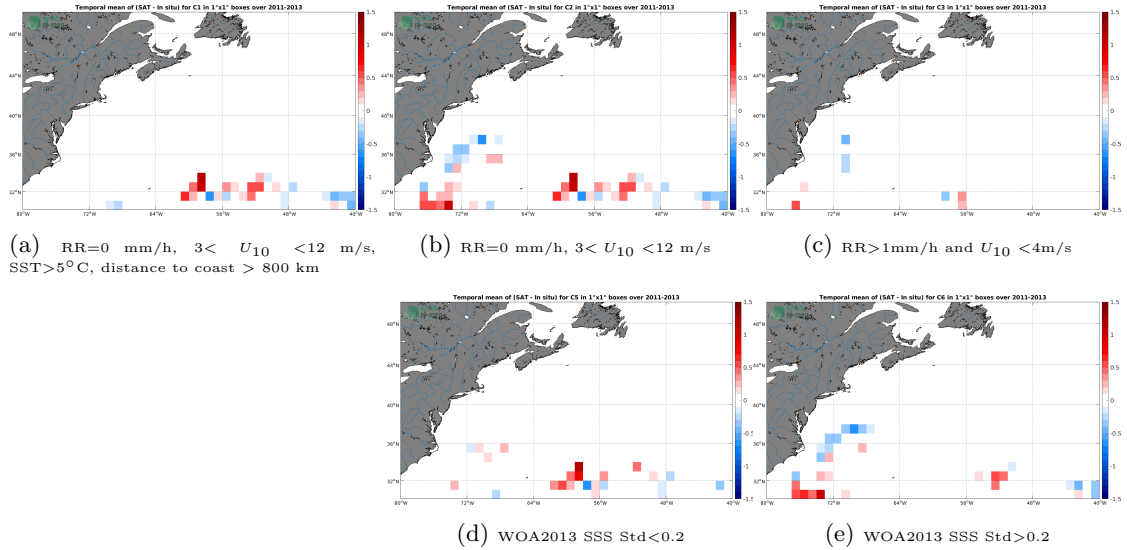
Figure 11: Temporal mean gridded over spatial boxes of size 1^{\circ}\times 1^{\circ} of \Delta\text{SSS} (SMOS SSS L3 v3 Monthly (ICDC) - Surface drifters) for 5 different subdatasets corresponding to:RR=0 mm/h, 3 < U_{10} < 12 m/s, SST > 5^{\circ}\text{C} , distance to coast > 800 km (a), RR=0 mm/h, 3 < U_{10} < 12 m/s (b), RR > 1 mm/h and U_{10} < 4 m/s (c), WOA2013 SSS Std < 0.2 (d), WOA2013 SSS Std > 0.2 (e).
