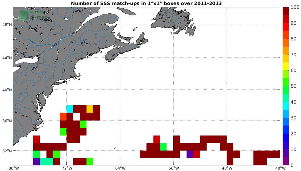
Figure 3: Number of SSS match-ups between Surface drifters SSS and the SMOS SSS L3 v3 Monthly (ICDC) SSS product for the Gulf Stream Pi-MEP region over 1°x1° boxes and for the full satellite product period.
