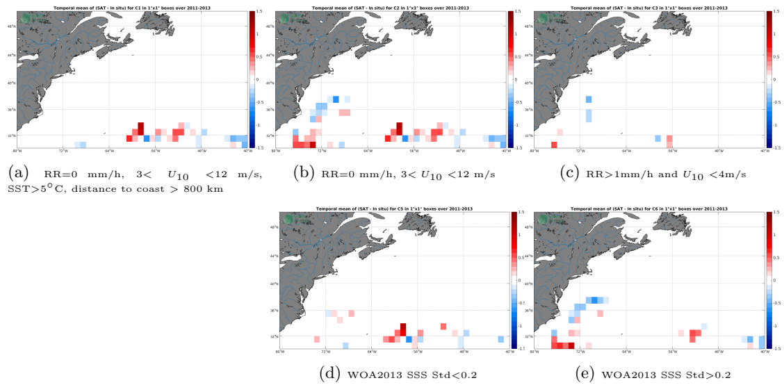
Figure 11: Temporal mean gridded over spatial boxes of size 1^\circ \times 1^\circ of \Delta SSS (SMOS-L3-ICDC-V3-MONTHLY-0.5DEG - Surface drifters) for 5 different subdatasets corresponding to: RR=0 mm/h, 3 < U_{10} < 12 m/s, SST > 5^\circ C , distance to coast > 800 km (a), RR=0 mm/h, 3 < U_{10} < 12 m/s (b), RR > 1 mm/h and U_{10} < 4 m/s (c), WOA2013 SSS Std < 0.2 (d), WOA2013 SSS Std > 0.2 (e).
