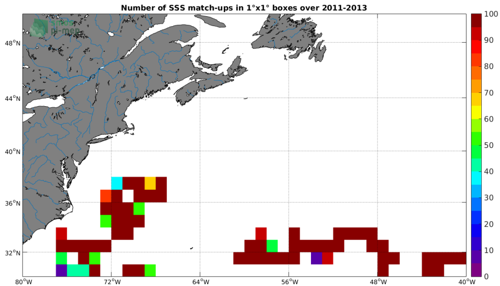
Figure 3: Number of SSS match-ups between Surface drifters SSS and the SMOS-L3-ICDC-V3-MONTHLY-0.5DEG SSS product for the Gulf Stream Pi-MEP region over 1^{\circ} \times 1^{\circ} boxes and for the full satellite product period.
