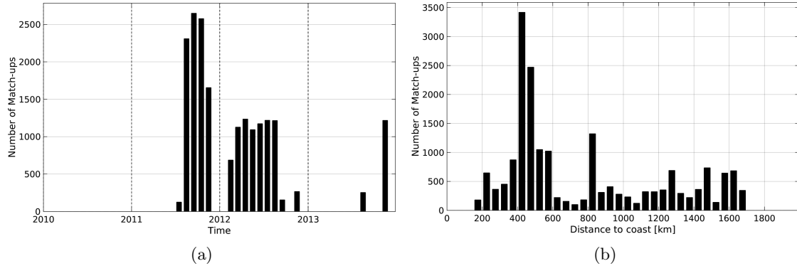
Figure 1: Number of match-ups between Surface drifters and SMOS-L3-ICDC-V3-MONTHLY-0.5DEG SSS as a function of time (a) and as function of the distance to coast (b) over the Gulf Stream Pi-MEP region and for the full satellite product period.
