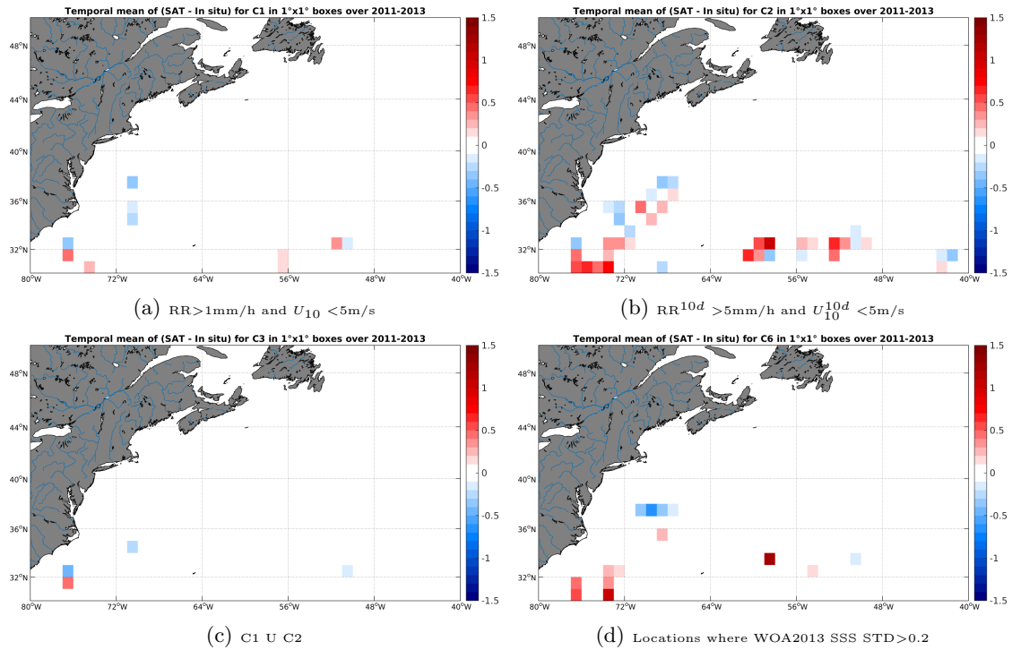
Figure 11: Temporal mean gridded over spatial boxes of size 1°x1° of \Delta SSS (SMOS-L3-ICDC-V3-MONTHLY-0.5DEG - Surface drifters) for 4 different subdatasets corresponding to:RR>1mm/h and U_{10} < 5\text{m/s} (a), RR^{10d} > 5\text{mm/h} and U_{10}^{10d} < 5\text{m/s} (b), C1 U C2 (c),Locations where WOA2013 SSS STD>0.2 (d).
