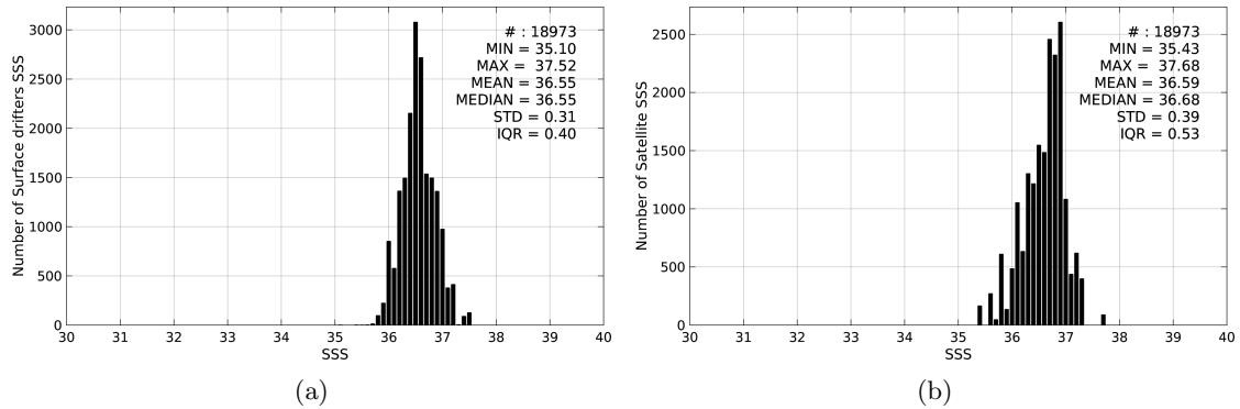
Figure 2: Histograms of SSS from Surface drifters (a) and SMOS-L3-ICDC-V3-MONTHLY-0.5DEG (b) considering all match-up pairs per bins of 0.1 over the Gulf Stream Pi-MEP region and for the full satellite product period.
