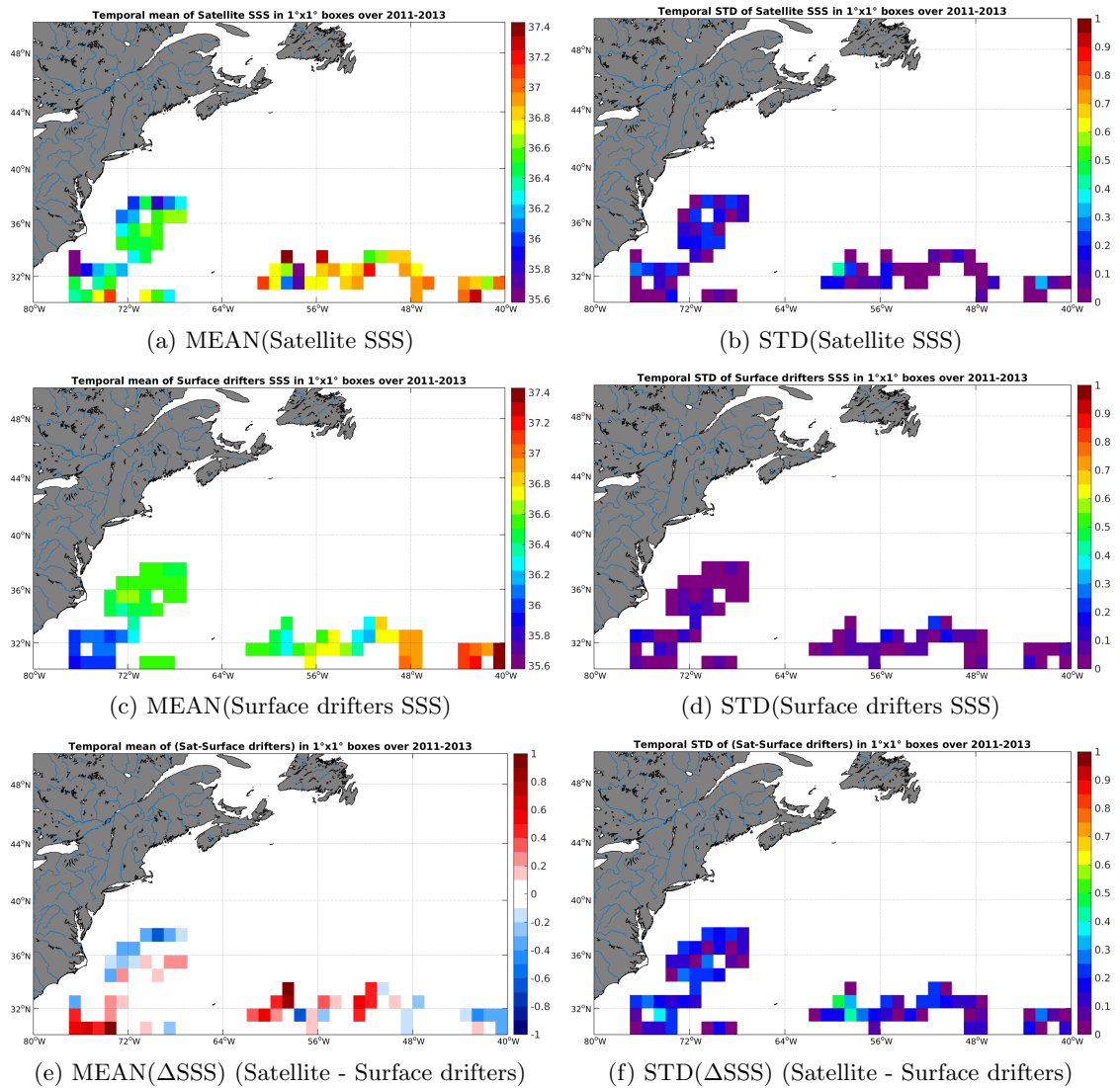
Figure 5: Temporal mean (left) and STD (right) of SSS from SMOS-L3-ICDC-V3-MONTHLY-0.5DEG (top), Surface drifters (middle), and of \Delta SSS (Satellite - Surface drifters). Only match-up pairs are used to generate these maps.
