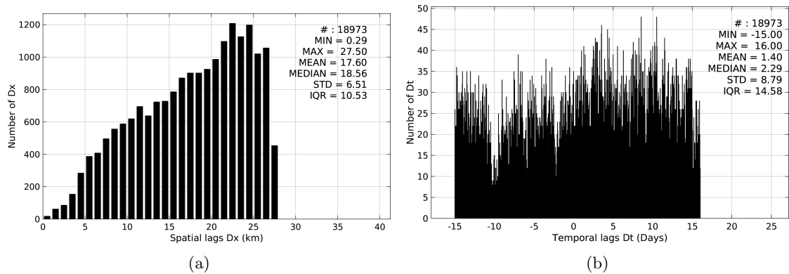
Figure 4: Histograms of the spatial (a) and temporal (b) lags between the time of the Surface drifters measurements and the date of the corresponding SMOS-L3-ICDC-V3-MONTHLY-0.5DEG SSS product.
