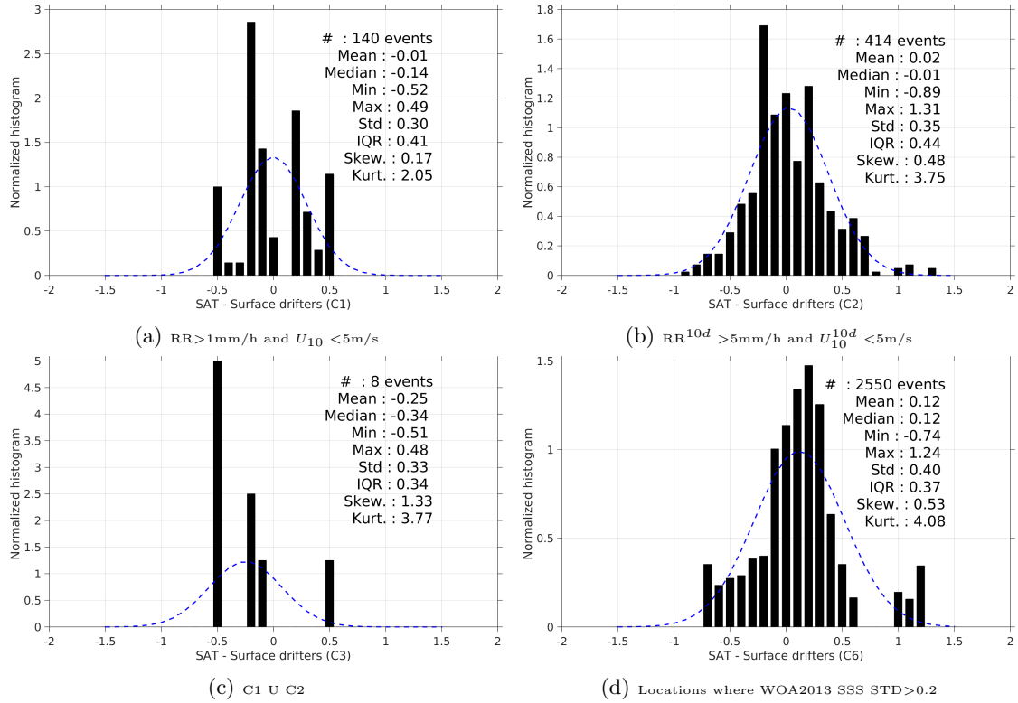
Figure 12: Normalized histogram of \Delta SSS (SMOS-L3-ICDC-V3-MONTHLY-0.5DEG - Surface drifters) for 6 different subdatasets corresponding to: RR > 1\text{mm/h} and U_{10} < 5\text{m/s} (a), RR^{10d} > 5\text{mm/h} and U_{10}^{10d} < 5\text{m/s} (b), C1 \cup C2 (c), Locations where WOA2013 SSS STD > 0.2 (d).
