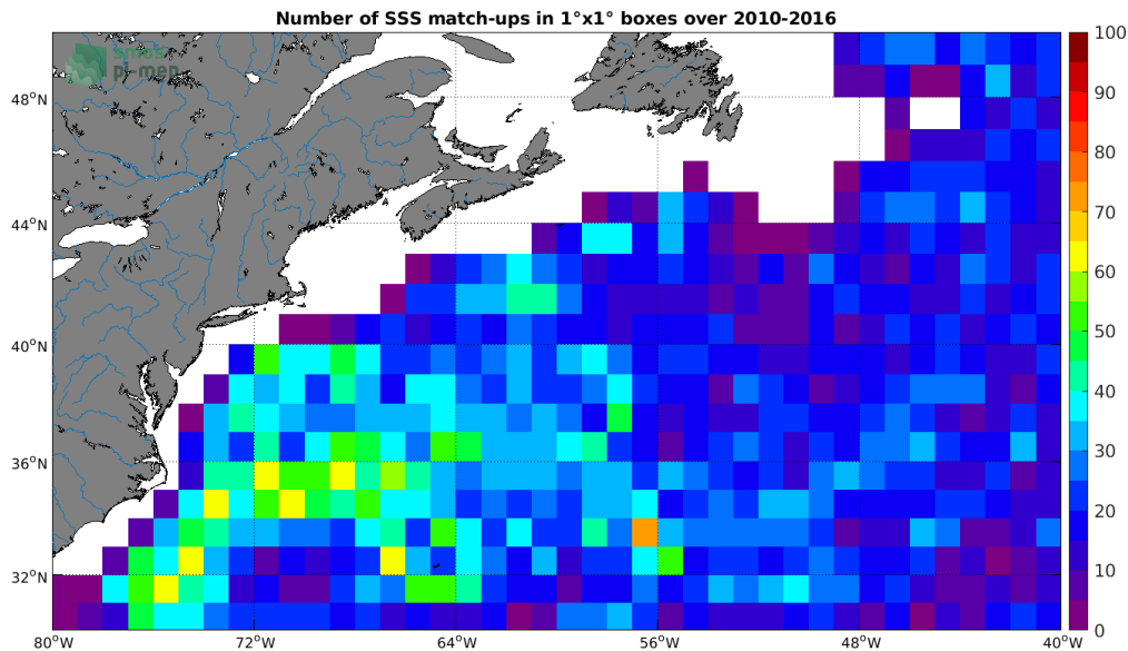
Figure 4: Number of SSS match-ups between Argo SSS and the SMOS SSS L3 v3 Monthly (ICDC) SSS product for the Gulf Stream Pi-MEP region over 1^\circ \times 1^\circ boxes and for the full satellite product period.
