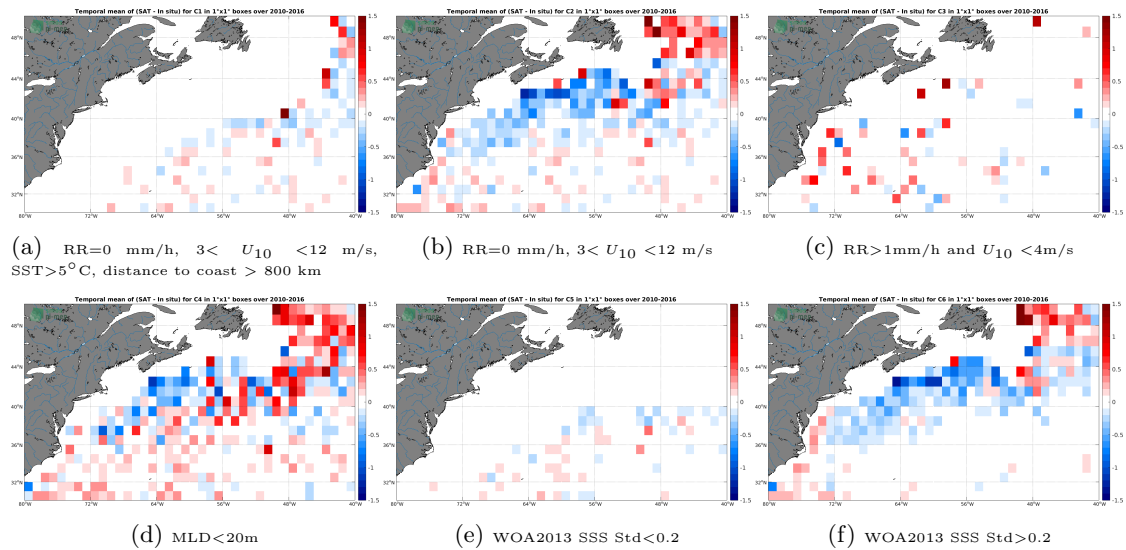
Figure 12: Temporal mean gridded over spatial boxes of size 1^\circ \times 1^\circ of \Delta SSS (SMOS SSS L3 v3 Monthly (ICDC) - Argo) for 6 different subdatasets corresponding to:RR=0 mm/h, 3 < U_{10} < 12 m/s, SST >5^\circ\text{C} , distance to coast > 800 km (a), RR=0 mm/h, 3 < U_{10} < 12 m/s (b), RR >1 mm/h and U_{10} < 4 m/s (c),MLD <20 m (d),WOA2013 SSS Std <0.2 (e),WOA2013 SSS Std >0.2 (f).
