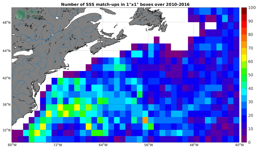
Figure 4: Number of SSS match-ups between Argos SSS and the SMOS SSS L3 v3 Monthly (ICDC) SSS product for the Gulf Stream Pi-MEP region over 1°x1° boxes and for the full satellite product period.
