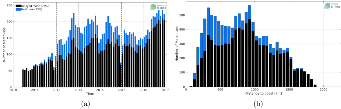
Figure 1: Number of match-ups between Argo and SMOS SSS L3 v3 Monthly (ICDC) SSS as a function of time (a) and as function of the distance to coast (b) over the Gulf Stream Pi-MEP region and for the full satellite product period.
