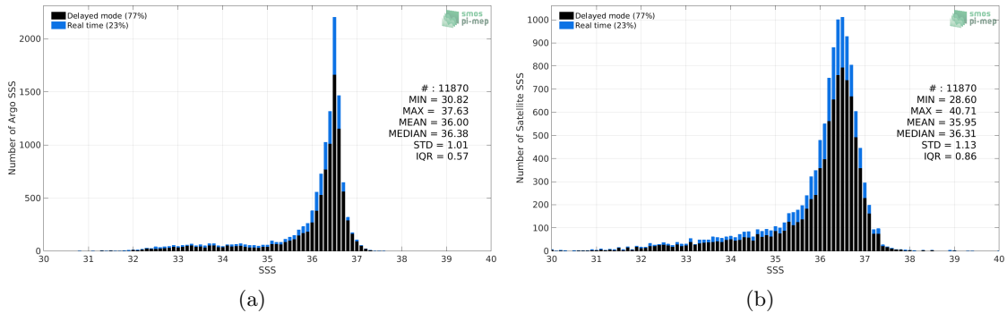
Figure 2: Histograms of SSS from Argo (a) and SMOS SSS L3 v3 Monthly (ICDC) (b) considering all match-up pairs per bins of 0.1 over the Gulf Stream Pi-MEP region and for the full satellite product period.
