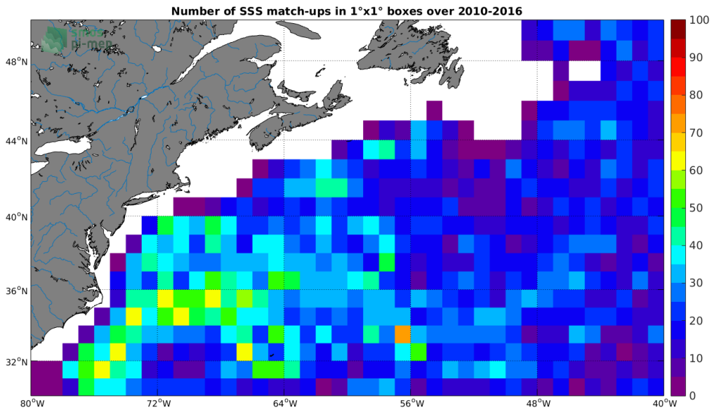
Figure 4: Number of SSS match-ups between Argo SSS and the SMOS-L3-ICDC-V3-MONTHLY-0.5DEG SSS product for the Gulf Stream Pi-MEP region over 1^\circ \times 1^\circ boxes and for the full satellite product period.
