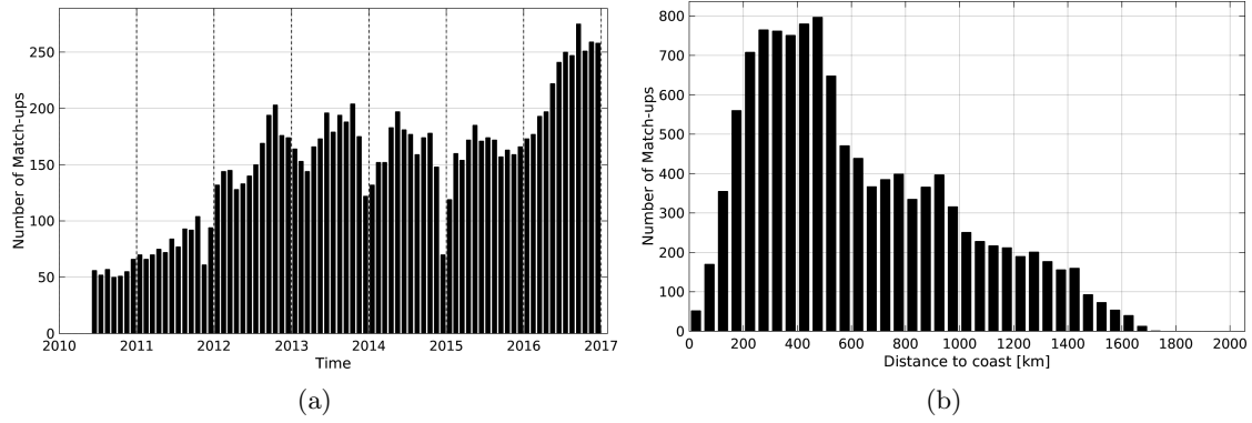
Figure 1: Number of match-ups between Argo and SMOS-L3-ICDC-V3-MONTHLY-0.5DEG SSS as a function of time (a) and as function of the distance to coast (b) over the Gulf Stream Pi-MEP region and for the full satellite product period.
