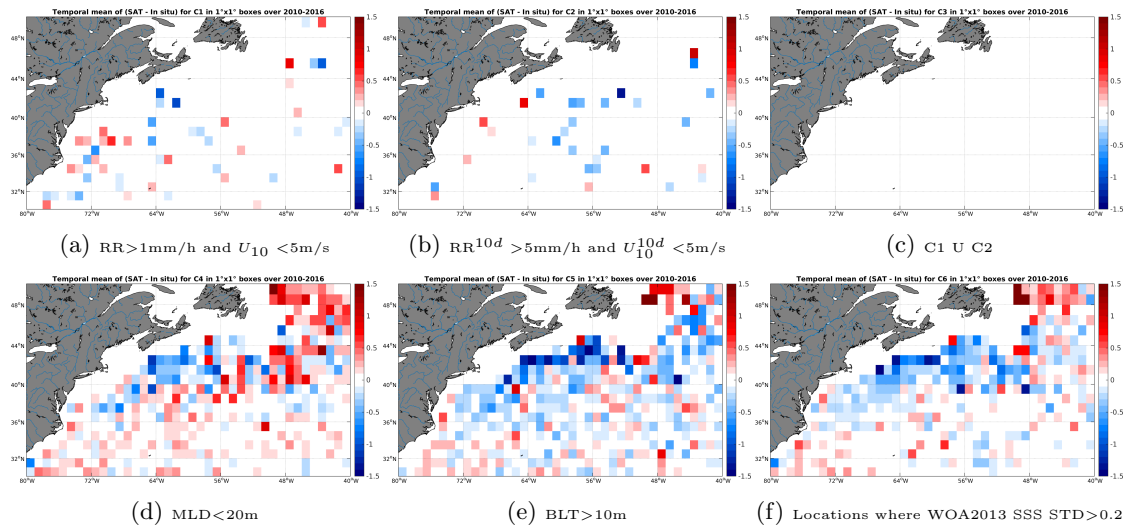
Figure 12: Temporal mean gridded over spatial boxes of size 1^\circ \times 1^\circ of \Delta SSS (SMOS-L3-ICDC-V3-MONTHLY-0.5DEG - Argo) for 6 different subdatasets corresponding to: RR > 1\text{mm/h} and U_{10} < 5\text{m/s} (a), RR^{10d} > 5\text{mm/h} and U_{10}^{10d} < 5\text{m/s} (b), C1 U C2 (c), MLD < 20\text{m} (d), BLT > 10\text{m} (e), Locations where WOA2013 SSS STD > 0.2 (f).
