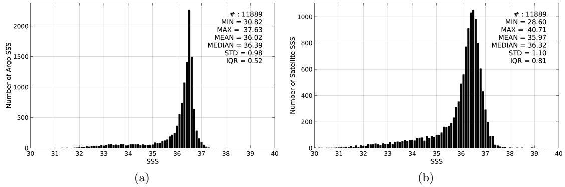
Figure 2: Histograms of SSS from Argo (a) and SMOS-L3-ICDC-V3-MONTHLY-0.5DEG (b) considering all match-up pairs per bins of 0.1 over the Gulf Stream Pi-MEP region and for the full satellite product period.
