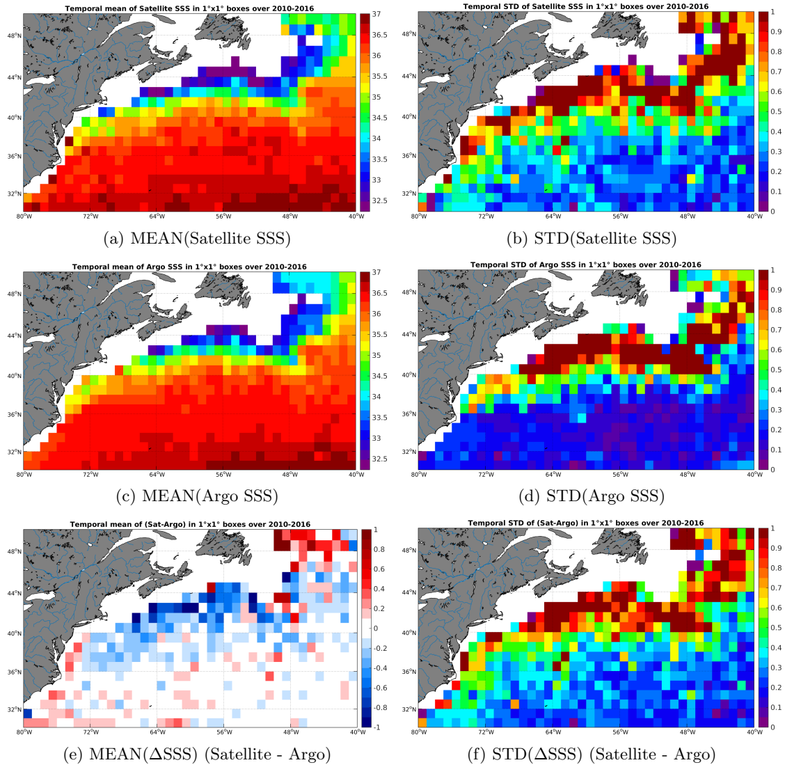
Figure 6: Temporal mean (left) and STD (right) of SSS from SMOS-L3-ICDC-V3-MONTHLY-0.5DEG (top), Argo (middle), and of \Delta SSS (Satellite - Argo). Only match-up pairs are used to generate these maps.
