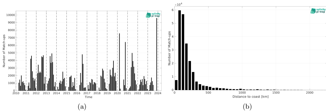
Figure 2: Number of match-ups between TSG (SAMOS) and SMOS SSS L2Q v331 - With FLAG (CMEMS-CATDS-CPDC) SSS as a function of time (a) and as function of the distance to coast (b) over the Gulf Stream Pi-MEP region and for the full satellite product period.
