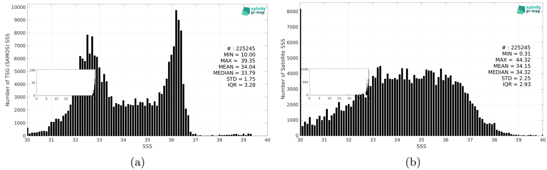
Figure 3: Histograms of SSS from TSG (SAMOS) (a) and SMOS SSS L2Q v331 - With FLAG (CMEMS-CATDS-CPDC) (b) considering all match-up pairs per bins of 0.1 over the Gulf Stream Pi-MEP region and for the full satellite product period.
