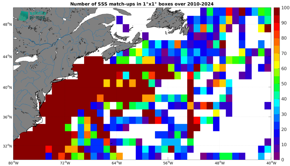
Figure 5: Number of SSS match-ups between TSG (SAMOS) SSS and the SMOS SSS L2Q v331 - With FLAG (CMEMS-CATDS-CPDC) SSS product for the Gulf Stream Pi-MEP region over 1^\circ \times 1^\circ boxes and for the full satellite product period.
