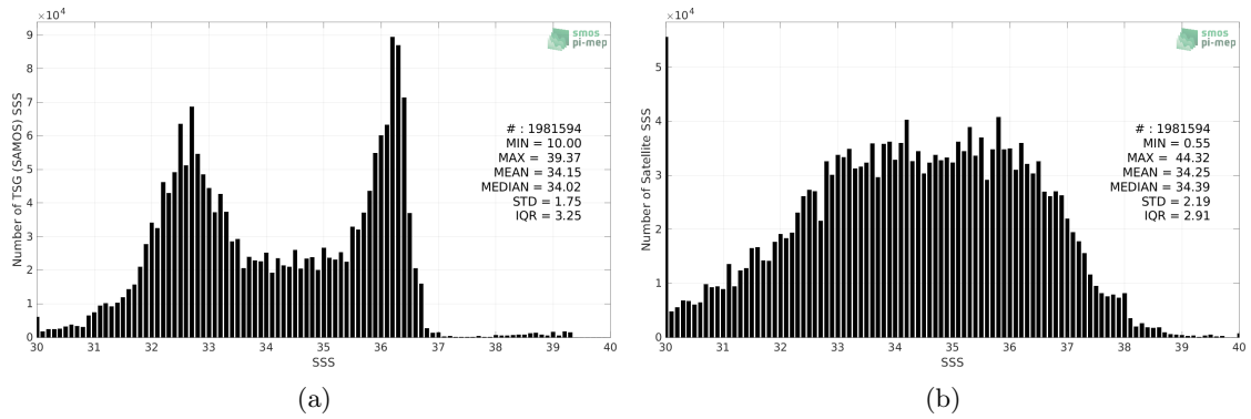
Figure 2: Histograms of SSS from TSG (SAMOS) (a) and SMOS SSS L2Q v331 - With FLAG (CMEMS-CATDS-CPDC) (b) considering all match-up pairs per bins of 0.1 over the Gulf Stream Pi-MEP region and for the full satellite product period.
