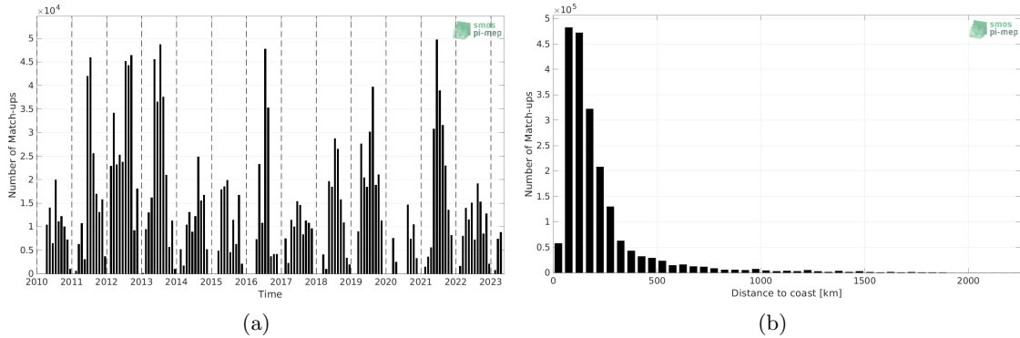
Figure 1: Number of match-ups between TSG (SAMOS) and SMOS SSS L2Q v331 - With FLAG (CMEMS-CATDS-CPDC) SSS as a function of time (a) and as function of the distance to coast (b) over the Gulf Stream Pi-MEP region and for the full satellite product period.
