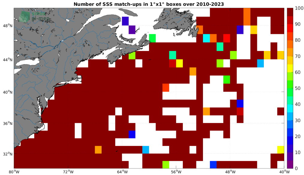
Figure 4: Number of SSS match-ups between TSG (SAMOS) SSS and the SMOS SSS L2Q v331 - With FLAG (CMEMS-CATDS-CPDC) SSS product for the Gulf Stream Pi-MEP region over 1^\circ \times 1^\circ boxes and for the full satellite product period.
