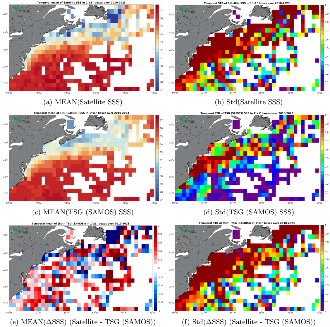
Figure 6: Temporal mean (left) and Std (right) of SSS from SMOS SSS L2Q v331 - With FLAG (CMEMS-CATDS-CPDC) (top), TSG (SAMOS) (middle), and of \Delta SSS (Satellite - TSG (SAMOS)). Only match-up pairs are used to generate these maps.
