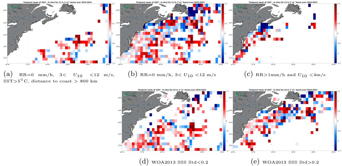
Figure 12: Temporal mean gridded over spatial boxes of size 1^{\circ}\times 1^{\circ} of \Delta\text{SSS} (SMOS SSS L2Q v331 - With FLAG (CMEMS-CATDS-CPDC) - TSG (SAMOS)) for 5 different subdatasets corresponding to:RR=0 mm/h, 3 < U_{10} < 12 m/s, SST >5^{\circ}\text{C} , distance to coast > 800 km (a), RR=0 mm/h, 3 < U_{10} < 12 m/s (b), RR >1 mm/h and U_{10} < 4 m/s (c), WOA2013 SSS Std <0.2 (d), WOA2013 SSS Std >0.2 (e).
