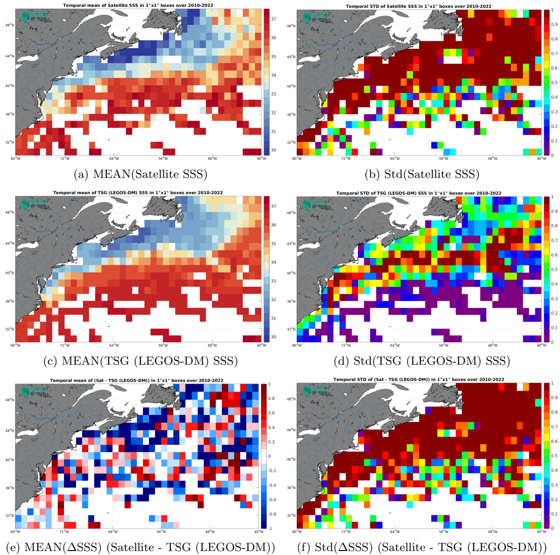
Figure 7: Temporal mean (left) and Std (right) of SSS from SMOS SSS L2Q v331 - With FLAG (CMEMS-CATDS-CPDC) (top), TSG (LEGOS-DM) (middle), and of \Delta SSS (Satellite - TSG (LEGOS-DM)). Only match-up pairs are used to generate these maps.
