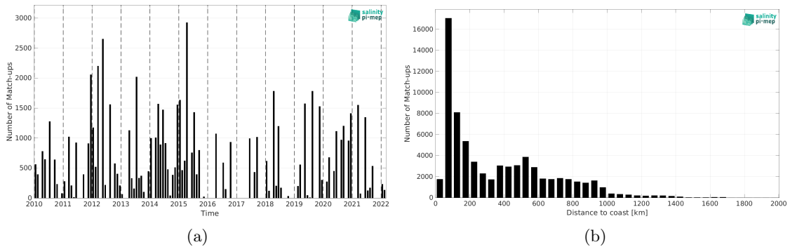
Figure 2: Number of match-ups between TSG (LEGOS-DM) and SMOS SSS L2Q v331 - With FLAG (CMEMS-CATDS-CPDC) SSS as a function of time (a) and as function of the distance to coast (b) over the Gulf Stream Pi-MEP region and for the full satellite product period.
