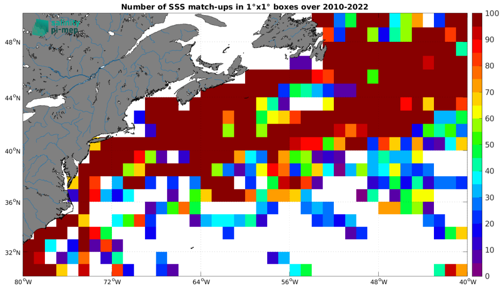
Figure 5: Number of SSS match-ups between TSG (LEGOS-DM) SSS and the SMOS SSS L2Q v331 - With FLAG (CMEMS-CATDS-CPDC) SSS product for the Gulf Stream Pi-MEP region over 1^\circ \times 1^\circ boxes and for the full satellite product period.
