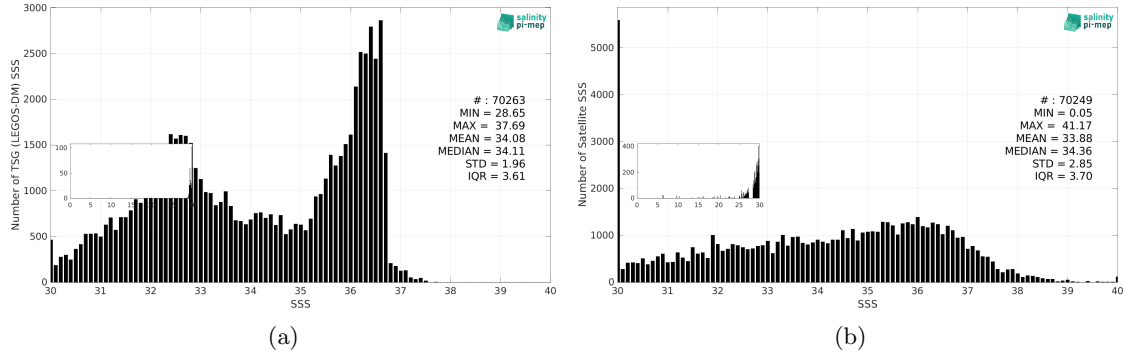
Figure 3: Histograms of SSS from TSG (LEGOS-DM) (a) and SMOS SSS L2Q v331 - With FLAG (CMEMS-CATDS-CPDC) (b) considering all match-up pairs per bins of 0.1 over the Gulf Stream Pi-MEP region and for the full satellite product period.
