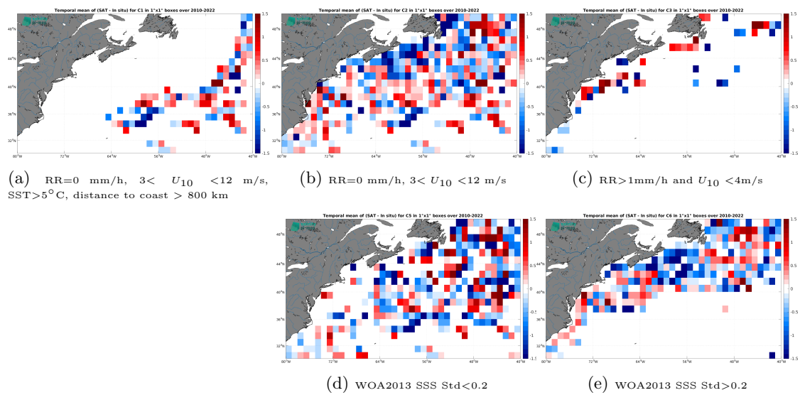
Figure 14: Temporal mean gridded over spatial boxes of size 1^\circ \times 1^\circ of \Delta SSS (SMOS SSS L2Q v331 - With FLAG (CMEMS-CATDS-CPDC) - TSG (LEGOS-DM)) for 5 different subdatasets corresponding to:RR=0 mm/h, 3 < U_{10} < 12 m/s, SST >5^\circ C, distance to coast > 800 km (a), RR=0 mm/h, 3 < U_{10} < 12 m/s (b), RR >1 mm/h and U_{10} < 4 m/s (c), WOA2013 SSS Std <0.2 (d), WOA2013 SSS Std >0.2 (e).
