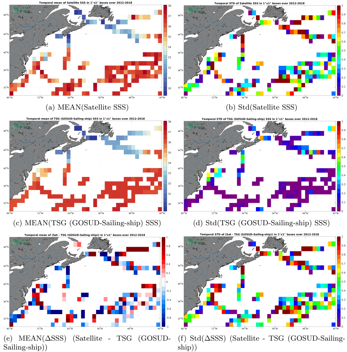
Figure 6: Temporal mean (left) and Std (right) of SSS from SMOS SSS L2Q v331 - With FLAG (CMEMS-CATDS-CPDC) (top), TSG (GOSUD-Sailing-ship) (middle), and of \Delta SSS (Satellite - TSG (GOSUD-Sailing-ship)). Only match-up pairs are used to generate these maps.
