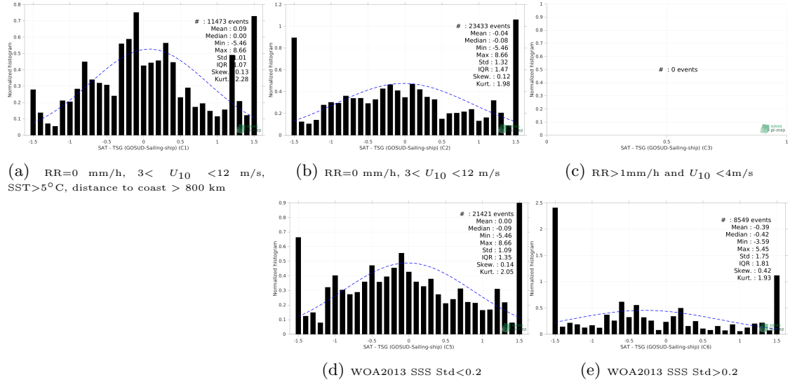
Figure 13: Normalized histogram of \Delta SSS (SMOS SSS L2Q v331 - With FLAG (CMEMS-CATDS-CPDC) - TSG (GOSUD-Sailing-ship)) for 5 different subdatasets corresponding to: RR=0 mm/h, 3 < U_{10} < 12 m/s, SST > 5°C, distance to coast > 800 km (a), RR=0 mm/h, 3 < U_{10} < 12 m/s (b), RR > 1mm/h and U_{10} < 4 m/s (c), WOA2013 SSS Std < 0.2 (d), WOA2013 SSS Std > 0.2 (e).
