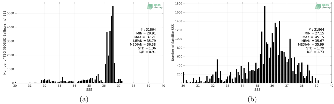
Figure 2: Histograms of SSS from TSG (GOSUD-Sailing-ship) (a) and SMOS SSS L2Q v331 - With FLAG (CMEMS-CATDS-CPDC) (b) considering all match-up pairs per bins of 0.1 over the Gulf Stream Pi-MEP region and for the full satellite product period.
