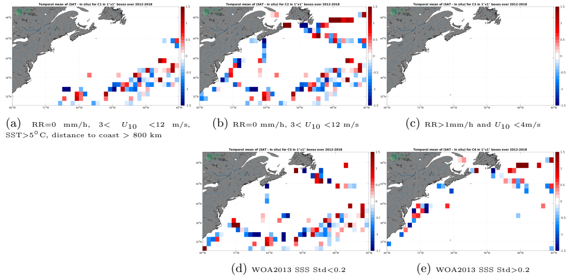
Figure 12: Temporal mean gridded over spatial boxes of size 1^{\circ}\times 1^{\circ} of \Delta SSS (SMOS SSS L2Q v331 - With FLAG (CMEMS-CATDS-CPDC) - TSG (GOSUD-Sailing-ship)) for 5 different subdatasets corresponding to:RR=0 mm/h, 3 < U_{10} < 12 m/s, SST >5^{\circ}\text{C} , distance to coast > 800 km (a), RR=0 mm/h, 3 < U_{10} < 12 m/s (b), RR >1 mm/h and U_{10} < 4 m/s (c), WOA2013 SSS Std <0.2 (d), WOA2013 SSS Std >0.2 (e).
