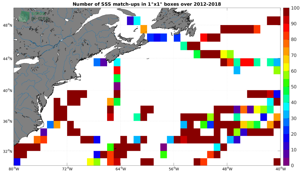
Figure 4: Number of SSS match-ups between TSG (GOSUD-Sailing-ship) SSS and the SMOS SSS L2Q v331 - With FLAG (CMEMS-CATDS-CPDC) SSS product for the Gulf Stream Pi-MEP region over 1^\circ \times 1^\circ boxes and for the full satellite product period.
