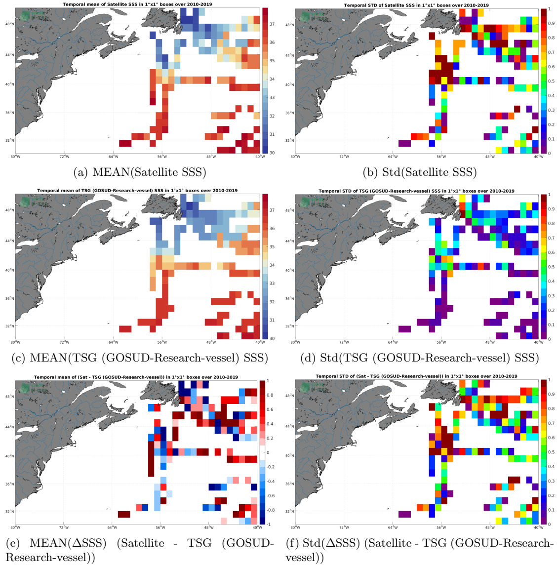
Figure 6: Temporal mean (left) and Std (right) of SSS from SMOS SSS L2Q v331 - With FLAG (CMEMS-CATDS-CPDC) (top), TSG (GOSUD-Research-vessel) (middle), and of \Delta SSS (Satellite - TSG (GOSUD-Research-vessel)). Only match-up pairs are used to generate these maps.
