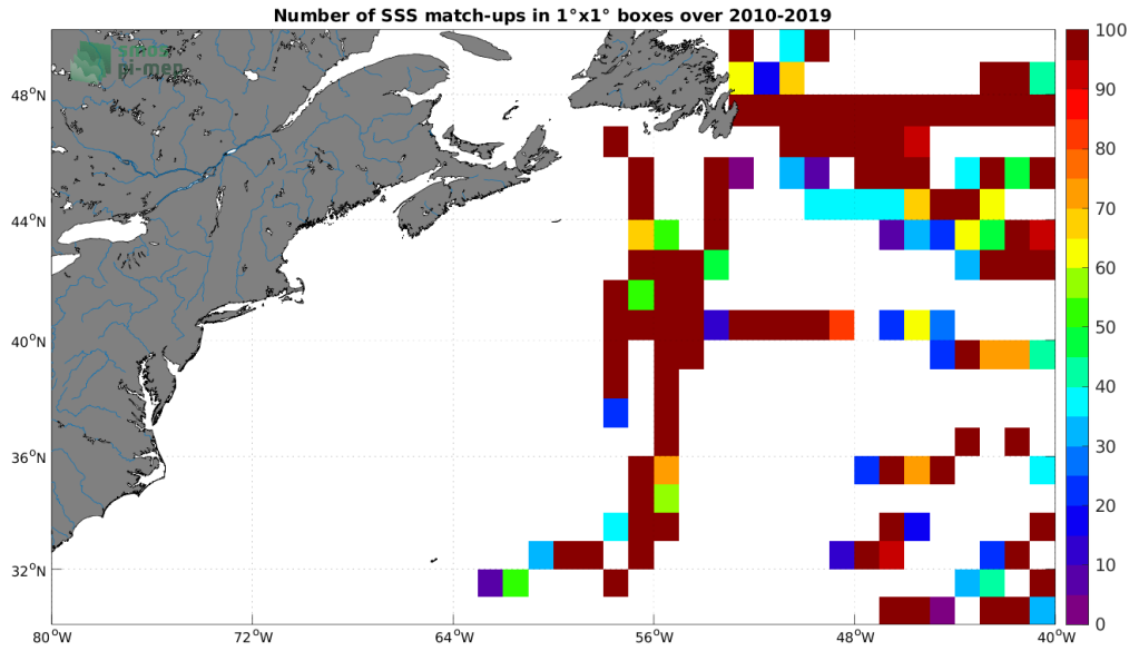
Figure 4: Number of SSS match-ups between TSG (GOSUD-Research-vessel) SSS and the SMOS SSS L2Q v331 - With FLAG (CMEMS-CATDS-CPDC) SSS product for the Gulf Stream Pi-MEP region over 1^\circ \times 1^\circ boxes and for the full satellite product period.
