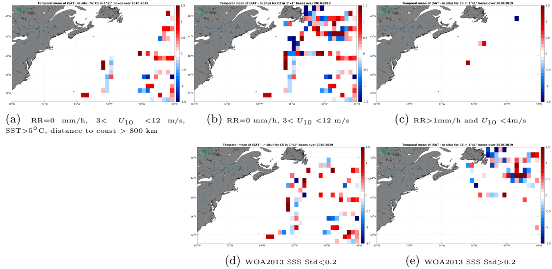
Figure 12: Temporal mean gridded over spatial boxes of size 1^\circ \times 1^\circ of \Delta SSS (SMOS SSS L2Q v331 - With FLAG (CMEMS-CATDS-CPDC) - TSG (GOSUD-Research-vessel)) for 5 different subdatasets corresponding to:RR=0 mm/h, 3 < U_{10} < 12 m/s, SST > 5^\circ\text{C} , distance to coast > 800 km (a), RR=0 mm/h, 3 < U_{10} < 12 m/s (b), RR > 1 mm/h and U_{10} < 4 m/s (c), WOA2013 SSS Std < 0.2 (d), WOA2013 SSS Std > 0.2 (e).
