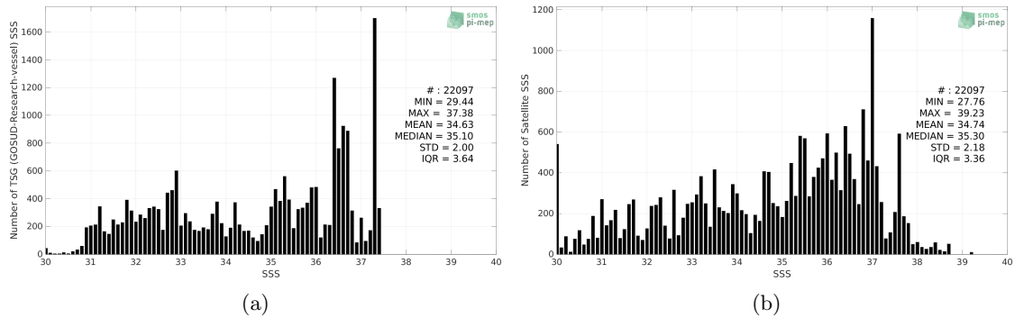
Figure 2: Histograms of SSS from TSG (GOSUD-Research-vessel) (a) and SMOS SSS L2Q v331 - With FLAG (CMEMS-CATDS-CPDC) (b) considering all match-up pairs per bins of 0.1 over the Gulf Stream Pi-MEP region and for the full satellite product period.
