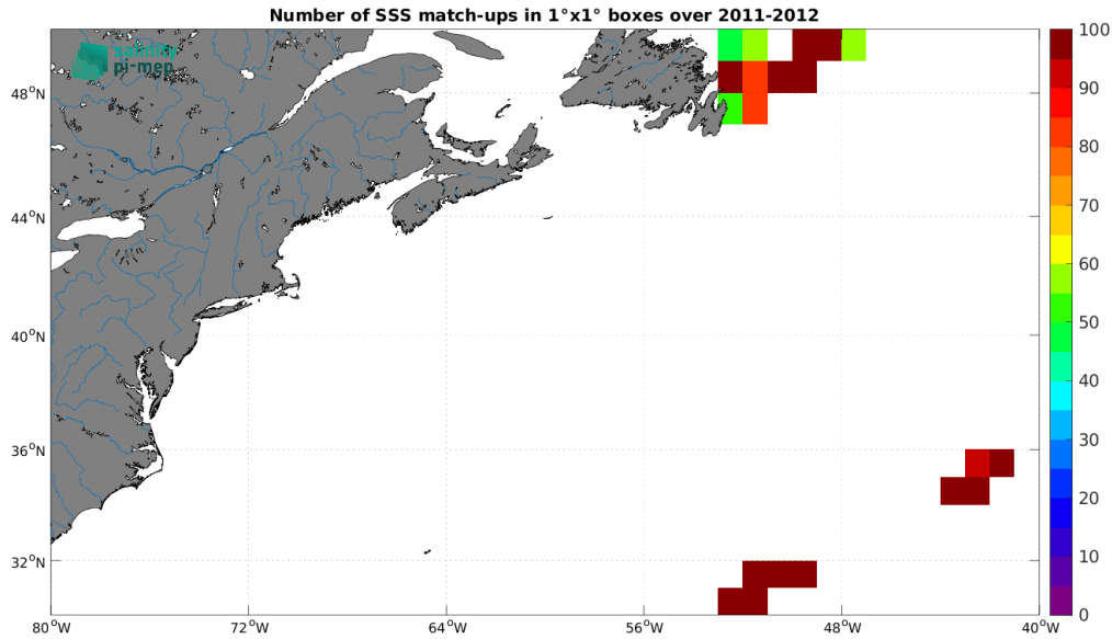
Figure 4: Number of SSS match-ups between TSG (CSIC-UTM) SSS and the SMOS SSS L2Q v331 - With FLAG (CMEMS-CATDS-CPDC) SSS product for the Gulf Stream Pi-MEP region over 1^\circ \times 1^\circ boxes and for the full satellite product period.
