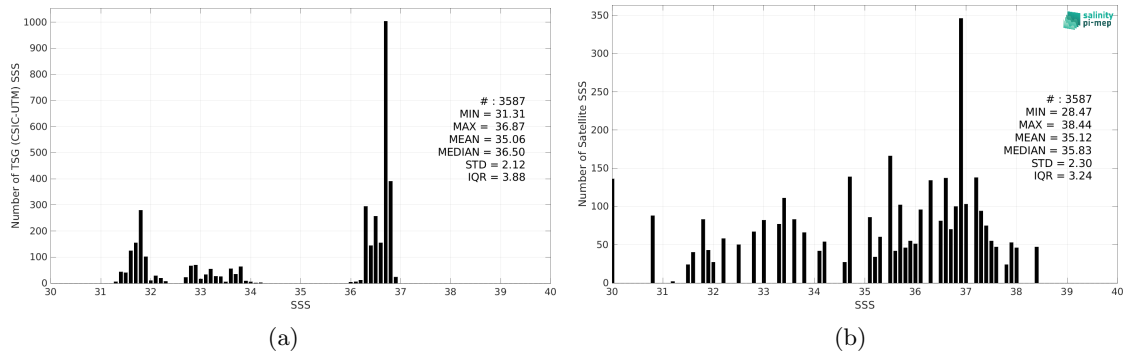
Figure 2: Histograms of SSS from TSG (CSIC-UTM) (a) and SMOS SSS L2Q v331 - With FLAG (CMEMS-CATDS-CPDC) (b) considering all match-up pairs per bins of 0.1 over the Gulf Stream Pi-MEP region and for the full satellite product period.
