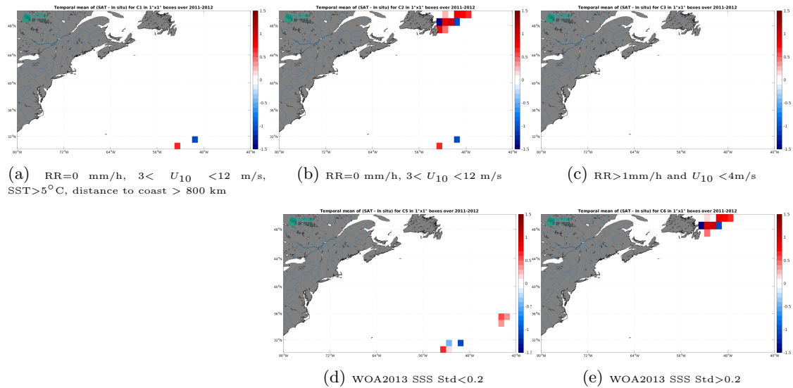
Figure 12: Temporal mean gridded over spatial boxes of size 1^{\circ}\times 1^{\circ} of \Delta\text{SSS} (SMOS SSS L2Q v331 - With FLAG (CMEMS-CATDS-CPDC) - TSG (CSIC-UTM)) for 5 different subdatasets corresponding to:RR=0 mm/h, 3 < U_{10} < 12 m/s, SST >5^{\circ}\text{C} , distance to coast > 800 km (a), RR=0 mm/h, 3 < U_{10} < 12 m/s (b), RR >1 mm/h and U_{10} < 4 m/s (c), WOA2013 SSS Std <0.2 (d), WOA2013 SSS Std >0.2 (e).
