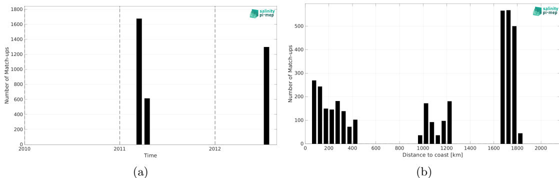
Figure 1: Number of match-ups between TSG (CSIC-UTM) and SMOS SSS L2Q v331 - With FLAG (CMEMS-CATDS-CPDC) SSS as a function of time (a) and as function of the distance to coast (b) over the Gulf Stream Pi-MEP region and for the full satellite product period.
