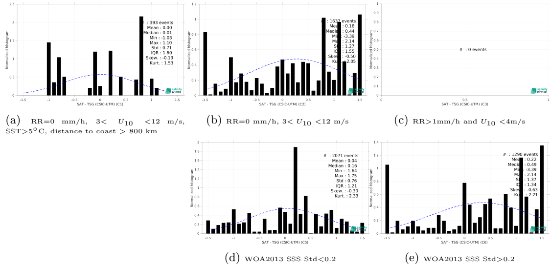
Figure 13: Normalized histogram of \Delta SSS (SMOS SSS L2Q v331 - With FLAG (CMEMS-CATDS-CPDC) - TSG (CSIC-UTM)) for 5 different subdatasets corresponding to: RR=0 mm/h, 3 < U_{10} < 12 m/s, SST>5°C, distance to coast > 800 km (a), RR=0 mm/h, 3 < U_{10} < 12 m/s (b), RR>1mm/h and U_{10} < 4 m/s (c), WOA2013 SSS Std<0.2 (d), WOA2013 SSS Std>0.2 (e).
