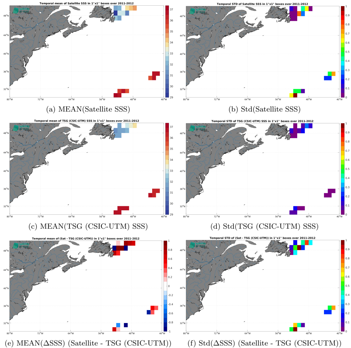
Figure 6: Temporal mean (left) and Std (right) of SSS from SMOS SSS L2Q v331 - With FLAG (CMEMS-CATDS-CPDC) (top), TSG (CSIC-UTM) (middle), and of \Delta SSS (Satellite - TSG (CSIC-UTM)). Only match-up pairs are used to generate these maps.
