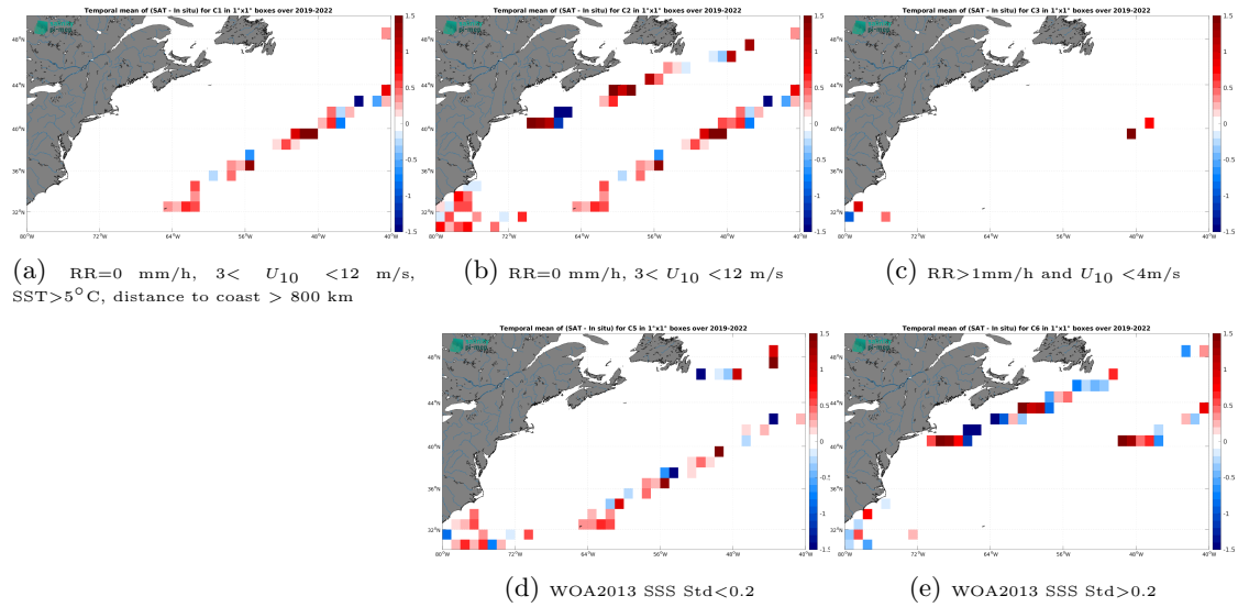
Figure 12: Temporal mean gridded over spatial boxes of size 1^\circ \times 1^\circ of \Delta\text{SSS} (SMOS SSS L2Q v331 - With FLAG (CMEMS-CATDS-CPDC) - Saildrone) for 5 different subdatasets corresponding to: \text{RR}=0 mm/h, 3 < U_{10} < 12 m/s, \text{SST} > 5^\circ\text{C} , distance to coast > 800 km (a), \text{RR}=0 mm/h, 3 < U_{10} < 12 m/s (b), \text{RR} > 1\text{mm/h} and U_{10} < 4\text{m/s} (c), WOA2013 SSS Std < 0.2 (d), WOA2013 SSS Std > 0.2 (e).
