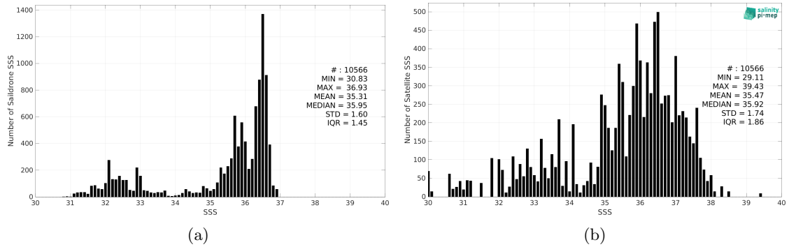
Figure 2: Histograms of SSS from Sairdrone (a) and SMOS SSS L2Q v331 - With FLAG (CMEMS-CATDS-CPDC) (b) considering all match-up pairs per bins of 0.1 over the Gulf Stream Pi-MEP region and for the full satellite product period.
