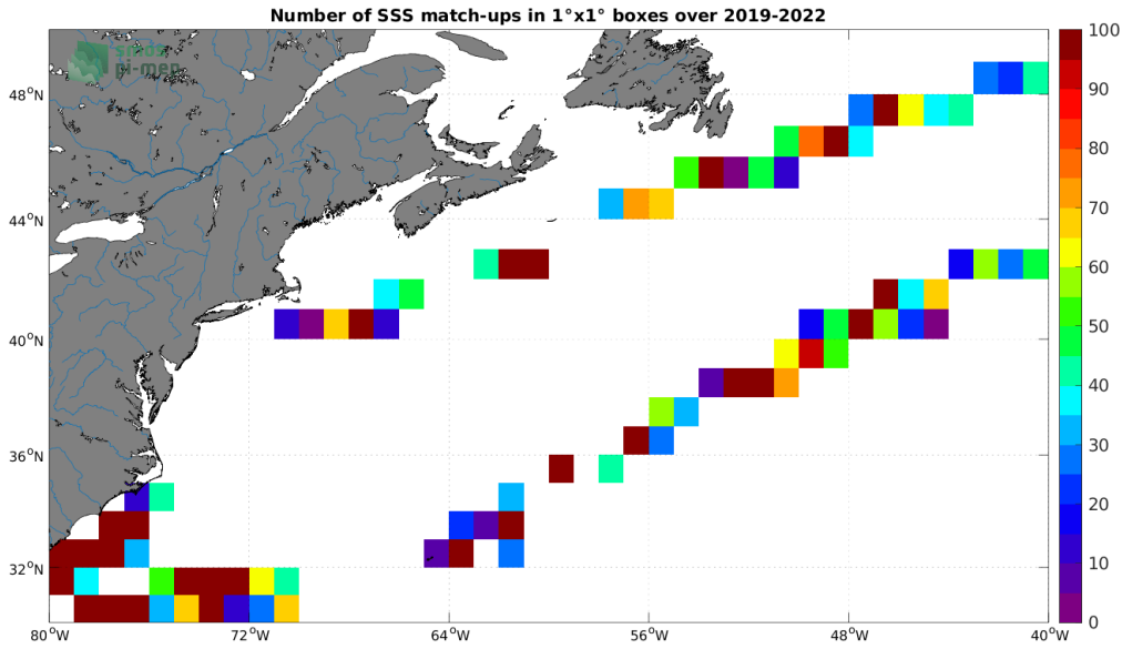
Figure 4: Number of SSS match-ups between Saildrone SSS and the SMOS SSS L2Q v331 - With FLAG (CMEMS-CATDS-CPDC) SSS product for the Gulf Stream Pi-MEP region over 1^\circ \times 1^\circ boxes and for the full satellite product period.
