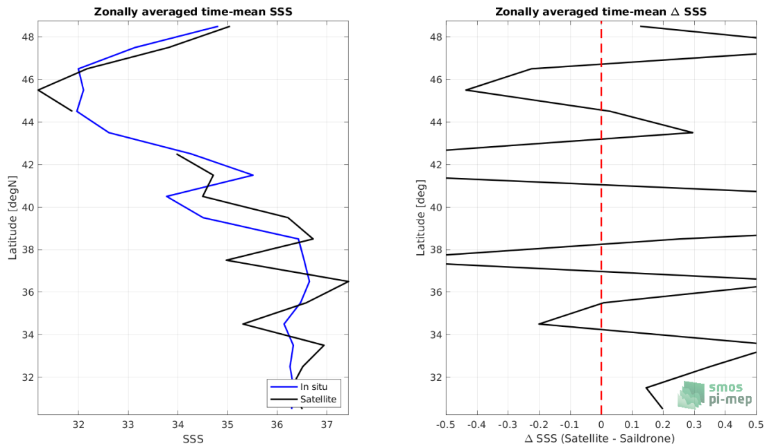
Figure 8: Left panel: Zonal mean SSS from SMOS SSS L2Q v331 - With FLAG (CMEMS-CATDS-CPDC) satellite product (black) and from Sairdron (blue). Right panel: Zonal mean of \Delta SSS (Satellite - Sairdron) for all the collected Pi-MEP match-up pairs estimated over the full satellite product period.
