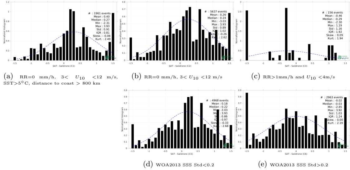
Figure 13: Normalized histogram of \Delta SSS (SMOS SSS L2Q v331 - With FLAG (CMEMS-CATDS-CPDC) - Sairdronne) for 5 different subdatasets corresponding to: RR=0 mm/h, 3 < U_{10} < 12 m/s, SST > 5°C, distance to coast > 800 km (a), RR=0 mm/h, 3 < U_{10} < 12 m/s (b), RR > 1mm/h and U_{10} < 4 m/s (c), WOA2013 SSS Std < 0.2 (d), WOA2013 SSS Std > 0.2 (e).
