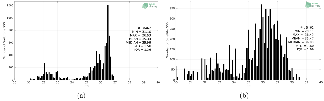
Figure 2: Histograms of SSS from Saildrone (a) and SMOS SSS L2Q v331 - With FLAG (CMEMS-CATDS-CPDC) (b) considering all match-up pairs per bins of 0.1 over the Gulf Stream Pi-MEP region and for the full satellite product period.
