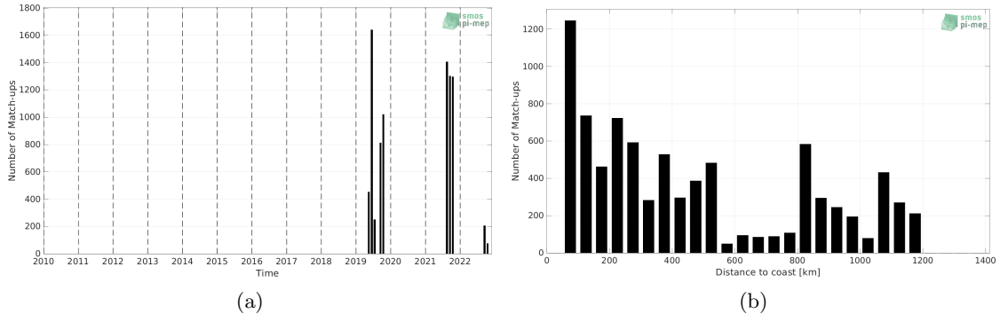
Figure 1: Number of match-ups between Saildrone and SMOS SSS L2Q v331 - With FLAG (CMEMS-CATDS-CPDC) SSS as a function of time (a) and as function of the distance to coast (b) over the Gulf Stream Pi-MEP region and for the full satellite product period.
