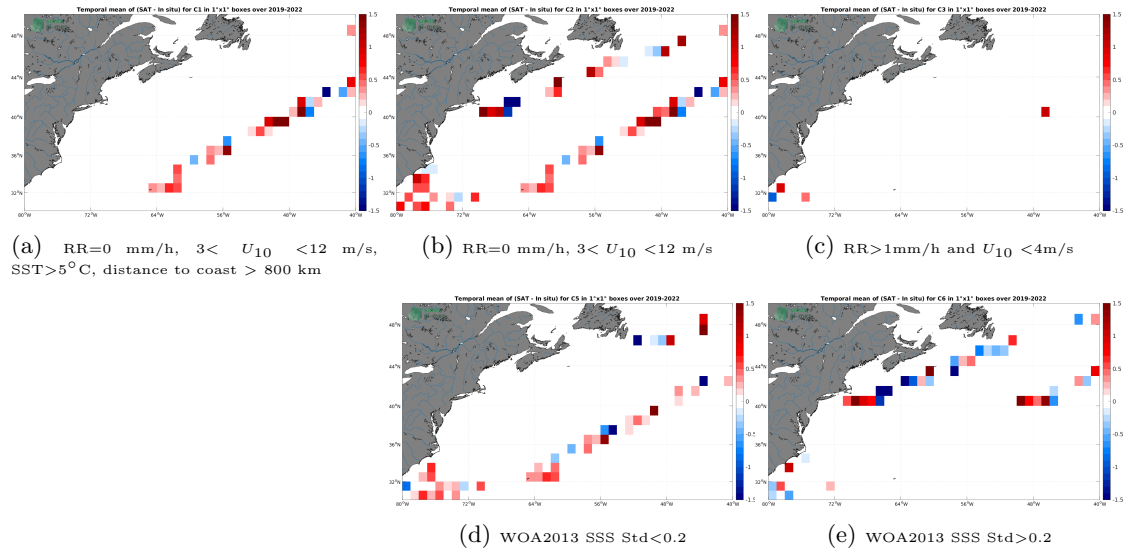
Figure 12: Temporal mean gridded over spatial boxes of size 1^\circ \times 1^\circ of \Delta SSS (SMOS SSS L2Q v331 - With FLAG (CMEMS-CATDS-CPDC) - Saildrone) for 5 different subdatasets corresponding to: RR=0 mm/h, 3 < U_{10} < 12 m/s, SST > 5^\circ C , distance to coast > 800 km (a), RR=0 mm/h, 3 < U_{10} < 12 m/s (b), RR > 1 mm/h and U_{10} < 4 m/s (c), WOA2013 SSS Std < 0.2 (d), WOA2013 SSS Std > 0.2 (e).
