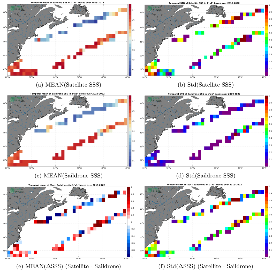
Figure 6: Temporal mean (left) and Std (right) of SSS from SMOS SSS L2Q v331 - With FLAG (CMEMS-CATDS-CPDC) (top), Saildrone (middle), and of \Delta SSS (Satellite - Saildrone). Only match-up pairs are used to generate these maps.
