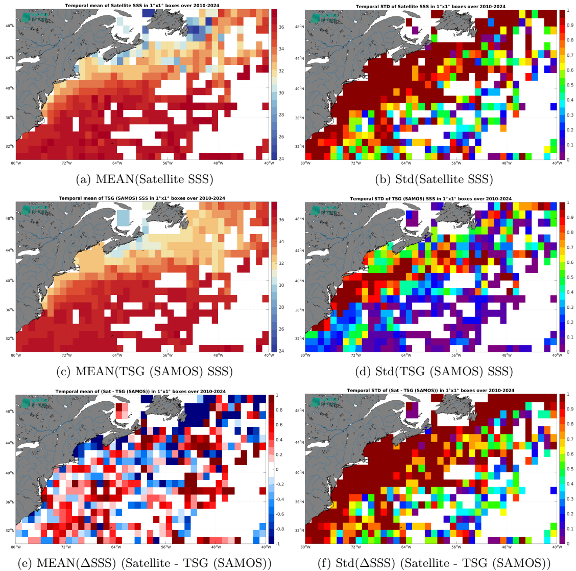
Figure 7: Temporal mean (left) and Std (right) of SSS from SMOS SSS L2Q v331 - No FLAG (CMEMS-CATDS-CPDC) (top), TSG (SAMOS) (middle), and of \Delta SSS (Satellite - TSG (SAMOS)). Only match-up pairs are used to generate these maps.
