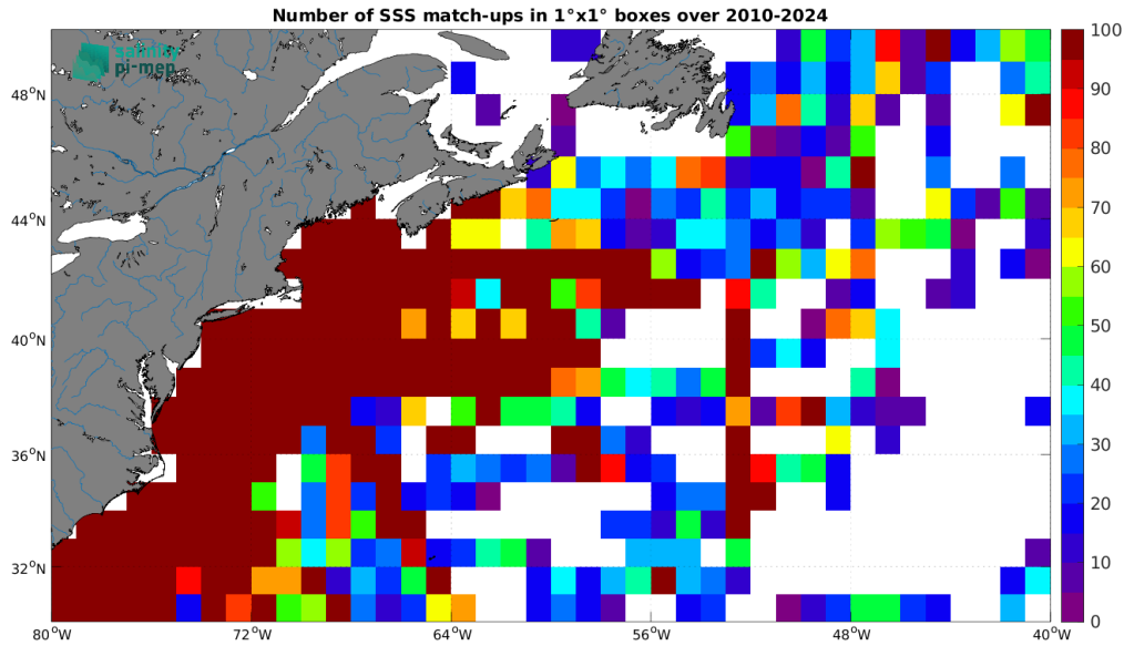
Figure 5: Number of SSS match-ups between TSG (SAMOS) SSS and the SMOS SSS L2Q v331 - No FLAG (CMEMS-CATDS-CPDC) SSS product for the Gulf Stream Pi-MEP region over 1^\circ \times 1^\circ boxes and for the full satellite product period.
