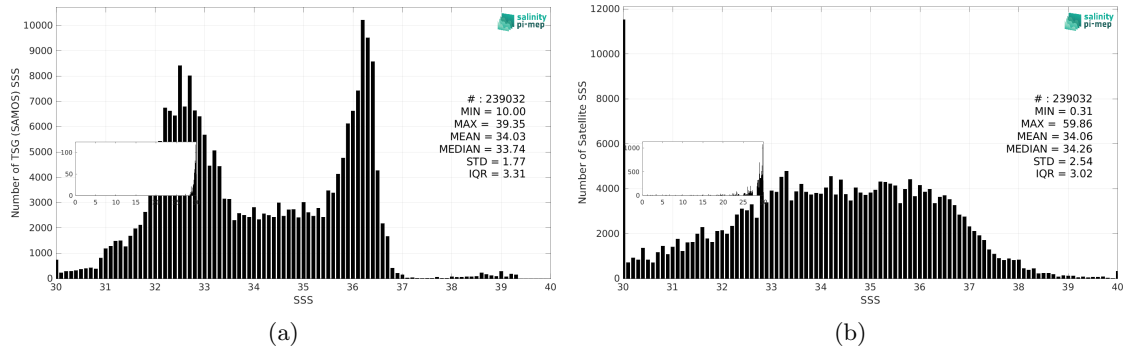
Figure 3: Histograms of SSS from TSG (SAMOS) (a) and SMOS SSS L2Q v331 - No FLAG (CMEMS-CATDS-CPDC) (b) considering all match-up pairs per bins of 0.1 over the Gulf Stream Pi-MEP region and for the full satellite product period.
