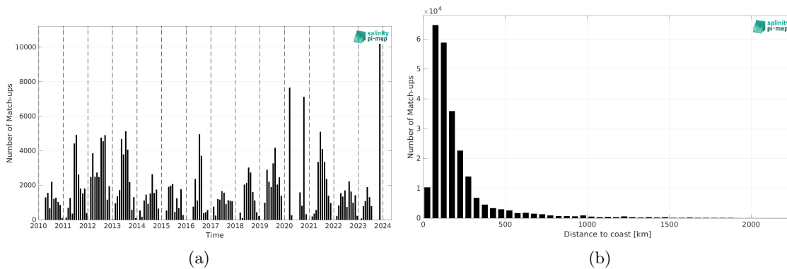
Figure 2: Number of match-ups between TSG (SAMOS) and SMOS SSS L2Q v331 - No FLAG (CMEMS-CATDS-CPDC) SSS as a function of time (a) and as function of the distance to coast (b) over the Gulf Stream Pi-MEP region and for the full satellite product period.
