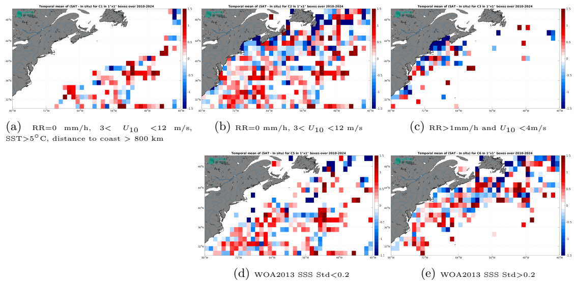
Figure 14: Temporal mean gridded over spatial boxes of size 1^\circ \times 1^\circ of \Delta SSS (SMOS SSS L2Q v331 - No FLAG (CMEMS-CATDS-CPDC) - TSG (SAMOS)) for 5 different subdatasets corresponding to: RR=0 mm/h, 3 < U_{10} < 12 m/s, SST > 5°C, distance to coast > 800 km (a), RR=0 mm/h, 3 < U_{10} < 12 m/s (b), RR > 1mm/h and U_{10} < 4 m/s (c), WOA2013 SSS Std < 0.2 (d), WOA2013 SSS Std > 0.2 (e).
