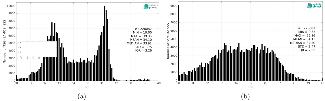
Figure 2: Histograms of SSS from TSG (SAMOS) (a) and SMOS SSS L2Q v331 - No FLAG (CMEMS-CATDS-CPDC) (b) considering all match-up pairs per bins of 0.1 over the Gulf Stream Pi-MEP region and for the full satellite product period.
