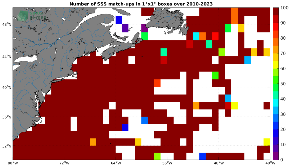
Figure 4: Number of SSS match-ups between TSG (SAMOS) SSS and the SMOS SSS L2Q v331 - No FLAG (CMEMS-CATDS-CPDC) SSS product for the Gulf Stream Pi-MEP region over 1^\circ \times 1^\circ boxes and for the full satellite product period.
