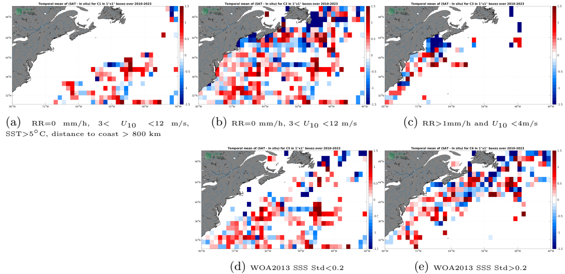
Figure 12: Temporal mean gridded over spatial boxes of size 1^{\circ}\times 1^{\circ} of \Delta\text{SSS} (SMOS SSS L2Q v331 - No FLAG (CMEMS-CATDS-CPDC) - TSG (SAMOS)) for 5 different subdatasets corresponding to:RR=0 mm/h, 3 < U_{10} < 12 m/s, SST >5^{\circ}\text{C} , distance to coast > 800 km (a), RR=0 mm/h, 3 < U_{10} < 12 m/s (b), RR >1 mm/h and U_{10} < 4 m/s (c), WOA2013 SSS Std <0.2 (d), WOA2013 SSS Std >0.2 (e).
