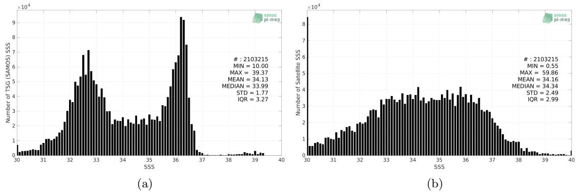
Figure 2: Histograms of SSS from TSG (SAMOS) (a) and SMOS SSS L2Q v331 - No FLAG (CMEMS-CATDS-CPDC) (b) considering all match-up pairs per bins of 0.1 over the Gulf Stream Pi-MEP region and for the full satellite product period.
