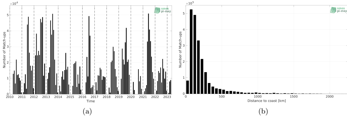
Figure 1: Number of match-ups between TSG (SAMOS) and SMOS SSS L2Q v331 - No FLAG (CMEMS-CATDS-CPDC) SSS as a function of time (a) and as function of the distance to coast (b) over the Gulf Stream Pi-MEP region and for the full satellite product period.
