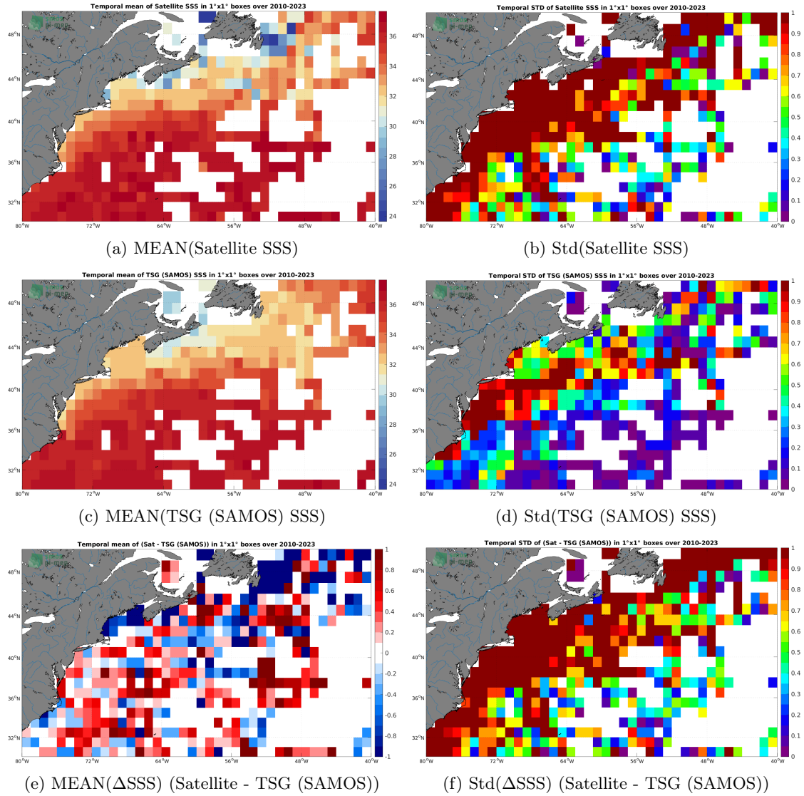
Figure 6: Temporal mean (left) and Std (right) of SSS from SMOS SSS L2Q v331 - No FLAG (CMEMS-CATDS-CPDC) (top), TSG (SAMOS) (middle), and of \Delta SSS (Satellite - TSG (SAMOS)). Only match-up pairs are used to generate these maps.
