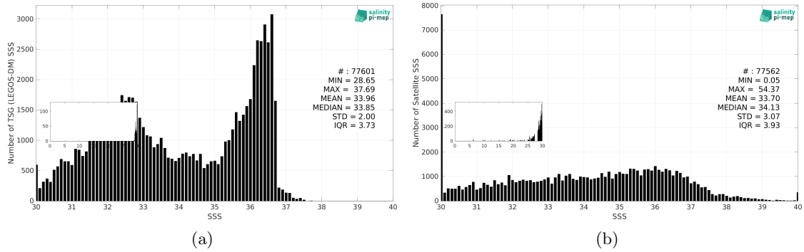
Figure 3: Histograms of SSS from TSG (LEGOS-DM) (a) and SMOS SSS L2Q v331 - No FLAG (CMEMS-CATDS-CPDC) (b) considering all match-up pairs per bins of 0.1 over the Gulf Stream Pi-MEP region and for the full satellite product period.
