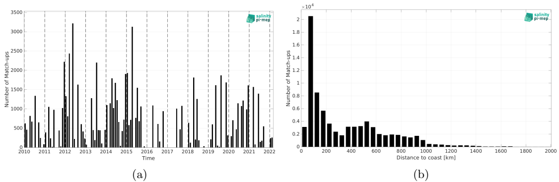
Figure 2: Number of match-ups between TSG (LEGOS-DM) and SMOS SSS L2Q v331 - No FLAG (CMEMS-CATDS-CPDC) SSS as a function of time (a) and as function of the distance to coast (b) over the Gulf Stream Pi-MEP region and for the full satellite product period.
