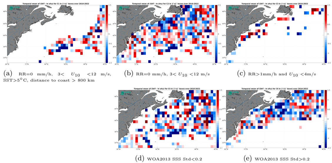
Figure 14: Temporal mean gridded over spatial boxes of size 1^\circ \times 1^\circ of \Delta SSS (SMOS SSS L2Q v331 - No FLAG (CMEMS-CATDS-CPDC) - TSG (LEGOS-DM)) for 5 different subdatasets corresponding to: RR=0 mm/h, 3 < U_{10} < 12 m/s, SST>5°C, distance to coast > 800 km (a), RR=0 mm/h, 3 < U_{10} < 12 m/s (b), RR>1mm/h and U_{10} < 4 m/s (c), WOA2013 SSS Std<0.2 (d), WOA2013 SSS Std>0.2 (e).
