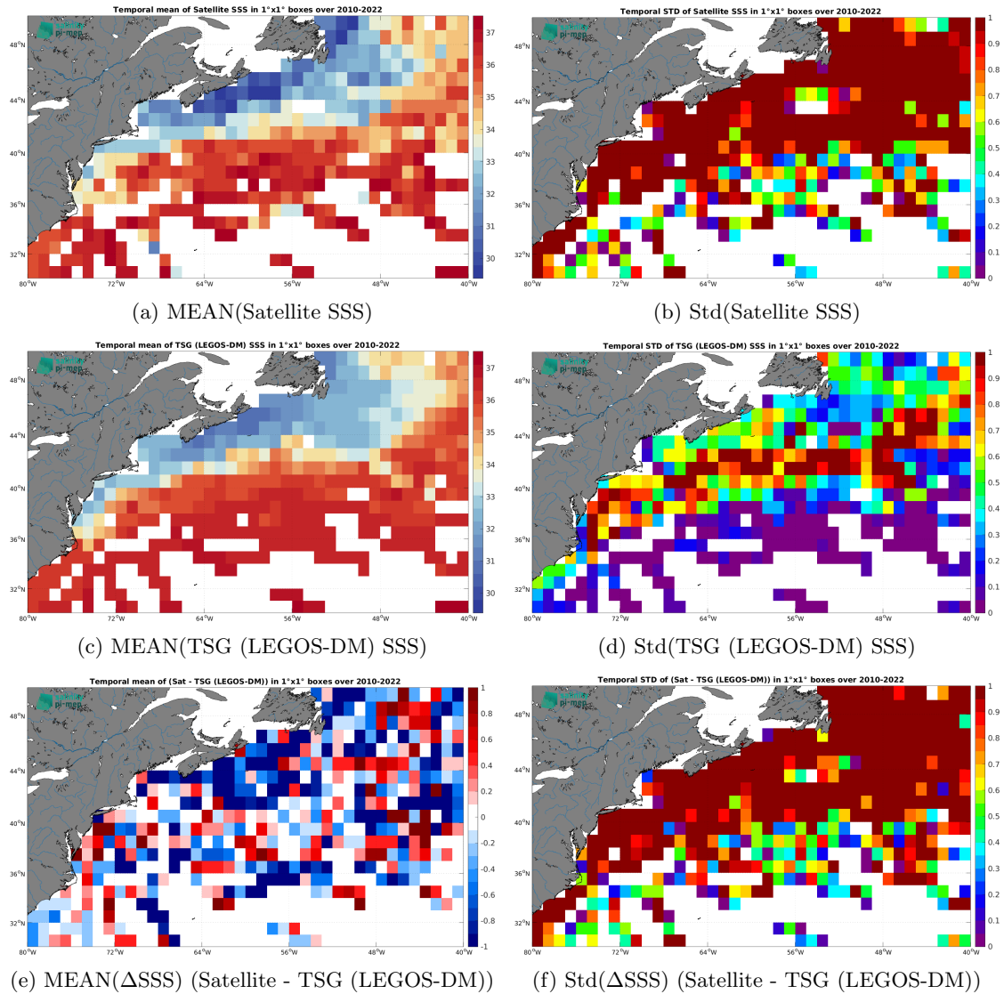
Figure 7: Temporal mean (left) and Std (right) of SSS from SMOS SSS L2Q v331 - No FLAG (CMEMS-CATDS-CPDC) (top), TSG (LEGOS-DM) (middle), and of \Delta SSS (Satellite - TSG (LEGOS-DM)). Only match-up pairs are used to generate these maps.
