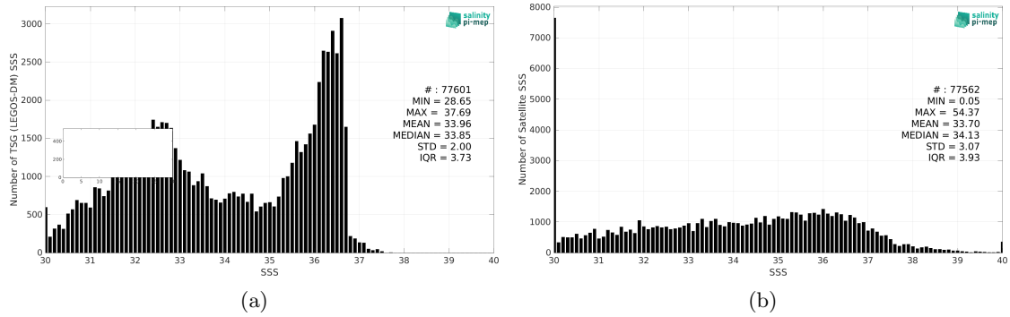
Figure 2: Histograms of SSS from TSG (LEGOS-DM) (a) and SMOS SSS L2Q v331 - No FLAG (CMEMS-CATDS-CPDC) (b) considering all match-up pairs per bins of 0.1 over the Gulf Stream Pi-MEP region and for the full satellite product period.
