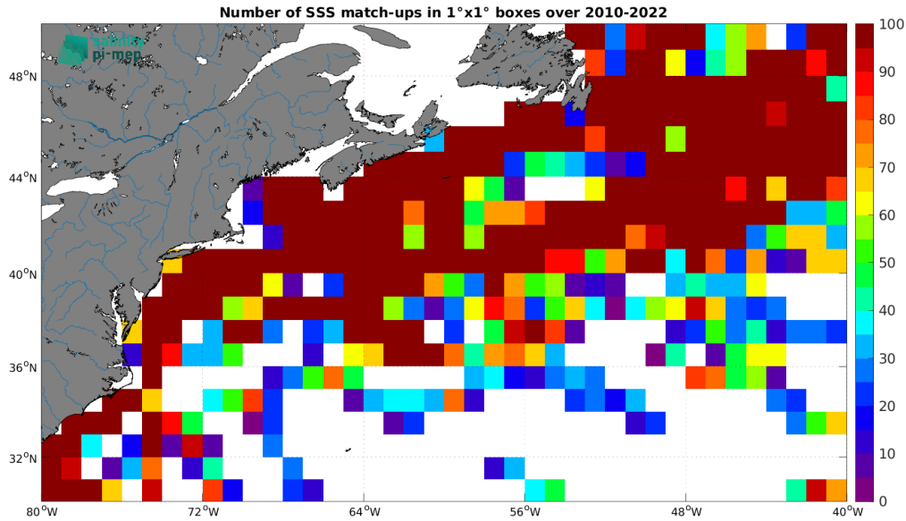
Figure 4: Number of SSS match-ups between TSG (LEGOS-DM) SSS and the SMOS SSS L2Q v331 - No FLAG (CMEMS-CATDS-CPDC) SSS product for the Gulf Stream Pi-MEP region over 1^\circ \times 1^\circ boxes and for the full satellite product period.
