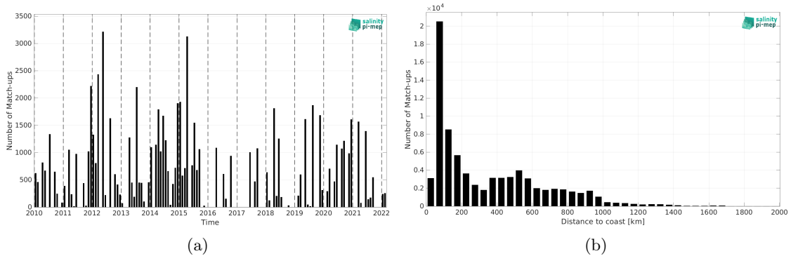
Figure 1: Number of match-ups between TSG (LEGOS-DM) and SMOS SSS L2Q v331 - No FLAG (CMEMS-CATDS-CPDC) SSS as a function of time (a) and as function of the distance to coast (b) over the Gulf Stream Pi-MEP region and for the full satellite product period.
