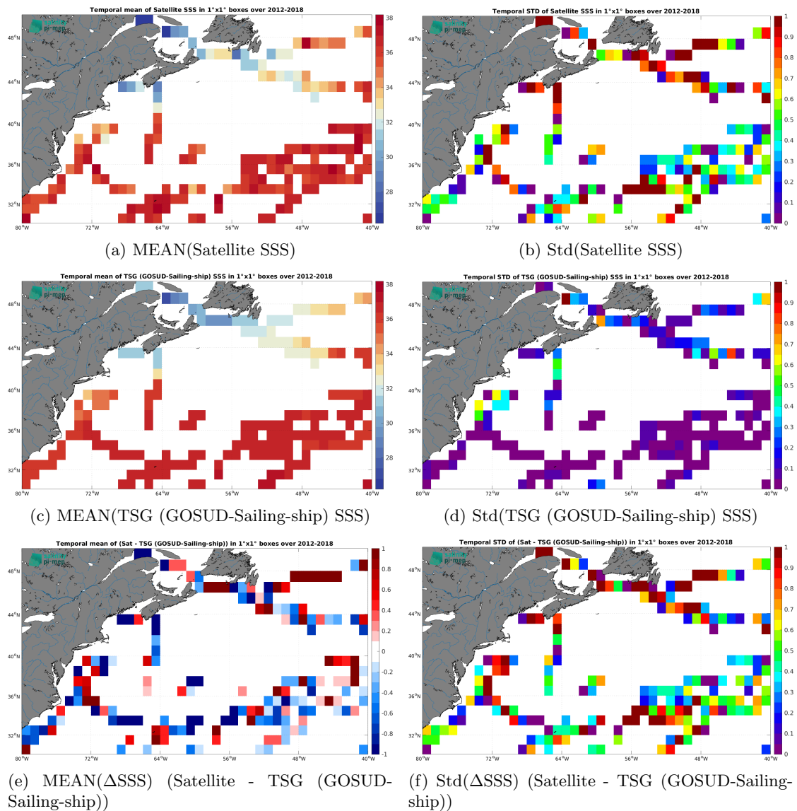
Figure 7: Temporal mean (left) and Std (right) of SSS from SMOS SSS L2Q v331 - No FLAG (CMEMS-CATDS-CPDC) (top), TSG (GOSUD-Sailing-ship) (middle), and of \Delta SSS (Satellite - TSG (GOSUD-Sailing-ship)). Only match-up pairs are used to generate these maps.
