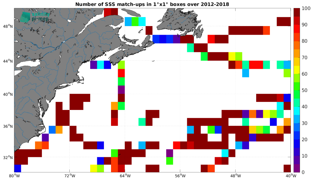
Figure 5: Number of SSS match-ups between TSG (GOSUD-Sailing-ship) SSS and the SMOS SSS L2Q v331 - No FLAG (CMEMS-CATDS-CPDC) SSS product for the Gulf Stream Pi-MEP region over 1^\circ \times 1^\circ boxes and for the full satellite product period.
