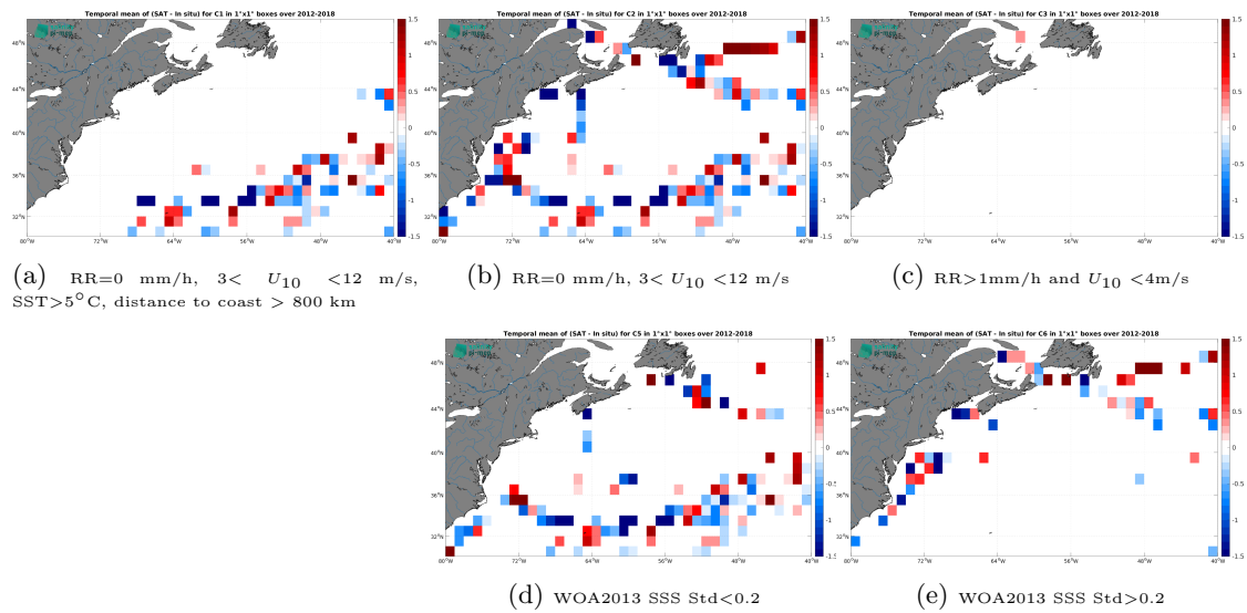
Figure 14: Temporal mean gridded over spatial boxes of size 1^\circ \times 1^\circ of \Delta SSS (SMOS SSS L2Q v331 - No FLAG (CMEMS-CATDS-CPDC) - TSG (GOSUD-Sailing-ship)) for 5 different sub-datasets corresponding to:RR=0 mm/h, 3 < U_{10} < 12 m/s, SST >5^\circ\text{C} , distance to coast > 800 km (a), RR=0 mm/h, 3 < U_{10} < 12 m/s (b), RR >1 mm/h and U_{10} < 4 m/s (c), WOA2013 SSS Std <0.2 (d), WOA2013 SSS Std >0.2 (e).
