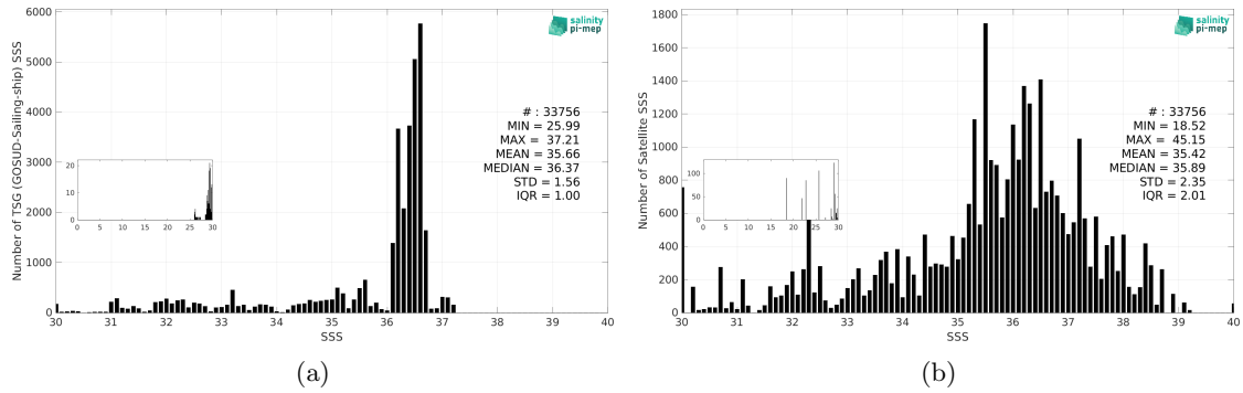
Figure 3: Histograms of SSS from TSG (GOSUD-Sailing-ship) (a) and SMOS SSS L2Q v331 - No FLAG (CMEMS-CATDS-CPDC) (b) considering all match-up pairs per bins of 0.1 over the Gulf Stream Pi-MEP region and for the full satellite product period.
