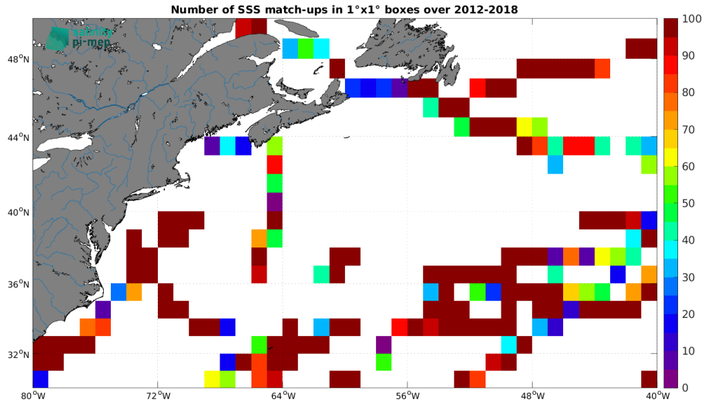
Figure 4: Number of SSS match-ups between TSG (GOSUD-Sailing-ship) SSS and the SMOS SSS L2Q v331 - No FLAG (CMEMS-CATDS-CPDC) SSS product for the Gulf Stream Pi-MEP region over 1^{\circ} \times 1^{\circ} boxes and for the full satellite product period.
