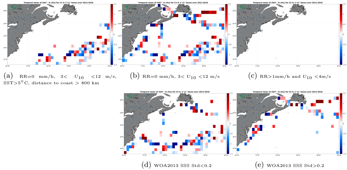
Figure 12: Temporal mean gridded over spatial boxes of size 1^{\circ}\times 1^{\circ} of \Delta SSS (SMOS SSS L2Q v331 - No FLAG (CMEMS-CATDS-CPDC) - TSG (GOSUD-Sailing-ship)) for 5 different sub-datasets corresponding to:RR=0 mm/h, 3 < U_{10} < 12 m/s, SST >5^{\circ}\text{C} , distance to coast > 800 km (a), RR=0 mm/h, 3 < U_{10} < 12 m/s (b), RR >1 mm/h and U_{10} < 4 m/s (c), WOA2013 SSS Std <0.2 (d), WOA2013 SSS Std >0.2 (e).
