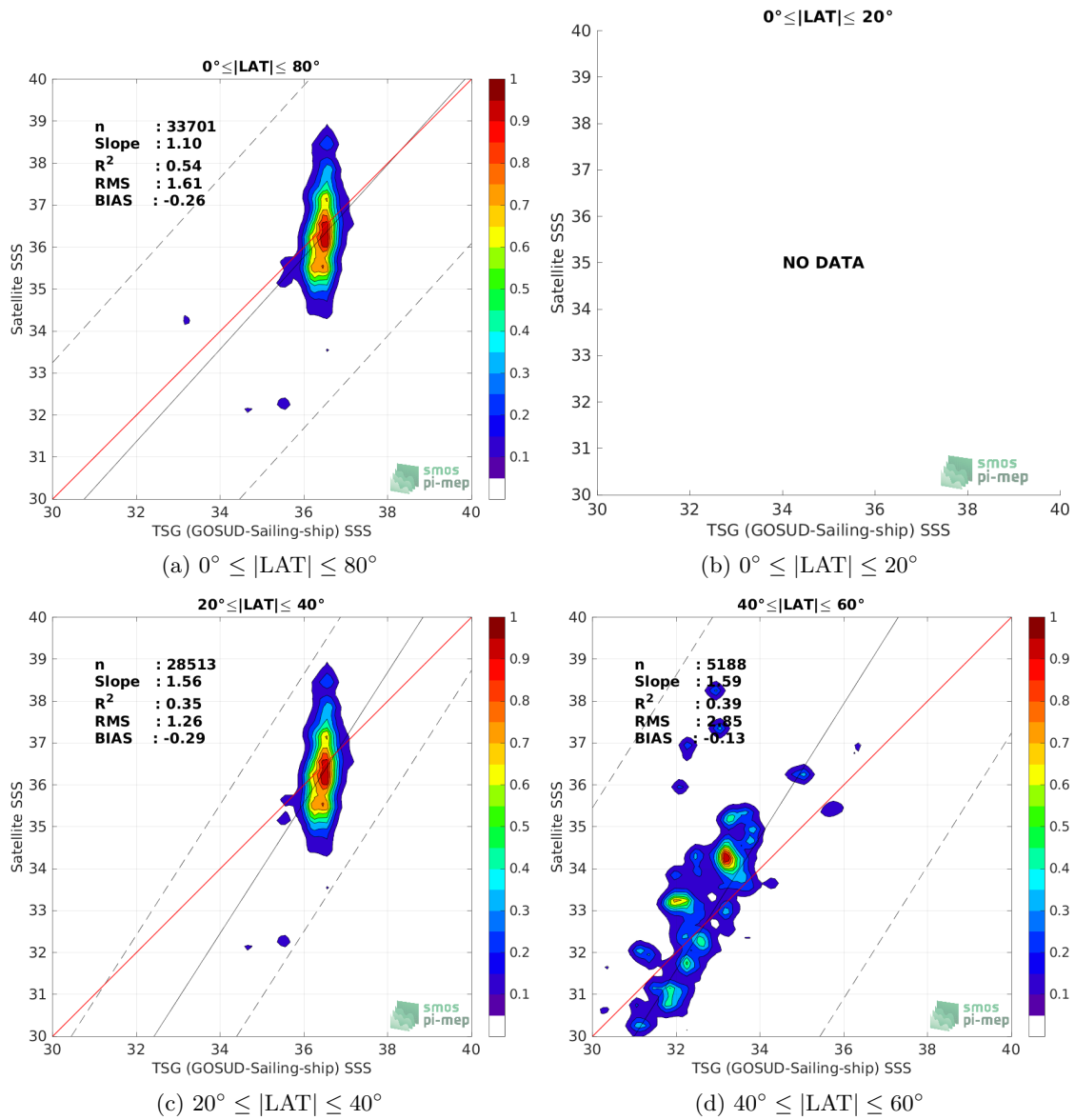
Figure 9: Contour maps of the concentration of SMOS SSS L2Q v331 - No FLAG (CMEMS-CATDS-CPDC) SSS (y-axis) versus TSG (GOSUD-Sailing-ship) SSS (x-axis) at match-up pairs for different latitude bands. For each plot, the red line shows x=y . The black thin and dashed lines indicate a linear fit through the data cloud and the \pm 95\% confidence levels, respectively. The number match-up pairs n , the slope and R^2 coefficient of the linear fit, the root mean square (RMS) and the mean bias between satellite and in situ data are indicated for each latitude band in each plots.
