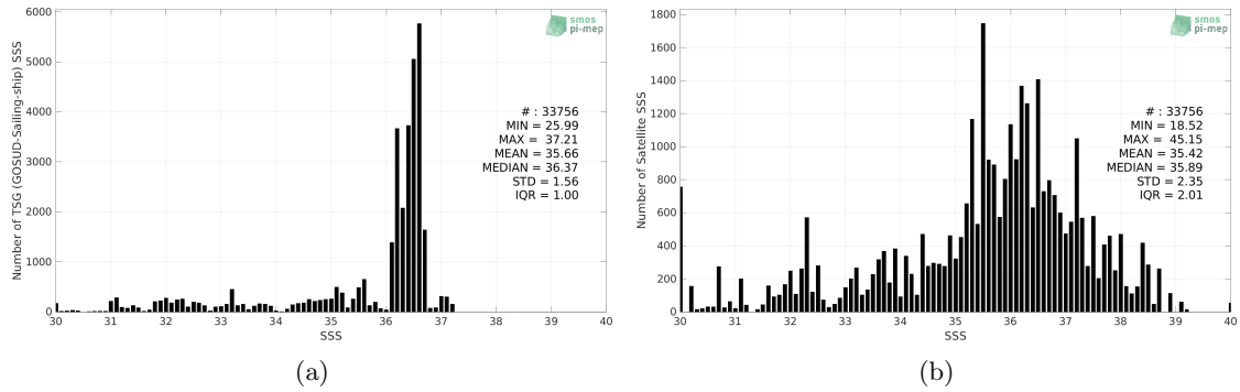
Figure 2: Histograms of SSS from TSG (GOSUD-Sailing-ship) (a) and SMOS SSS L2Q v331 - No FLAG (CMEMS-CATDS-CPDC) (b) considering all match-up pairs per bins of 0.1 over the Gulf Stream Pi-MEP region and for the full satellite product period.
