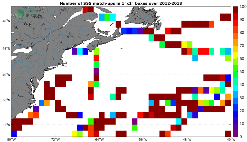
Figure 4: Number of SSS match-ups between TSG (GOSUD-Sailing-ship) SSS and the SMOS SSS L2Q v331 - No FLAG (CMEMS-CATDS-CPDC) SSS product for the Gulf Stream Pi-MEP region over 1^\circ \times 1^\circ boxes and for the full satellite product period.
