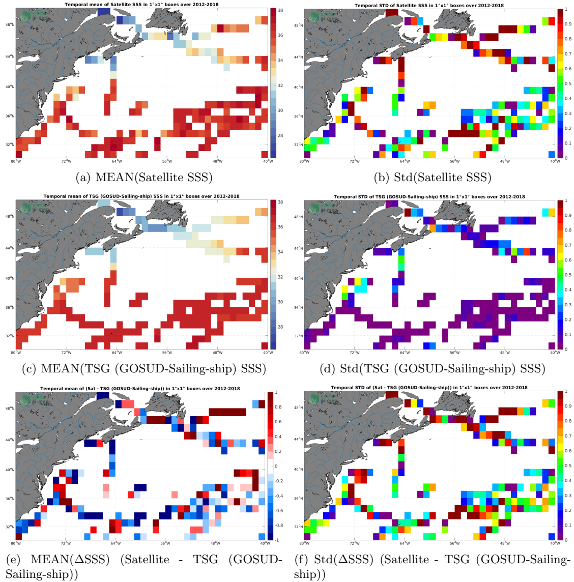
Figure 6: Temporal mean (left) and Std (right) of SSS from SMOS SSS L2Q v331 - No FLAG (CMEMS-CATDS-CPDC) (top), TSG (GOSUD-Sailing-ship) (middle), and of \Delta SSS (Satellite - TSG (GOSUD-Sailing-ship)). Only match-up pairs are used to generate these maps.
