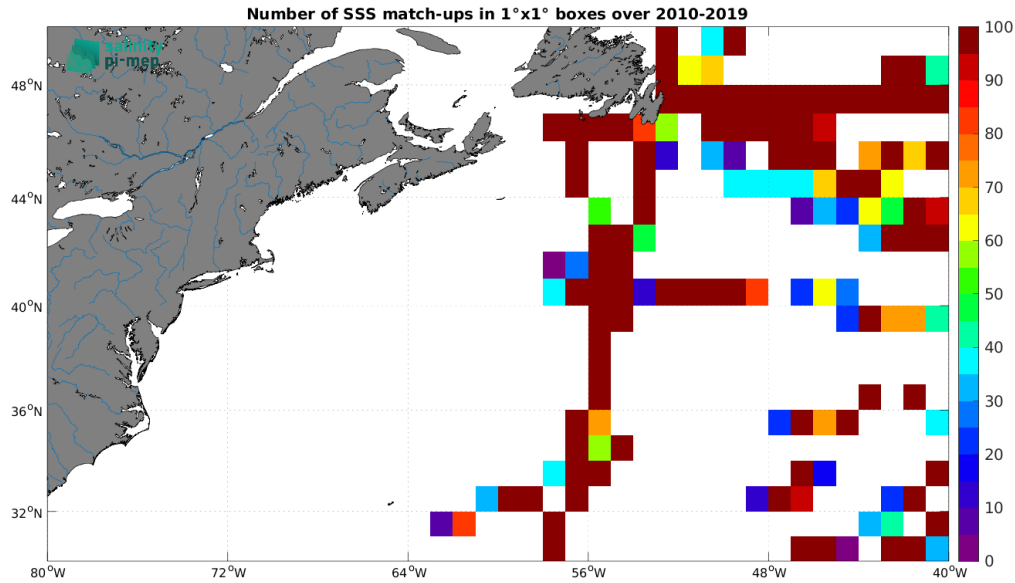
Figure 5: Number of SSS match-ups between TSG (GOSUD-Research-vessel) SSS and the SMOS SSS L2Q v331 - No FLAG (CMEMS-CATDS-CPDC) SSS product for the Gulf Stream Pi-MEP region over 1^\circ \times 1^\circ boxes and for the full satellite product period.
