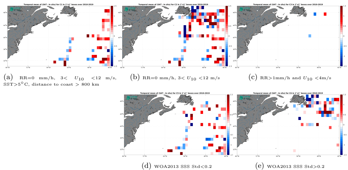
Figure 14: Temporal mean gridded over spatial boxes of size 1^\circ \times 1^\circ of \Delta SSS (SMOS SSS L2Q v331 - No FLAG (CMEMS-CATDS-CPDC) - TSG (GOSUD-Research-vessel)) for 5 different subdatasets corresponding to:RR=0 mm/h, 3 < U_{10} < 12 m/s, SST >5^\circ C, distance to coast > 800 km (a), RR=0 mm/h, 3 < U_{10} < 12 m/s (b), RR >1 mm/h and U_{10} < 4 m/s (c), WOA2013 SSS Std <0.2 (d), WOA2013 SSS Std >0.2 (e).
