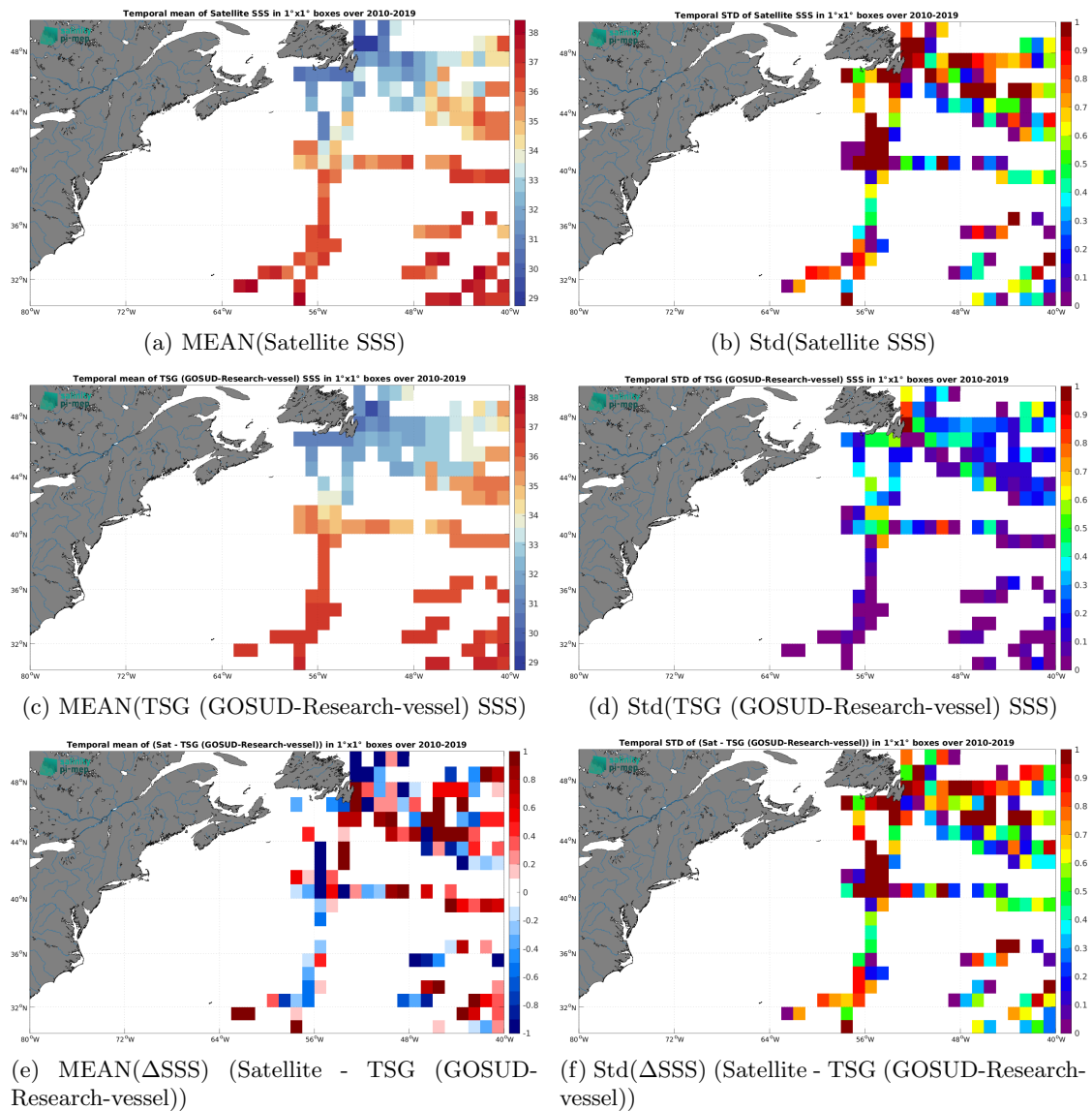
Figure 7: Temporal mean (left) and Std (right) of SSS from SMOS SSS L2Q v331 - No FLAG (CMEMS-CATDS-CPDC) (top), TSG (GOSUD-Research-vessel) (middle), and of \Delta SSS (Satellite - TSG (GOSUD-Research-vessel)). Only match-up pairs are used to generate these maps.
