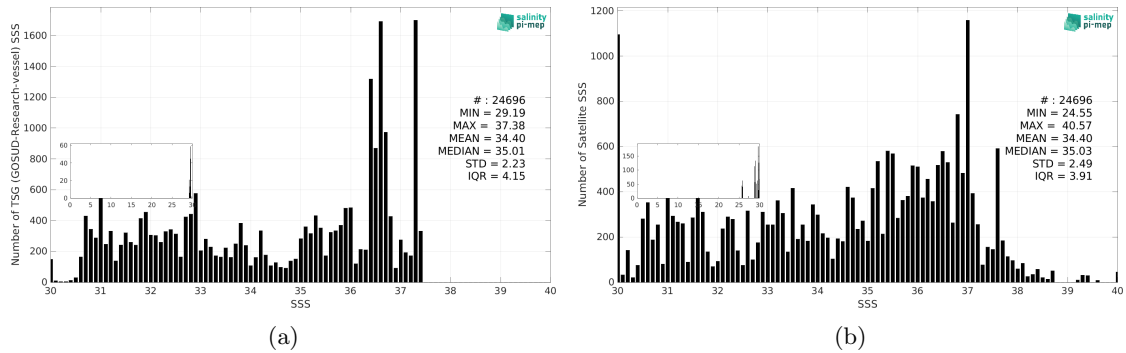
Figure 3: Histograms of SSS from TSG (GOSUD-Research-vessel) (a) and SMOS SSS L2Q v331 - No FLAG (CMEMS-CATDS-CPDC) (b) considering all match-up pairs per bins of 0.1 over the Gulf Stream Pi-MEP region and for the full satellite product period.
