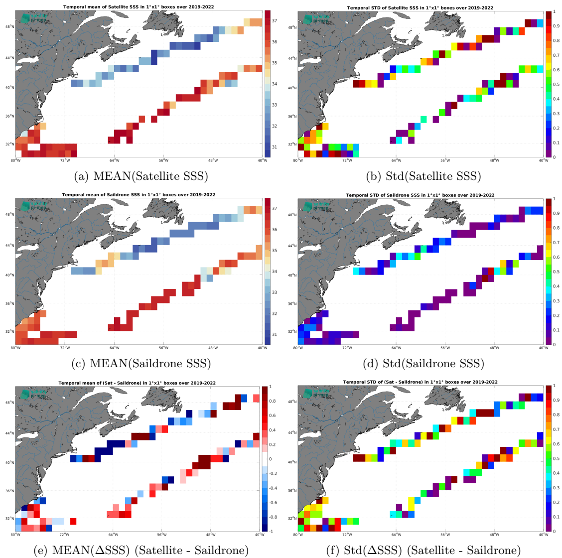
Figure 7: Temporal mean (left) and Std (right) of SSS from SMOS SSS L2Q v331 - No FLAG (CMEMS-CATDS-CPDC) (top), Saildrone (middle), and of \Delta SSS (Satellite - Saildrone). Only match-up pairs are used to generate these maps.
