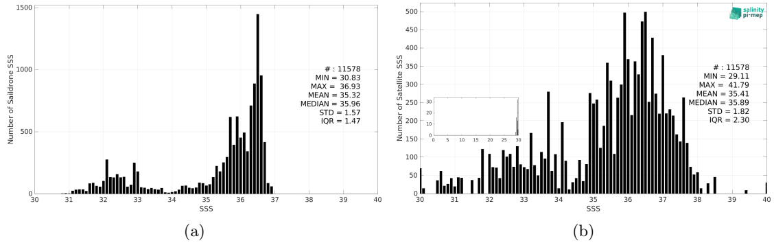
Figure 3: Histograms of SSS from Saildrone (a) and SMOS SSS L2Q v331 - No FLAG (CMEMS-CATDS-CPDC) (b) considering all match-up pairs per bins of 0.1 over the Gulf Stream Pi-MEP region and for the full satellite product period.
