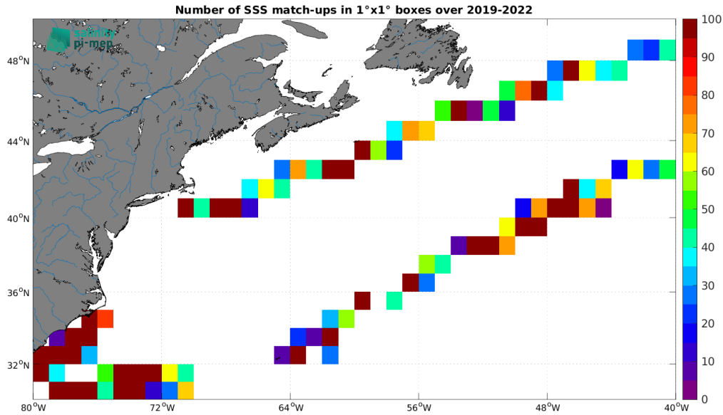
Figure 5: Number of SSS match-ups between Saildrone SSS and the SMOS SSS L2Q v331 - No FLAG (CMEMS-CATDS-CPDC) SSS product for the Gulf Stream Pi-MEP region over 1^\circ \times 1^\circ boxes and for the full satellite product period.
