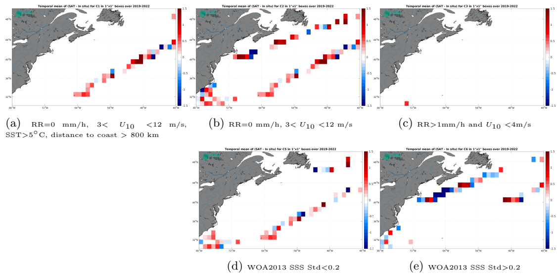
Figure 14: Temporal mean gridded over spatial boxes of size 1^\circ \times 1^\circ of \Delta SSS (SMOS SSS L2Q v331 - No FLAG (CMEMS-CATDS-CPDC) - Saildrone) for 5 different subdatasets corresponding to:RR=0 mm/h, 3 < U_{10} < 12 m/s, SST >5^\circ C, distance to coast > 800 km (a), RR=0 mm/h, 3 < U_{10} < 12 m/s (b), RR >1 mm/h and U_{10} < 4 m/s (c), WOA2013 SSS Std <0.2 (d), WOA2013 SSS Std >0.2 (e).
