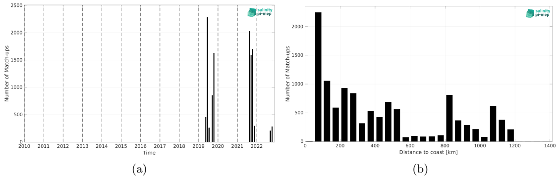
Figure 2: Number of match-ups between Saildrone and SMOS SSS L2Q v331 - No FLAG (CMEMS-CATDS-CPDC) SSS as a function of time (a) and as function of the distance to coast (b) over the Gulf Stream Pi-MEP region and for the full satellite product period.
