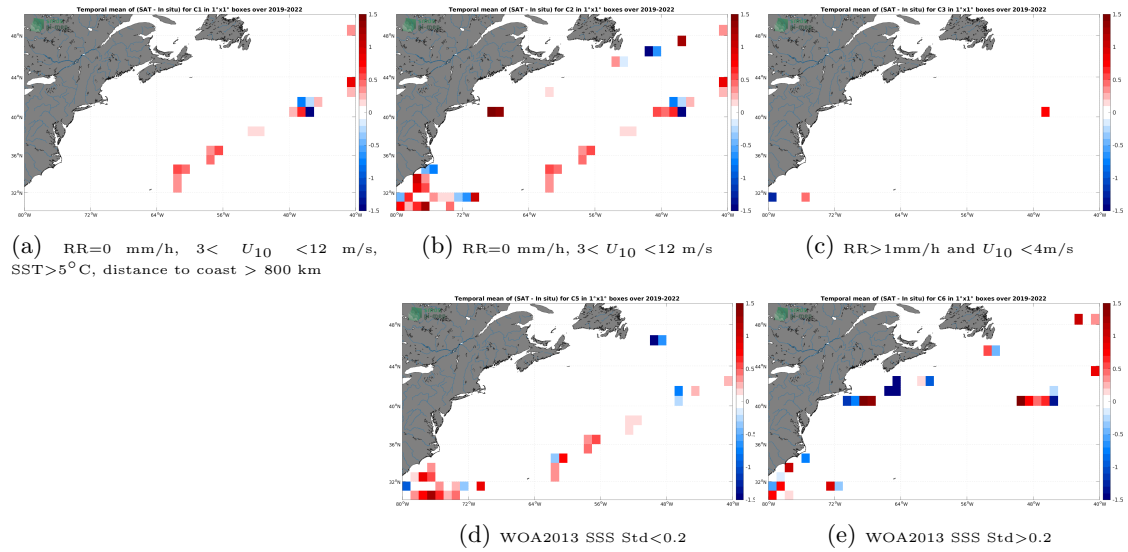
Figure 12: Temporal mean gridded over spatial boxes of size 1^\circ \times 1^\circ of \Delta SSS (SMOS SSS L2Q v331 - No FLAG (CMEMS-CATDS-CPDC) - Saildrone) for 5 different subdatasets corresponding to:RR=0 mm/h, 3 < U_{10} < 12 m/s, SST >5^\circ C, distance to coast > 800 km (a), RR=0 mm/h, 3 < U_{10} < 12 m/s (b), RR >1 mm/h and U_{10} < 4 m/s (c), WOA2013 SSS Std <0.2 (d), WOA2013 SSS Std >0.2 (e).
