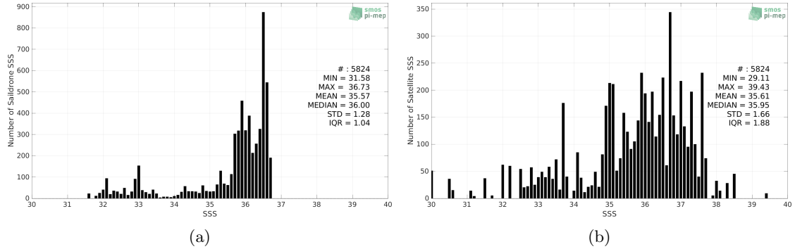
Figure 2: Histograms of SSS from Saifdrone (a) and SMOS SSS L2Q v331 - No FLAG (CMEMS-CATDS-CPDC) (b) considering all match-up pairs per bins of 0.1 over the Gulf Stream Pi-MEP region and for the full satellite product period.
