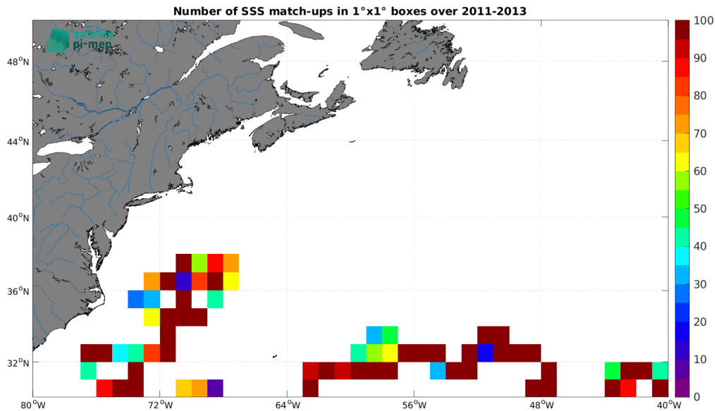
Figure 3: Number of SSS match-ups between Surface drifters SSS and the SMOS SSS L2Q v331 - No FLAG (CMEMS-CATDS-CPDC) SSS product for the Gulf Stream Pi-MEP region over 1^\circ \times 1^\circ boxes and for the full satellite product period.
