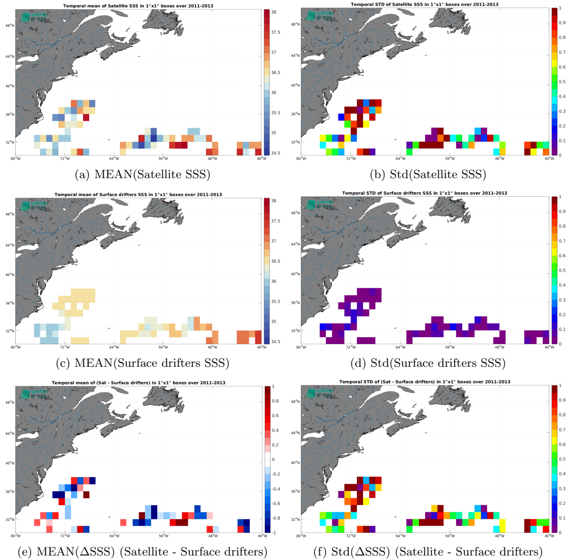
Figure 5: Temporal mean (left) and Std (right) of SSS from SMOS SSS L2Q v331 - No FLAG (CMEMS-CATDS-CPDC) (top), Surface drifters (middle), and of \Delta SSS (Satellite - Surface drifters). Only match-up pairs are used to generate these maps.
