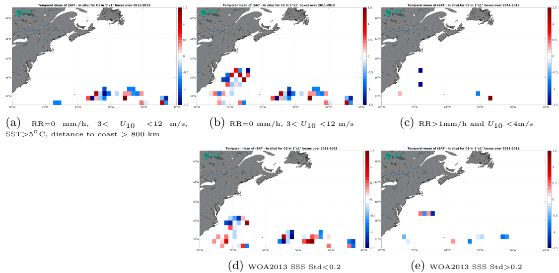
Figure 11: Temporal mean gridded over spatial boxes of size 1^{\circ}\times 1^{\circ} of \Delta\text{SSS} (SMOS SSS L2Q v331 - No FLAG (CMEMS-CATDS-CPDC) - Surface drifters) for 5 different subdatasets corresponding to:RR=0 mm/h, 3 < U_{10} < 12 m/s, SST >5^{\circ}\text{C} , distance to coast > 800 km (a), RR=0 mm/h, 3 < U_{10} < 12 m/s (b), RR >1 mm/h and U_{10} < 4 m/s (c), WOA2013 SSS Std <0.2 (d), WOA2013 SSS Std >0.2 (e).
