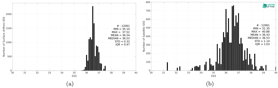
Figure 2: Histograms of SSS from Surface drifters (a) and SMOS SSS L2Q v331 - No FLAG (CMEMS-CATDS-CPDC) (b) considering all match-up pairs per bins of 0.1 over the Gulf Stream Pi-MEP region and for the full satellite product period.
