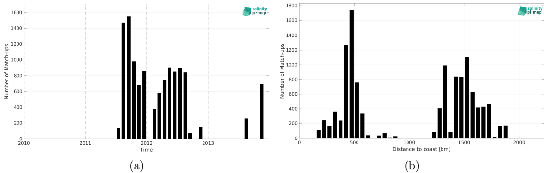
Figure 1: Number of match-ups between Surface drifters and SMOS SSS L2Q v331 - No FLAG (CMEMS-CATDS-CPDC) SSS as a function of time (a) and as function of the distance to coast (b) over the Gulf Stream Pi-MEP region and for the full satellite product period.
