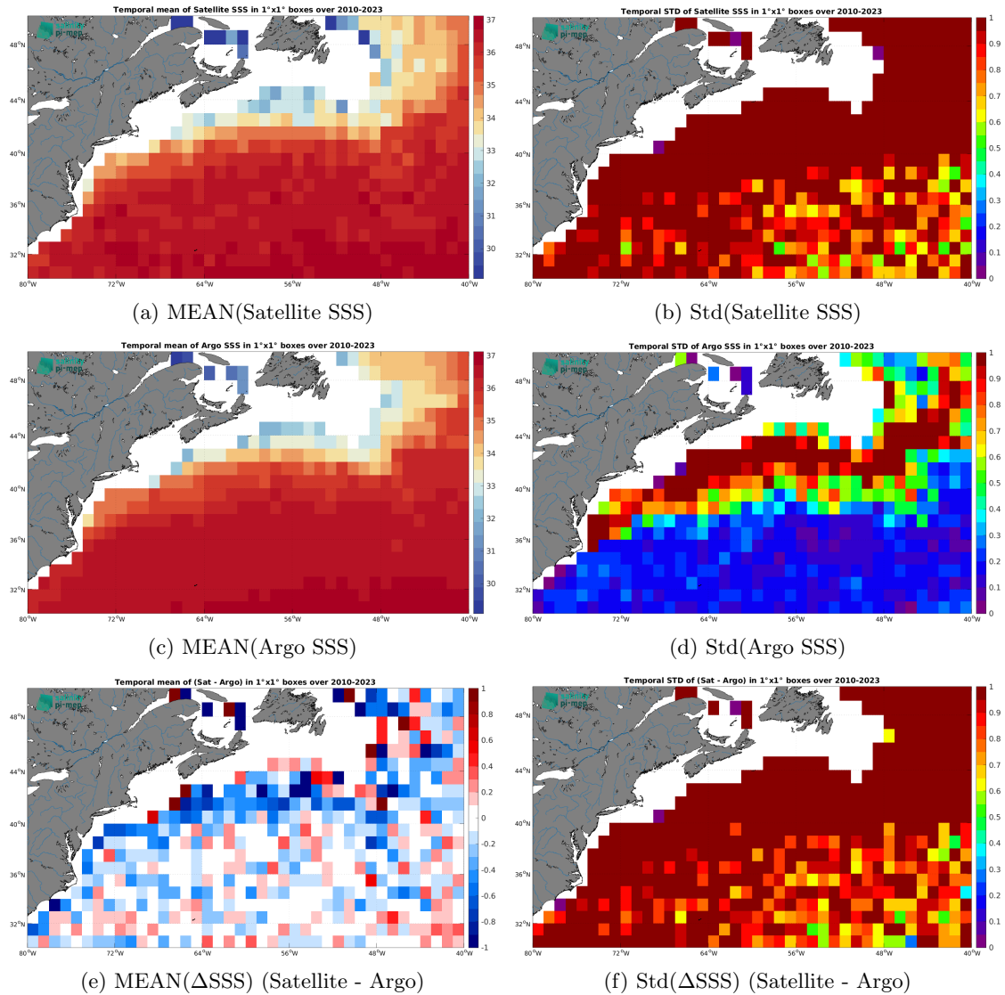
Figure 6: Temporal mean (left) and Std (right) of SSS from SMOS SSS L2Q v331 - No FLAG (CMEMS-CATDS-CPDC) (top), Argo (middle), and of \Delta SSS (Satellite - Argo). Only match-up pairs are used to generate these maps.
