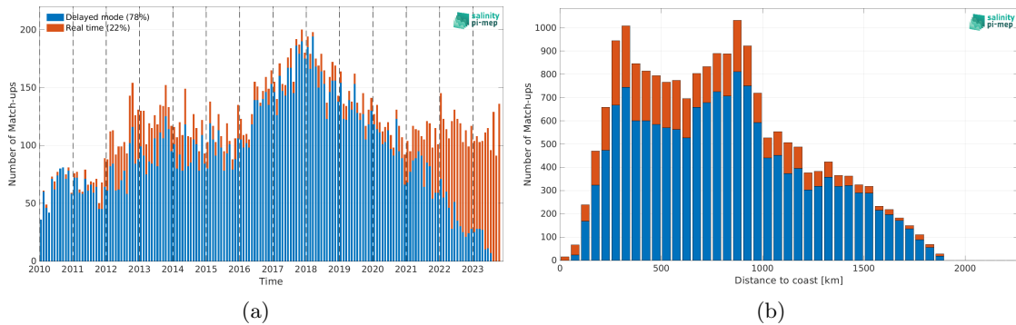
Figure 1: Number of match-ups between Argo and SMOS SSS L2Q v331 - No FLAG (CMEMS-CATDS-CPDC) SSS as a function of time (a) and as function of the distance to coast (b) over the Gulf Stream Pi-MEP region and for the full satellite product period.
