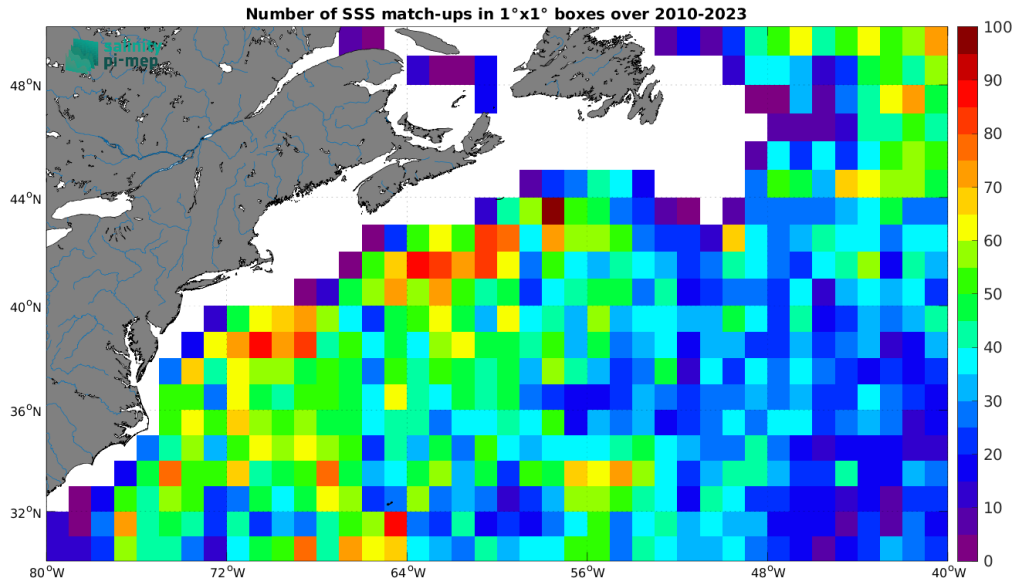
Figure 4: Number of SSS match-ups between Argo SSS and the SMOS SSS L2Q v331 - No FLAG (CMEMS-CATDS-CPDC) SSS product for the Gulf Stream Pi-MEP region over 1^\circ \times 1^\circ boxes and for the full satellite product period.
