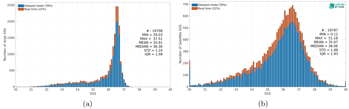
Figure 2: Histograms of SSS from Argo (a) and SMOS SSS L2Q v331 - No FLAG (CMEMS-CATDS-CPDC) (b) considering all match-up pairs per bins of 0.1 over the Gulf Stream Pi-MEP region and for the full satellite product period.
