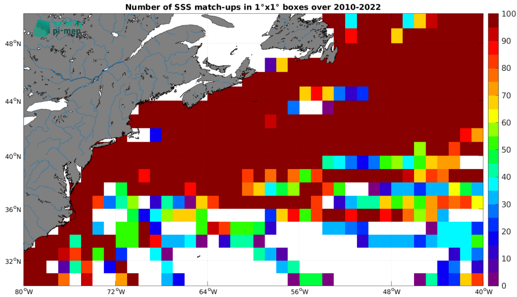
Figure 5: Number of SSS match-ups between TSG (LEGOS-DM) SSS and the SMOS SSS L3 v9 - 9 Days (CATDS-CEC-LOCEAN) SSS product for the Gulf Stream Pi-MEP region over 1^\circ \times 1^\circ boxes and for the full satellite product period.
