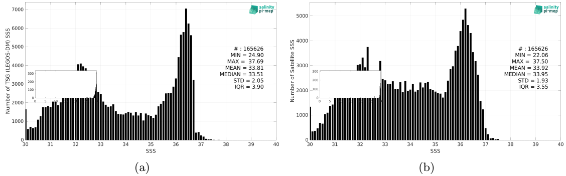
Figure 3: Histograms of SSS from TSG (LEGOS-DM) (a) and SMOS SSS L3 v9 - 9 Days (CATDS-CEC-LOCEAN) (b) considering all match-up pairs per bins of 0.1 over the Gulf Stream Pi-MEP region and for the full satellite product period.
