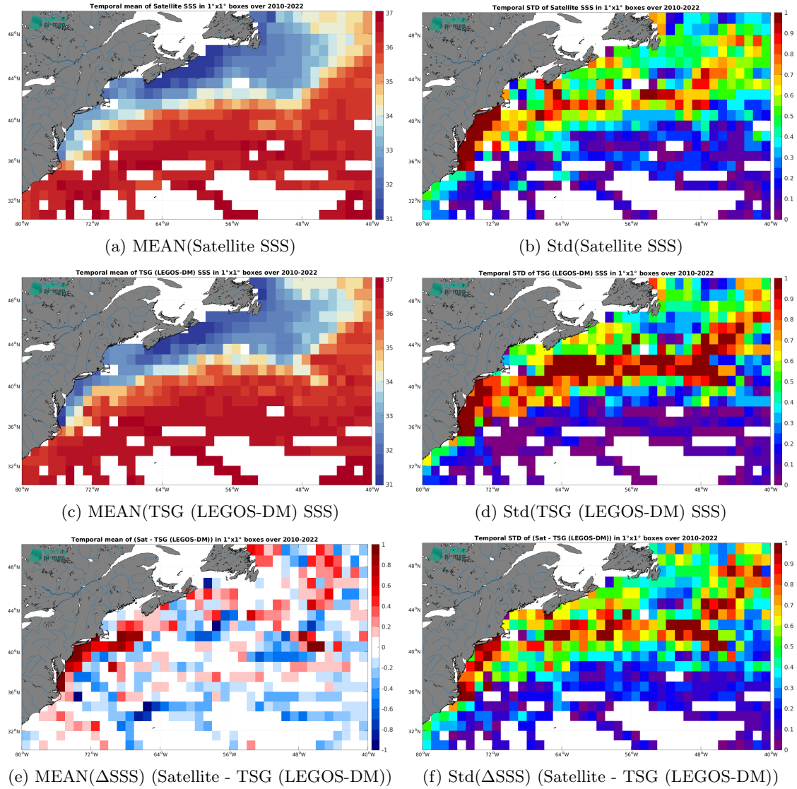
Figure 7: Temporal mean (left) and Std (right) of SSS from SMOS SSS L3 v9 - 9 Days (CATDS-CEC-LOCEAN) (top), TSG (LEGOS-DM) (middle), and of \Delta SSS (Satellite - TSG (LEGOS-DM)). Only match-up pairs are used to generate these maps.
