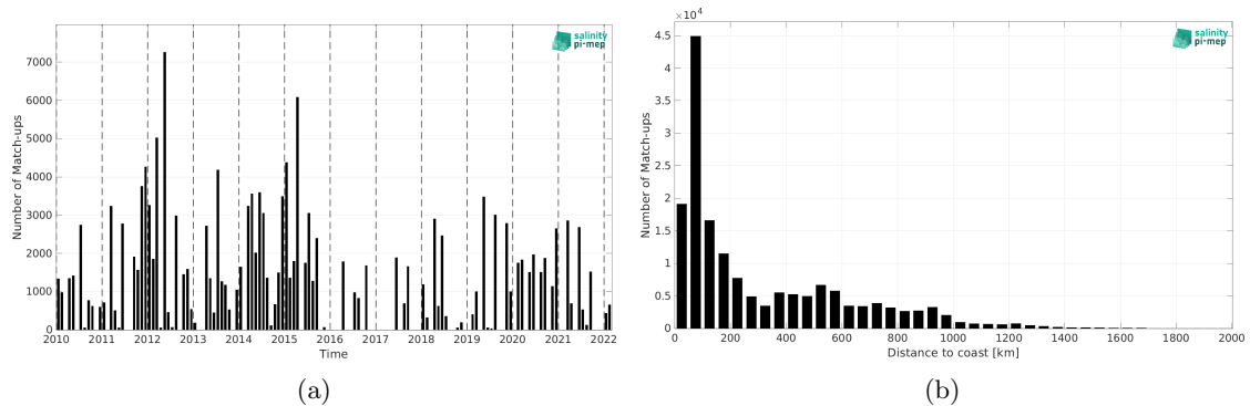
Figure 2: Number of match-ups between TSG (LEGOS-DM) and SMOS SSS L3 v9 - 9 Days (CATDS-CEC-LOCEAN) SSS as a function of time (a) and as function of the distance to coast (b) over the Gulf Stream Pi-MEP region and for the full satellite product period.
