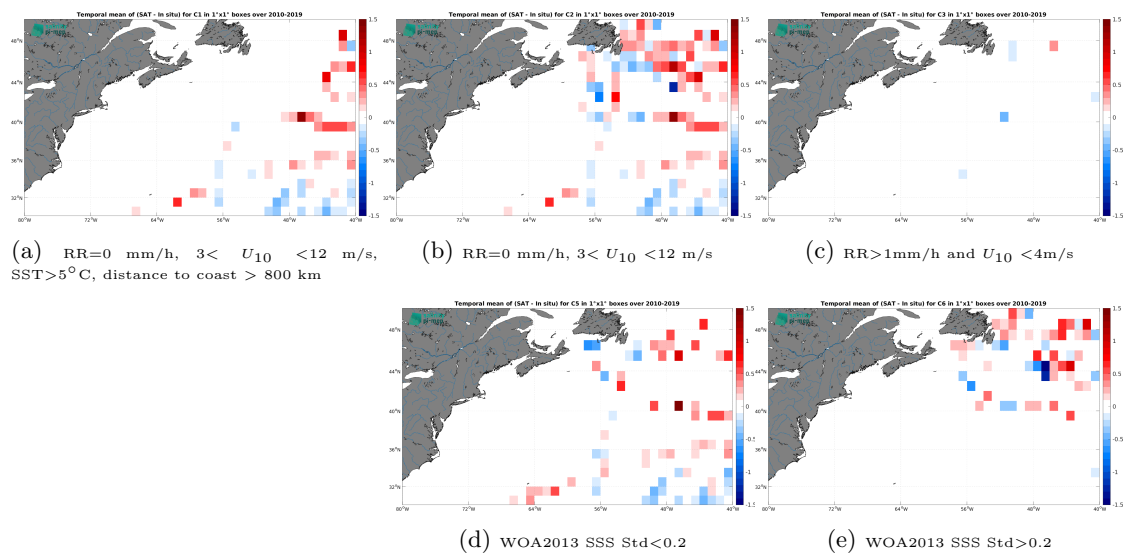
Figure 14: Temporal mean gridded over spatial boxes of size 1^\circ \times 1^\circ of \Delta SSS (SMOS SSS L3 v9 - 9 Days (CATDS-CEC-LOCEAN) - TSG (GOSUD-Research-vessel)) for 5 different subdatasets corresponding to:RR=0 mm/h, 3 < U_{10} < 12 m/s, SST>5°C, distance to coast > 800 km (a), RR=0 mm/h, 3 < U_{10} < 12 m/s (b), RR>1mm/h and U_{10} < 4 m/s (c), WOA2013 SSS Std<0.2 (d), WOA2013 SSS Std>0.2 (e).
