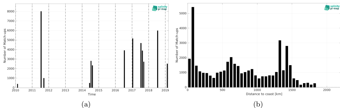
Figure 2: Number of match-ups between TSG (GOSUD-Research-vessel) and SMOS SSS L3 v9 - 9 Days (CATDS-CEC-LOCEAN) SSS as a function of time (a) and as function of the distance to coast (b) over the Gulf Stream Pi-MEP region and for the full satellite product period.
