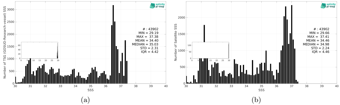
Figure 3: Histograms of SSS from TSG (GOSUD-Research-vessel) (a) and SMOS SSS L3 v9 - 9 Days (CATDS-CEC-LOCEAN) (b) considering all match-up pairs per bins of 0.1 over the Gulf Stream Pi-MEP region and for the full satellite product period.
