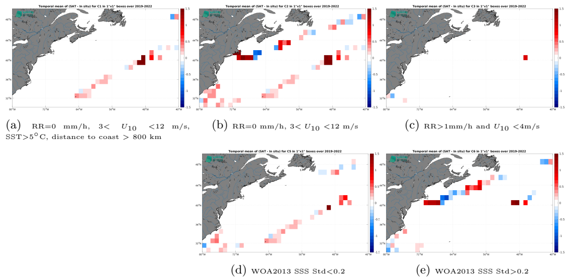
Figure 14: Temporal mean gridded over spatial boxes of size 1^\circ \times 1^\circ of \Delta SSS (SMOS SSS L3 v9 - 9 Days (CATDS-CEC-LOCEAN) - Sailability) for 5 different subdatasets corresponding to: RR=0 mm/h, 3 < U_{10} < 12 m/s, SST > 5°C, distance to coast > 800 km (a), RR=0 mm/h, 3 < U_{10} < 12 m/s (b), RR > 1mm/h and U_{10} < 4 m/s (c), WOA2013 SSS Std < 0.2 (d), WOA2013 SSS Std > 0.2 (e).
