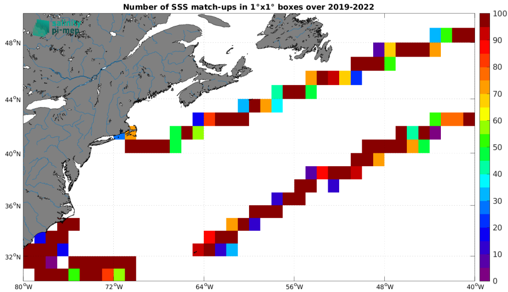
Figure 5: Number of SSS match-ups between Saildrone SSS and the SMOS SSS L3 v9 - 9 Days (CATDS-CEC-LOCEAN) SSS product for the Gulf Stream Pi-MEP region over 1^{\circ} \times 1^{\circ} boxes and for the full satellite product period.
