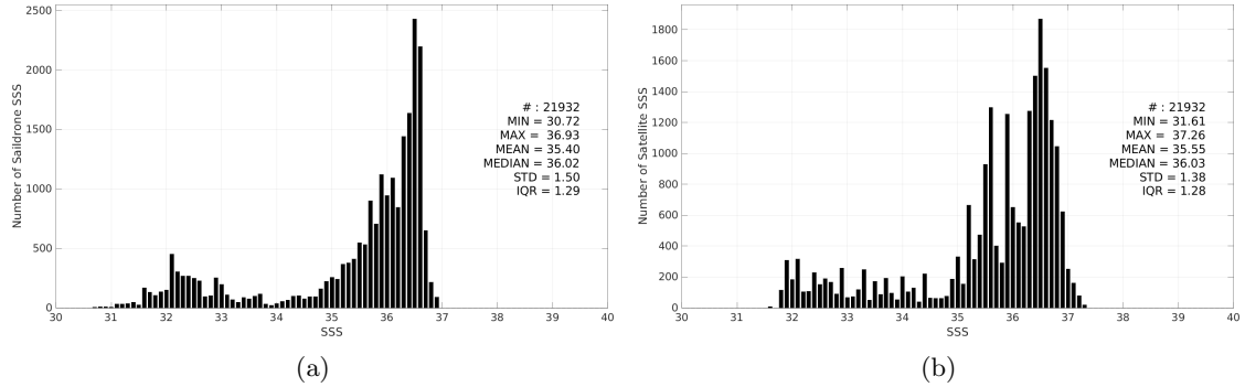
Figure 3: Histograms of SSS from Sairdrone (a) and SMOS SSS L3 v9 - 9 Days (CATDS-CEC-LOCEAN) (b) considering all match-up pairs per bins of 0.1 over the Gulf Stream Pi-MEP region and for the full satellite product period.
