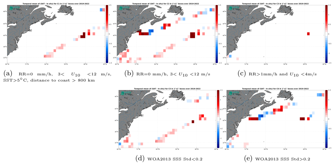
Figure 14: Temporal mean gridded over spatial boxes of size 1^\circ \times 1^\circ of \Delta SSS (SMOS SSS L3 v9 - 9 Days (CATDS-CEC-LOCEAN) - Saildrone) for 5 different subdatasets corresponding to:RR=0 mm/h, 3 < U_{10} < 12 m/s, SST>5°C, distance to coast > 800 km (a), RR=0 mm/h, 3 < U_{10} < 12 m/s (b), RR>1mm/h and U_{10} < 4 m/s (c), WOA2013 SSS Std<0.2 (d), WOA2013 SSS Std>0.2 (e).
