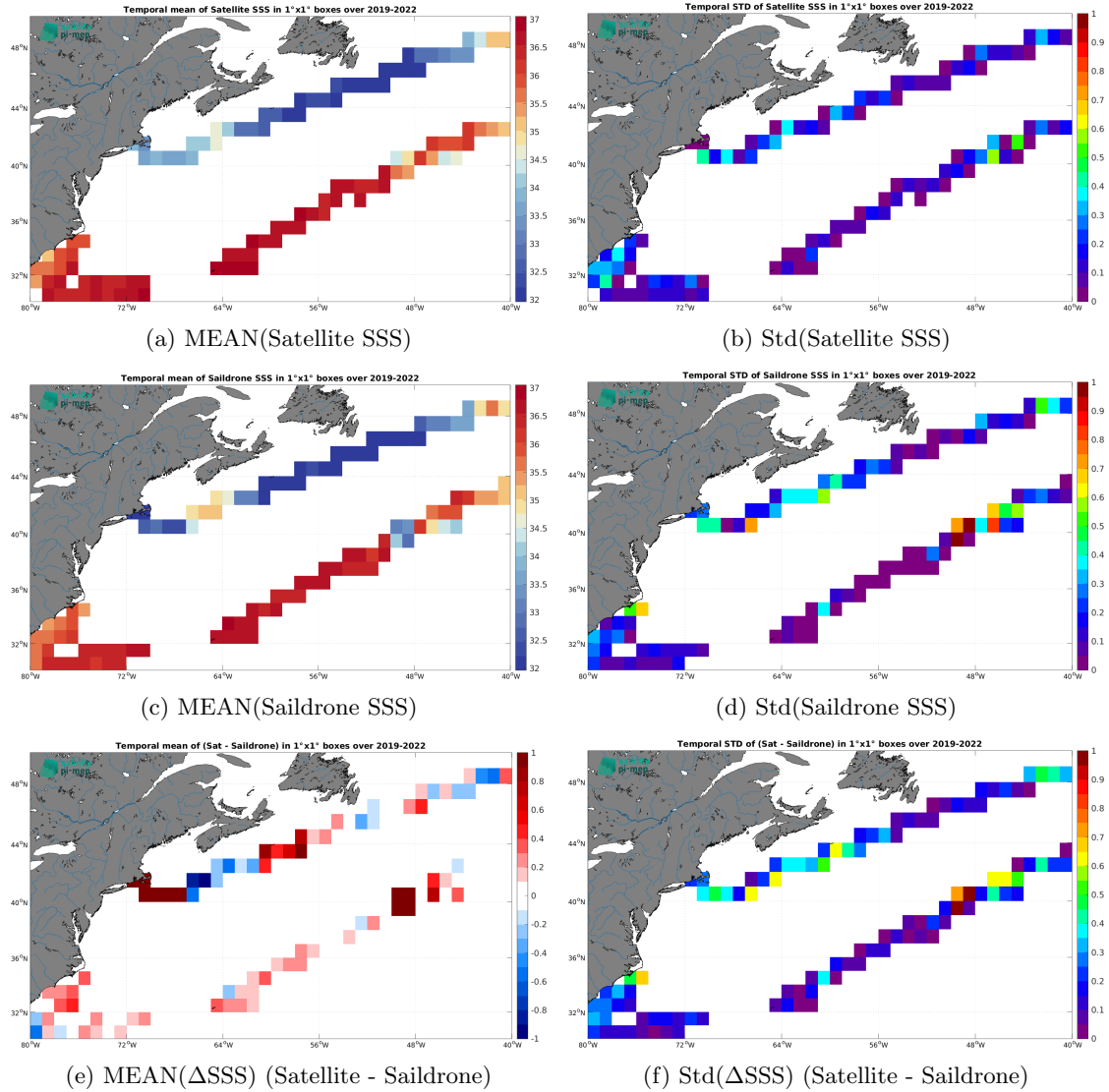
Figure 7: Temporal mean (left) and Std (right) of SSS from SMOS SSS L3 v9 - 9 Days (CATDS-CEC-LOCEAN) (top), Saildrone (middle), and of \Delta SSS (Satellite - Saildrone). Only match-up pairs are used to generate these maps.
