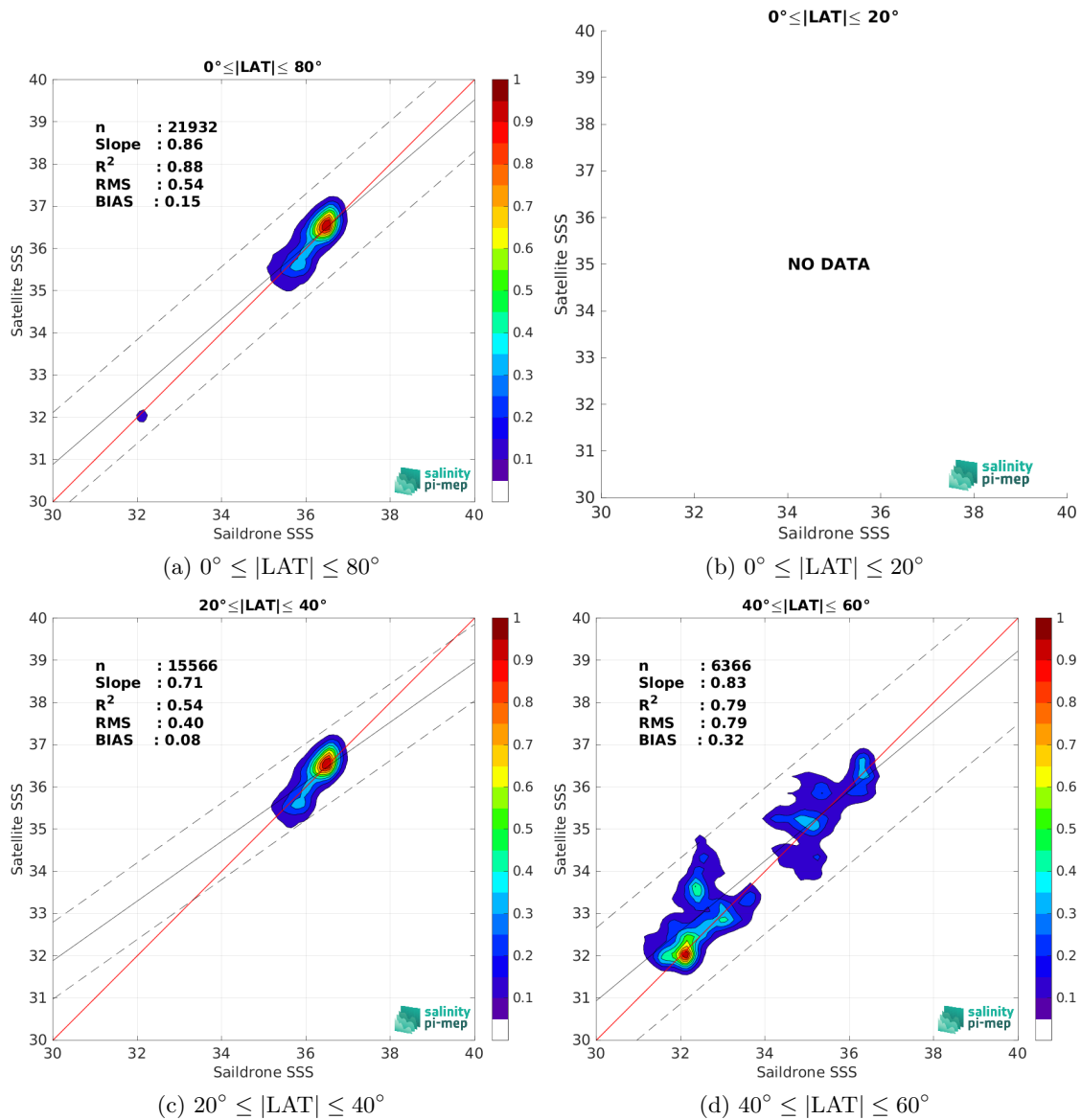
Figure 10: Contour maps of the concentration of SMOS SSS L3 v9 - 9 Days (CATDS-CEC-LOCEAN) SSS (y-axis) versus Sailldrone SSS (x-axis) at match-up pairs for different latitude bands. For each plot, the red line shows x=y . The black thin and dashed lines indicate a linear fit through the data cloud and the \pm 95\% confidence levels, respectively. The number match-up pairs n , the slope and R^2 coefficient of the linear fit, the root mean square (RMS) and the mean bias between satellite and in situ data are indicated for each latitude band in each plots.
