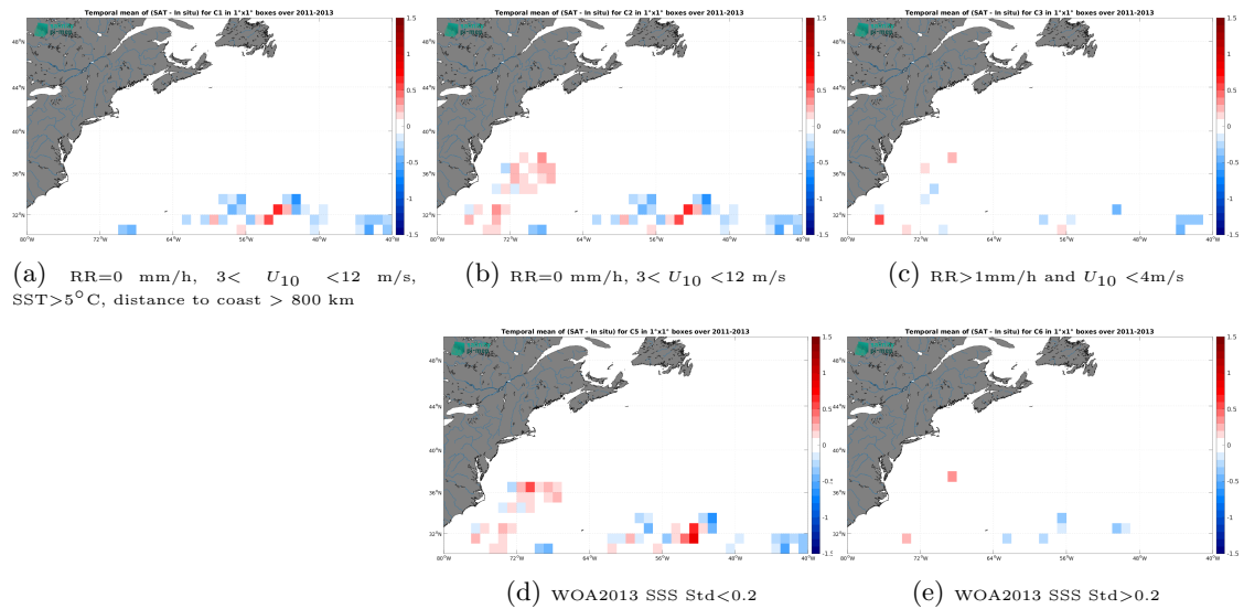
Figure 13: Temporal mean gridded over spatial boxes of size 1^\circ \times 1^\circ of \Delta SSS (SMOS SSS L3 v9 - 9 Days (CATDS-CEC-LOCEAN) - Surface drifters) for 5 different subdatasets corresponding to:RR=0 mm/h, 3 < U_{10} < 12 m/s, SST >5^\circ C, distance to coast > 800 km (a), RR=0 mm/h, 3 < U_{10} < 12 m/s (b), RR >1 mm/h and U_{10} < 4 m/s (c), WOA2013 SSS Std <0.2 (d), WOA2013 SSS Std >0.2 (e).
