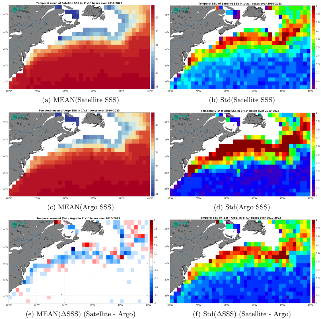
Figure 7: Temporal mean (left) and Std (right) of SSS from SMOS SSS L3 v9 - 9 Days (CATDS-CEC-LOCEAN) (top), Argo (middle), and of \Delta SSS (Satellite - Argo). Only match-up pairs are used to generate these maps.
