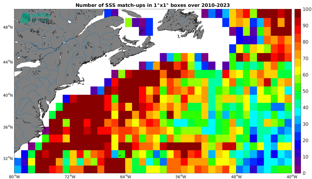
Figure 5: Number of SSS match-ups between Argo SSS and the SMOS SSS L3 v9 - 9 Days (CATDS-CEC-LOCEAN) SSS product for the Gulf Stream Pi-MEP region over 1^\circ \times 1^\circ boxes and for the full satellite product period.
