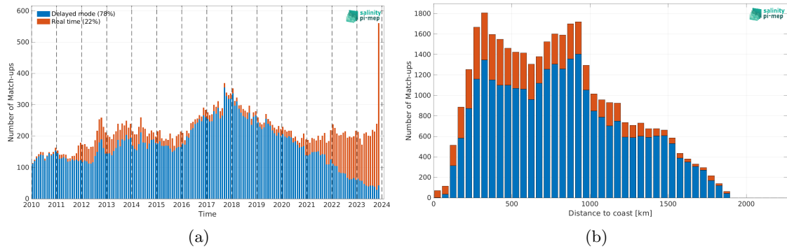
Figure 2: Number of match-ups between Argo and SMOS SSS L3 v9 - 9 Days (CATDS-CEC-LOCEAN) SSS as a function of time (a) and as function of the distance to coast (b) over the Gulf Stream Pi-MEP region and for the full satellite product period.
