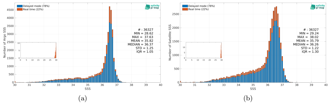
Figure 3: Histograms of SSS from Argo (a) and SMOS SSS L3 v9 - 9 Days (CATDS-CEC-LOCEAN) (b) considering all match-up pairs per bins of 0.1 over the Gulf Stream Pi-MEP region and for the full satellite product period.
