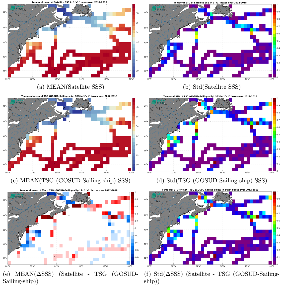
Figure 7: Temporal mean (left) and Std (right) of SSS from SMOS SSS L3 v9 - 18 Days (CATDS-CEC-LOCEAN) (top), TSG (GOSUD-Sailing-ship) (middle), and of \Delta SSS (Satellite - TSG (GOSUD-Sailing-ship)). Only match-up pairs are used to generate these maps.
