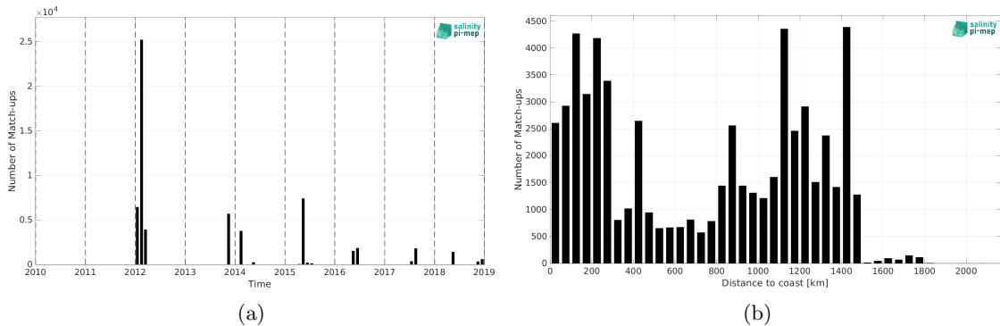
Figure 2: Number of match-ups between TSG (GOSUD-Sailing-ship) and SMOS SSS L3 v9 - 18 Days (CATDS-CEC-LOCEAN) SSS as a function of time (a) and as function of the distance to coast (b) over the Gulf Stream Pi-MEP region and for the full satellite product period.
