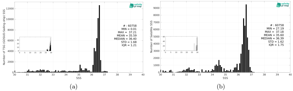
Figure 3: Histograms of SSS from TSG (GOSUD-Sailing-ship) (a) and SMOS SSS L3 v9 - 18 Days (CATDS-CEC-LOCEAN) (b) considering all match-up pairs per bins of 0.1 over the Gulf Stream Pi-MEP region and for the full satellite product period.
