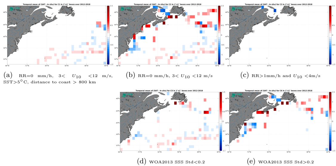
Figure 14: Temporal mean gridded over spatial boxes of size 1^\circ \times 1^\circ of \Delta SSS (SMOS SSS L3 v9 - 18 Days (CATDS-CEC-LOCEAN) - TSG (GOSUD-Sailing-ship)) for 5 different subdatasets corresponding to:RR=0 mm/h, 3 < U_{10} < 12 m/s, SST >5^\circ\text{C} , distance to coast > 800 km (a), RR=0 mm/h, 3 < U_{10} < 12 m/s (b), RR >1 mm/h and U_{10} < 4 m/s (c), WOA2013 SSS Std <0.2 (d), WOA2013 SSS Std >0.2 (e).
