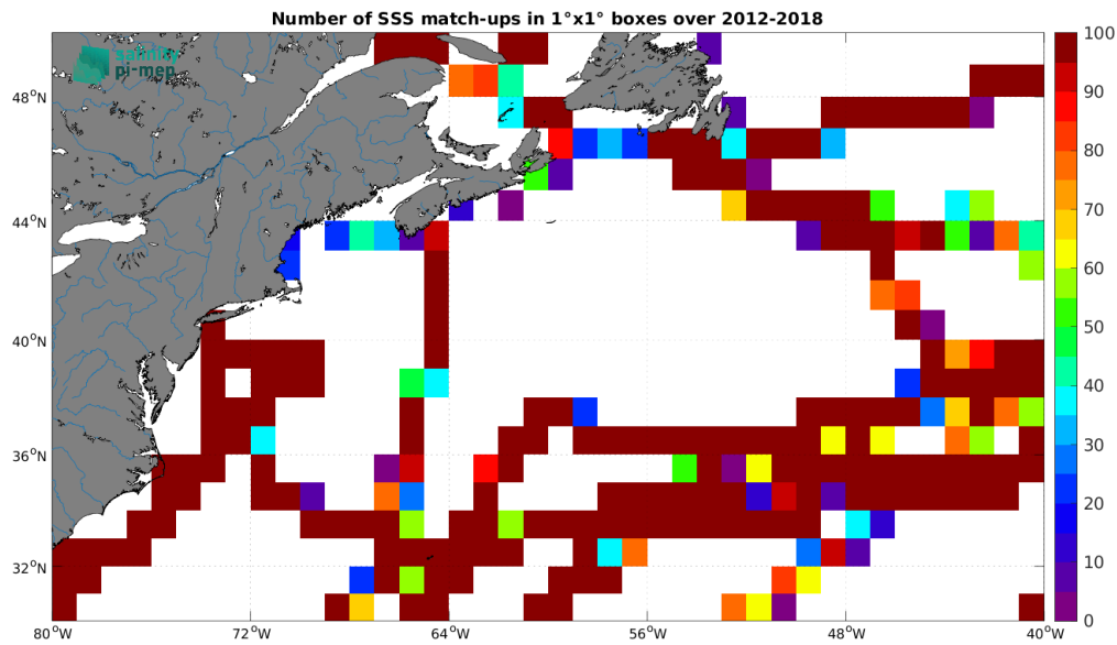
Figure 5: Number of SSS match-ups between TSG (GOSUD-Sailing-ship) SSS and the SMOS SSS L3 v9 - 18 Days (CATDS-CEC-LOCEAN) SSS product for the Gulf Stream Pi-MEP region over 1^\circ \times 1^\circ boxes and for the full satellite product period.
