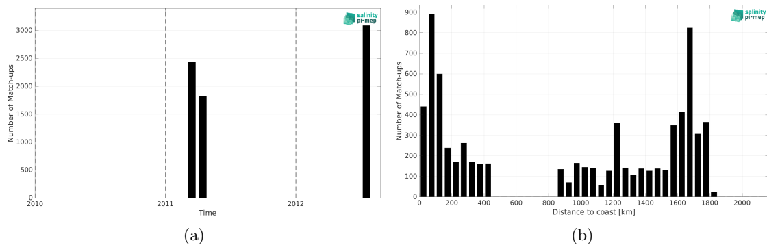
Figure 2: Number of match-ups between TSG (CSIC-UTM) and SMOS SSS L3 v9 - 18 Days (CATDS-CEC-LOCEAN) SSS as a function of time (a) and as function of the distance to coast (b) over the Gulf Stream Pi-MEP region and for the full satellite product period.
