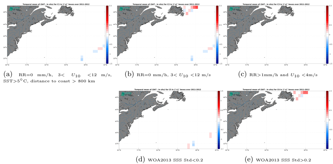
Figure 14: Temporal mean gridded over spatial boxes of size 1^\circ \times 1^\circ of \Delta SSS (SMOS SSS L3 v9 - 18 Days (CATDS-CEC-LOCEAN) - TSG (CSIC-UTM)) for 5 different subdatasets corresponding to:RR=0 mm/h, 3 < U_{10} < 12 m/s, SST>5°C, distance to coast > 800 km (a), RR=0 mm/h, 3 < U_{10} < 12 m/s (b), RR>1mm/h and U_{10} < 4 m/s (c), WOA2013 SSS Std<0.2 (d), WOA2013 SSS Std>0.2 (e).
