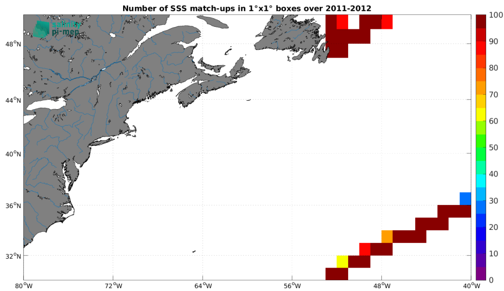
Figure 5: Number of SSS match-ups between TSG (CSIC-UTM) SSS and the SMOS SSS L3 v9 - 18 Days (CATDS-CEC-LOCEAN) SSS product for the Gulf Stream Pi-MEP region over 1^\circ \times 1^\circ boxes and for the full satellite product period.
