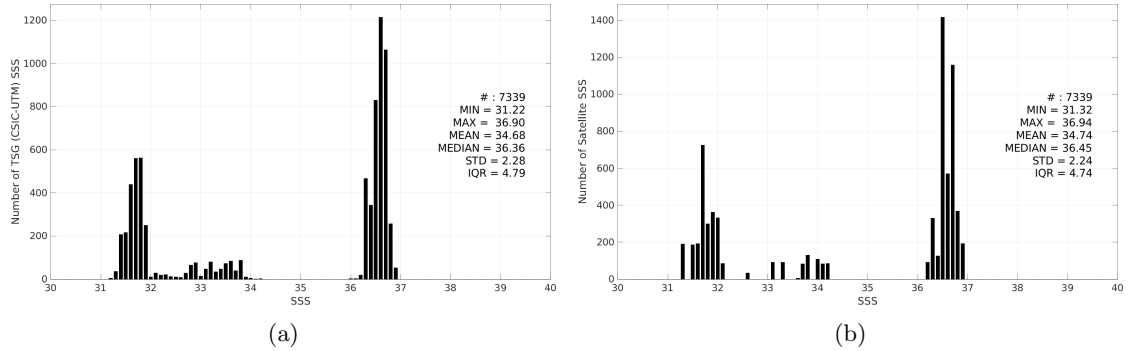
Figure 3: Histograms of SSS from TSG (CSIC-UTM) (a) and SMOS SSS L3 v9 - 18 Days (CATDS-CEC-LOCEAN) (b) considering all match-up pairs per bins of 0.1 over the Gulf Stream Pi-MEP region and for the full satellite product period.
