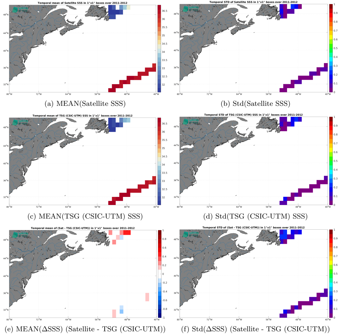
Figure 7: Temporal mean (left) and Std (right) of SSS from SMOS SSS L3 v9 - 18 Days (CATDS-CEC-LOCEAN) (top), TSG (CSIC-UTM) (middle), and of \Delta SSS (Satellite - TSG (CSIC-UTM)). Only match-up pairs are used to generate these maps.
