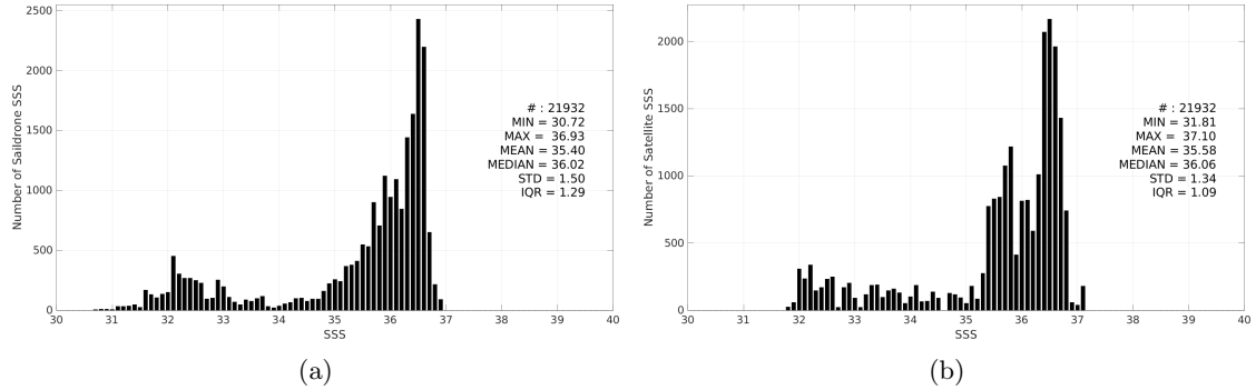
Figure 3: Histograms of SSS from Saildrone (a) and SMOS SSS L3 v9 - 18 Days (CATDS-CEC-LOCEAN) (b) considering all match-up pairs per bins of 0.1 over the Gulf Stream Pi-MEP region and for the full satellite product period.
