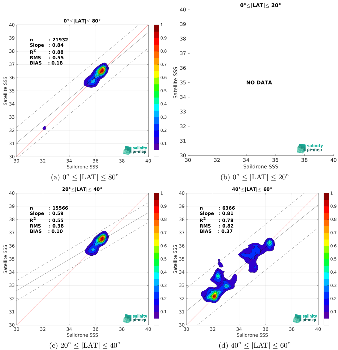
Figure 10: Contour maps of the concentration of SMOS SSS L3 v9 - 18 Days (CATDS-CEC-LOCEAN) SSS (y-axis) versus Sailldrone SSS (x-axis) at match-up pairs for different latitude bands. For each plot, the red line shows x=y . The black thin and dashed lines indicate a linear fit through the data cloud and the \pm 95\% confidence levels, respectively. The number match-up pairs n , the slope and R^2 coefficient of the linear fit, the root mean square (RMS) and the mean bias between satellite and in situ data are indicated for each latitude band in each plots.
