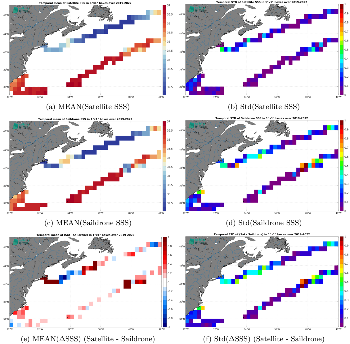
Figure 7: Temporal mean (left) and Std (right) of SSS from SMOS SSS L3 v9 - 18 Days (CATDS-CEC-LOCEAN) (top), Saildrone (middle), and of \Delta SSS (Satellite - Saildrone). Only match-up pairs are used to generate these maps.
