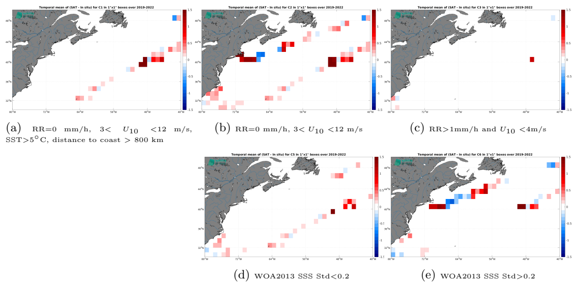
Figure 14: Temporal mean gridded over spatial boxes of size 1^\circ \times 1^\circ of \Delta SSS (SMOS SSS L3 v9 - 18 Days (CATDS-CEC-LOCEAN) - Sailydrone) for 5 different subdatasets corresponding to:RR=0 mm/h, 3 < U_{10} < 12 m/s, SST>5°C, distance to coast > 800 km (a), RR=0 mm/h, 3 < U_{10} < 12 m/s (b), RR>1mm/h and U_{10} < 4 m/s (c), WOA2013 SSS Std<0.2 (d), WOA2013 SSS Std>0.2 (e).
