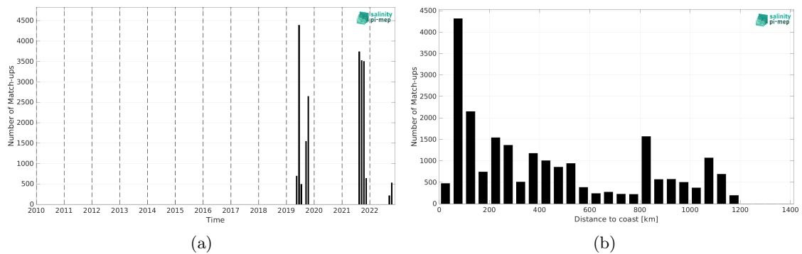
Figure 2: Number of match-ups between Saildrone and SMOS SSS L3 v9 - 18 Days (CATDS-CEC-LOCEAN) SSS as a function of time (a) and as function of the distance to coast (b) over the Gulf Stream Pi-MEP region and for the full satellite product period.
