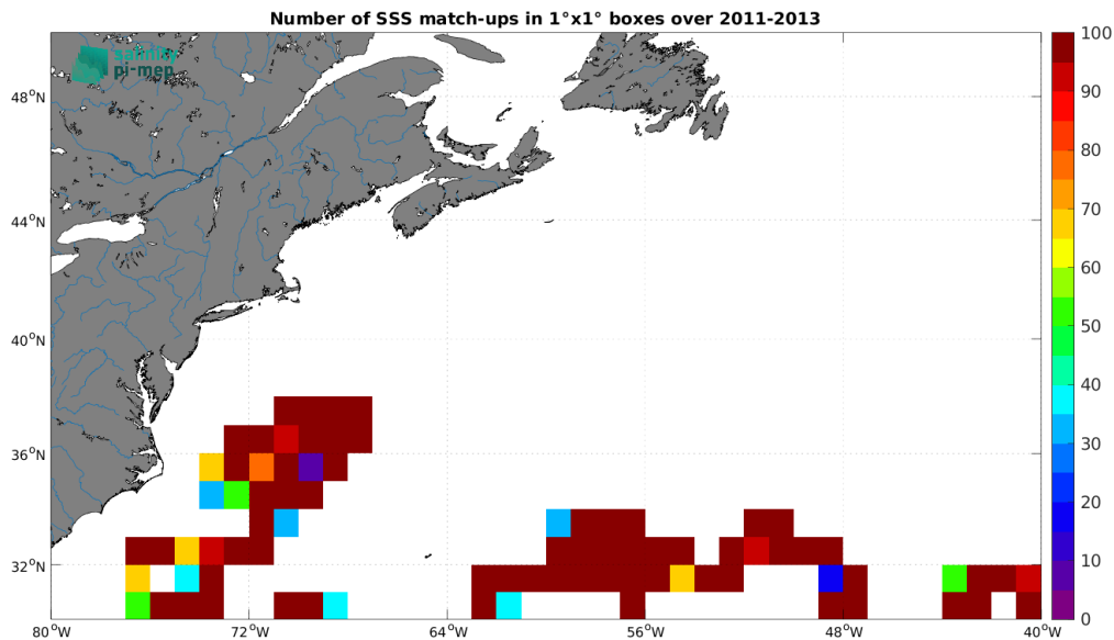
Figure 4: Number of SSS match-ups between Surface drifters SSS and the SMOS SSS L3 v9 - 18 Days (CATDS-CEC-LOCEAN) SSS product for the Gulf Stream Pi-MEP region over 1^\circ \times 1^\circ boxes and for the full satellite product period.
