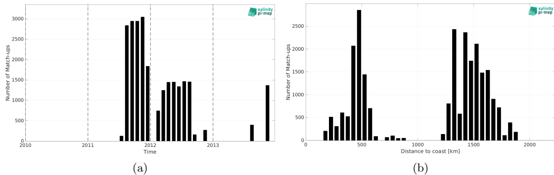
Figure 2: Number of match-ups between Surface drifters and SMOS SSS L3 v9 - 18 Days (CATDS-CEC-LOCEAN) SSS as a function of time (a) and as function of the distance to coast (b) over the Gulf Stream Pi-MEP region and for the full satellite product period.
