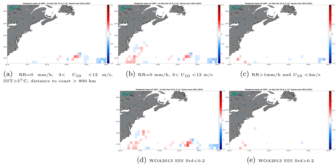
Figure 13: Temporal mean gridded over spatial boxes of size 1^\circ \times 1^\circ of \Delta SSS (SMOS SSS L3 v9 - 18 Days (CATDS-CEC-LOCEAN) - Surface drifters) for 5 different subdatasets corresponding to:RR=0 mm/h, 3 < U_{10} < 12 m/s, SST >5^\circ C, distance to coast > 800 km (a), RR=0 mm/h, 3 < U_{10} < 12 m/s (b), RR >1 mm/h and U_{10} < 4 m/s (c), WOA2013 SSS Std <0.2 (d), WOA2013 SSS Std >0.2 (e).
