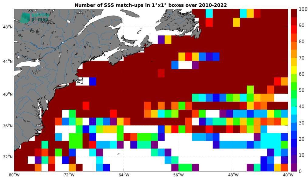
Figure 4: Number of SSS match-ups between TSG (LEGOS-DM) SSS and the SMOS SSS L3 v8 - 9 Days (CATDS-CEC-LOCEAN) SSS product for the Gulf Stream Pi-MEP region over 1^\circ \times 1^\circ boxes and for the full satellite product period.
