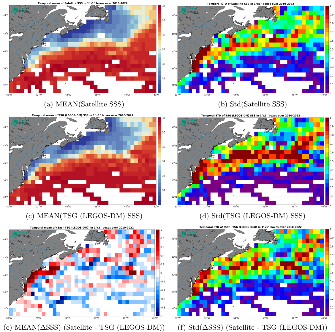
Figure 6: Temporal mean (left) and Std (right) of SSS from SMOS SSS L3 v8 - 9 Days (CATDS-CEC-LOCEAN) (top), TSG (LEGOS-DM) (middle), and of \Delta SSS (Satellite - TSG (LEGOS-DM)). Only match-up pairs are used to generate these maps.
