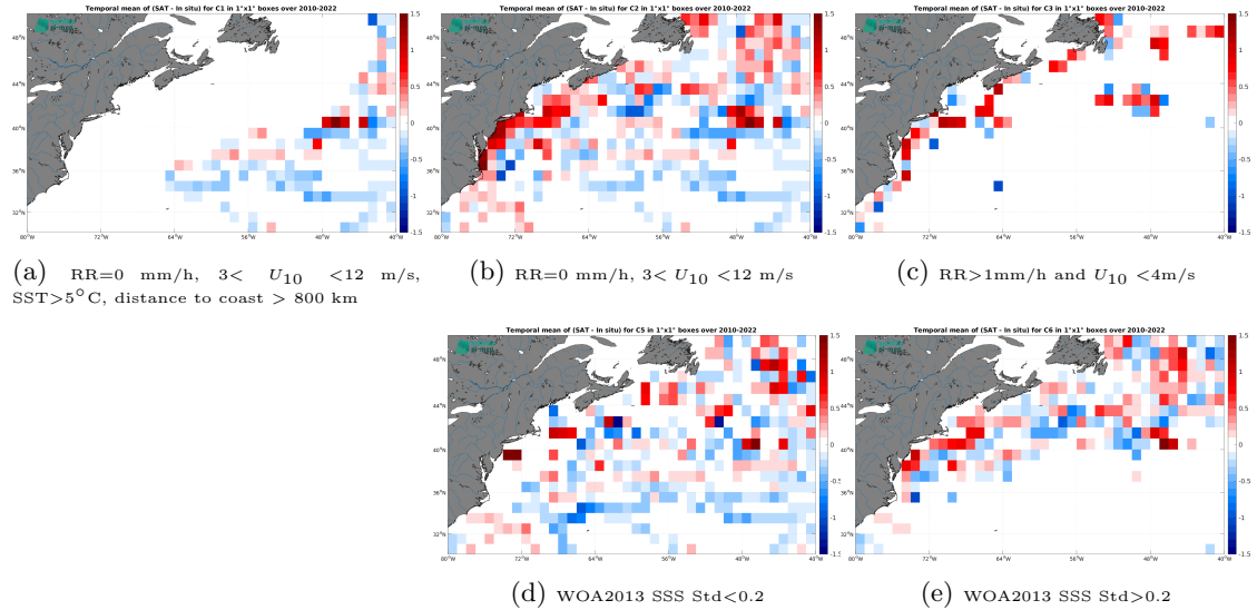
Figure 12: Temporal mean gridded over spatial boxes of size 1^{\circ}\times 1^{\circ} of \Delta\text{SSS} (SMOS SSS L3 v8 - 9 Days (CATDS-CEC-LOCEAN) - TSG (LEGOS-DM)) for 5 different subdatasets corresponding to:RR=0 mm/h, 3 < U_{10} < 12 m/s, SST >5^{\circ}\text{C} , distance to coast > 800 km (a), RR=0 mm/h, 3 < U_{10} < 12 m/s (b), RR >1 mm/h and U_{10} < 4 m/s (c), WOA2013 SSS Std <0.2 (d), WOA2013 SSS Std >0.2 (e).
