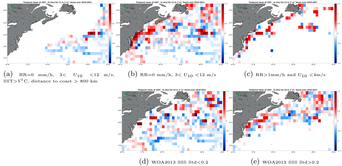
Figure 12: Temporal mean gridded over spatial boxes of size 1^{\circ}\times 1^{\circ} of \Delta\text{SSS} (SMOS SSS L3 v8 - 9 Days (CATDS-CECOS-LOCEAN) - TSG (LEGOS-DM)) for 5 different subdatasets corresponding to:RR=0 mm/h, 3 < U_{10} < 12 m/s, SST >5^{\circ}\text{C} , distance to coast > 800 km (a), RR=0 mm/h, 3 < U_{10} < 12 m/s (b), RR >1 mm/h and U_{10} < 4 m/s (c), WOA2013 SSS Std <0.2 (d), WOA2013 SSS Std >0.2 (e).
