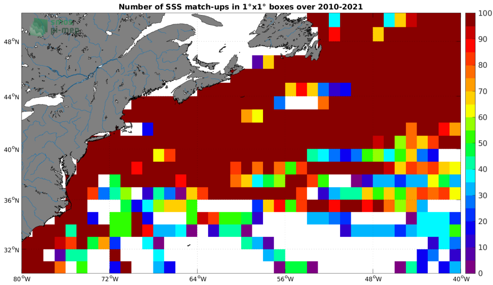
Figure 4: Number of SSS match-ups between TSG (LEGOS-DM) SSS and the SMOS SSS L3 v8 - 9 Days (CATDS-CECOS-LOCEAN) SSS product for the Gulf Stream Pi-MEP region over 1^\circ \times 1^\circ boxes and for the full satellite product period.
