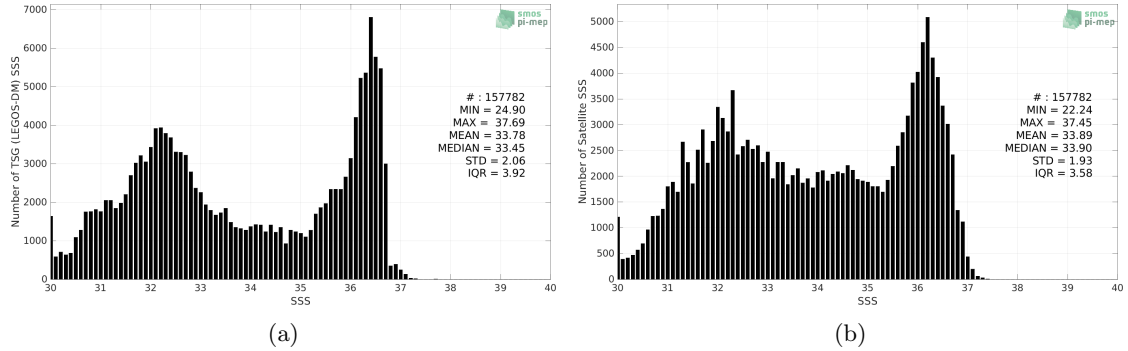
Figure 2: Histograms of SSS from TSG (LEGOS-DM) (a) and SMOS SSS L3 v8 - 9 Days (CATDS-CECOS-LOCEAN) (b) considering all match-up pairs per bins of 0.1 over the Gulf Stream Pi-MEP region and for the full satellite product period.
