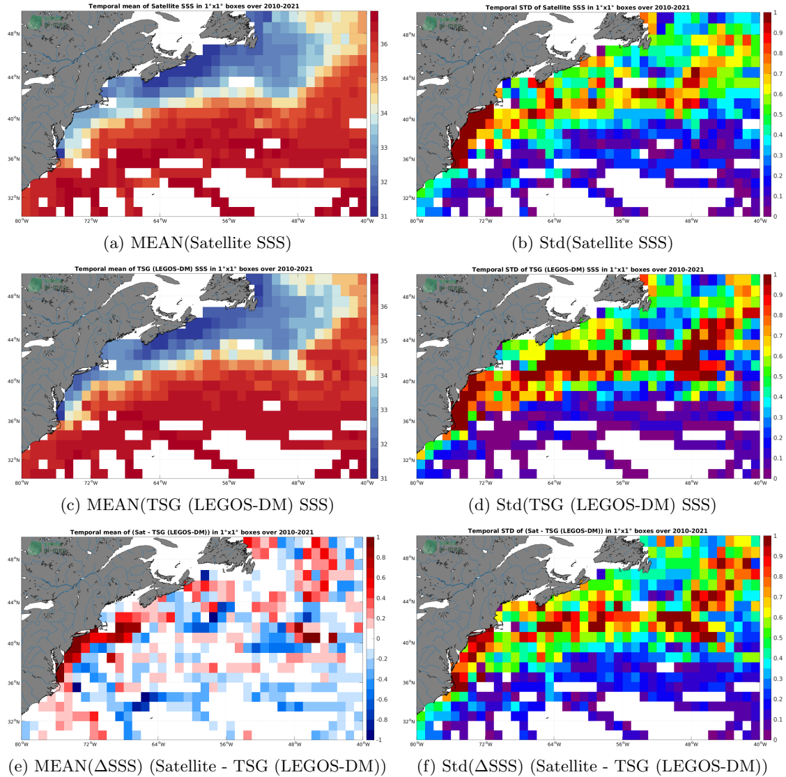
Figure 6: Temporal mean (left) and Std (right) of SSS from SMOS SSS L3 v8 - 9 Days (CATDS-CECOS-LOCEAN) (top), TSG (LEGOS-DM) (middle), and of \Delta SSS (Satellite - TSG (LEGOS-DM)). Only match-up pairs are used to generate these maps.
