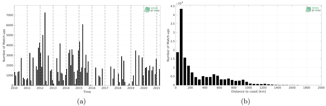
Figure 1: Number of match-ups between TSG (LEGOS-DM) and SMOS SSS L3 v8 - 9 Days (CATDS-CECOS-LOCEAN) SSS as a function of time (a) and as function of the distance to coast (b) over the Gulf Stream Pi-MEP region and for the full satellite product period.
