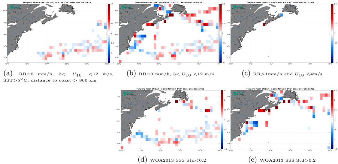
Figure 12: Temporal mean gridded over spatial boxes of size 1^{\circ}\times 1^{\circ} of \Delta SSS (SMOS SSS L3 v8 - 9 Days (CATDS-CEC-LOCEAN) - TSG (GOSUD-Sailing-ship)) for 5 different subdatasets corresponding to:RR=0 mm/h, 3 < U_{10} < 12 m/s, SST >5^{\circ}\text{C} , distance to coast > 800 km (a), RR=0 mm/h, 3 < U_{10} < 12 m/s (b), RR >1 mm/h and U_{10} < 4 m/s (c), WOA2013 SSS Std <0.2 (d), WOA2013 SSS Std >0.2 (e).
