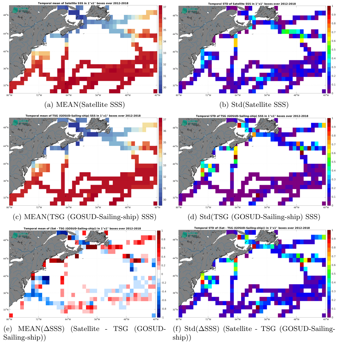
Figure 6: Temporal mean (left) and Std (right) of SSS from SMOS SSS L3 v8 - 9 Days (CATDS-CEC-LOCEAN) (top), TSG (GOSUD-Sailing-ship) (middle), and of \Delta SSS (Satellite - TSG (GOSUD-Sailing-ship)). Only match-up pairs are used to generate these maps.
