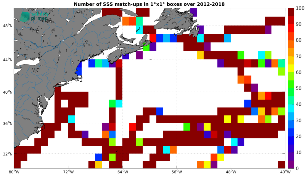
Figure 4: Number of SSS match-ups between TSG (GOSUD-Sailing-ship) SSS and the SMOS SSS L3 v8 - 9 Days (CATDS-CEC-LOCEAN) SSS product for the Gulf Stream Pi-MEP region over 1^\circ \times 1^\circ boxes and for the full satellite product period.
