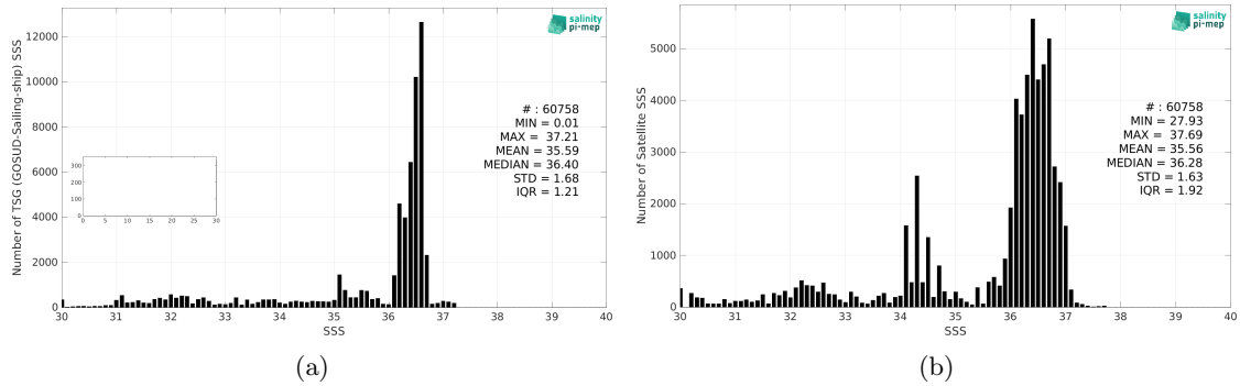
Figure 2: Histograms of SSS from TSG (GOSUD-Sailing-ship) (a) and SMOS SSS L3 v8 - 9 Days (CATDS-CEC-LOCEAN) (b) considering all match-up pairs per bins of 0.1 over the Gulf Stream Pi-MEP region and for the full satellite product period.
