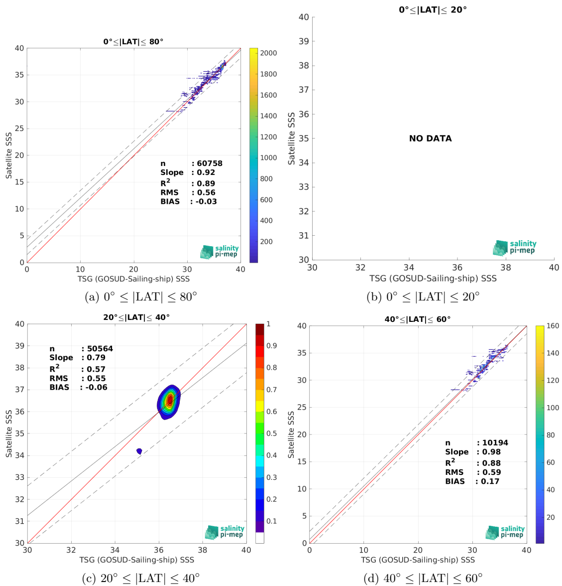
Figure 9: Contour maps of the concentration of SMOS SSS L3 v8 - 9 Days (CATDS-CEC-LOCEAN) SSS (y-axis) versus TSG (GOSUD-Sailing-ship) SSS (x-axis) at match-up pairs for different latitude bands. For each plot, the red line shows x=y . The black thin and dashed lines indicate a linear fit through the data cloud and the \pm 95\% confidence levels, respectively. The number match-up pairs n , the slope and R^2 coefficient of the linear fit, the root mean square (RMS) and the mean bias between satellite and in situ data are indicated for each latitude band in each plots.
