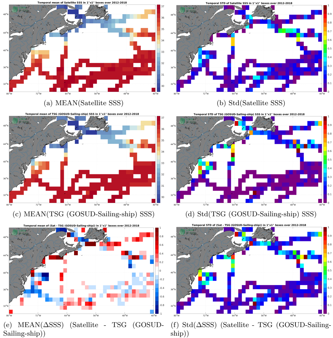
Figure 6: Temporal mean (left) and Std (right) of SSS from SMOS SSS L3 v8 - 9 Days (CATDS-CECOS-LOCEAN) (top), TSG (GOSUD-Sailing-ship) (middle), and of \Delta SSS (Satellite - TSG (GOSUD-Sailing-ship)). Only match-up pairs are used to generate these maps.
