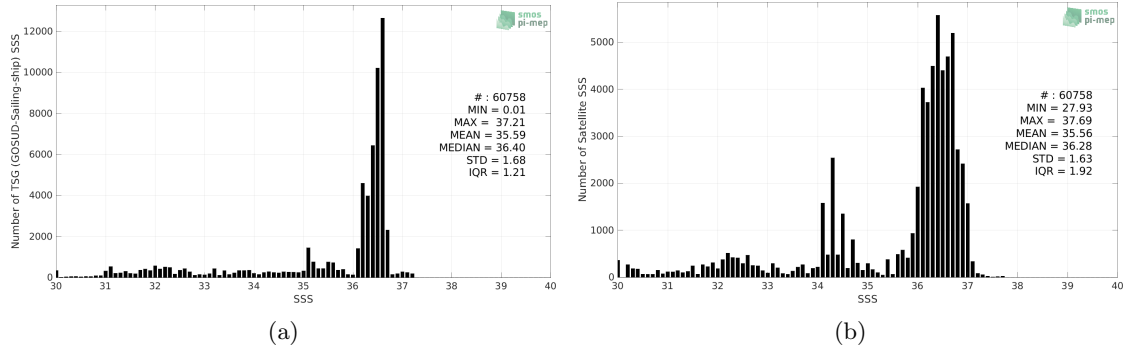
Figure 2: Histograms of SSS from TSG (GOSUD-Sailing-ship) (a) and SMOS SSS L3 v8 - 9 Days (CATDS-CECOS-LOCEAN) (b) considering all match-up pairs per bins of 0.1 over the Gulf Stream Pi-MEP region and for the full satellite product period.
