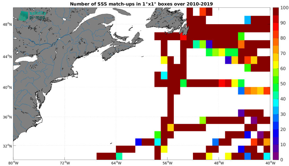
Figure 4: Number of SSS match-ups between TSG (GOSUD-Research-vessel) SSS and the SMOS SSS L3 v8 - 9 Days (CATDS-CEC-LOCEAN) SSS product for the Gulf Stream Pi-MEP region over 1^\circ \times 1^\circ boxes and for the full satellite product period.
