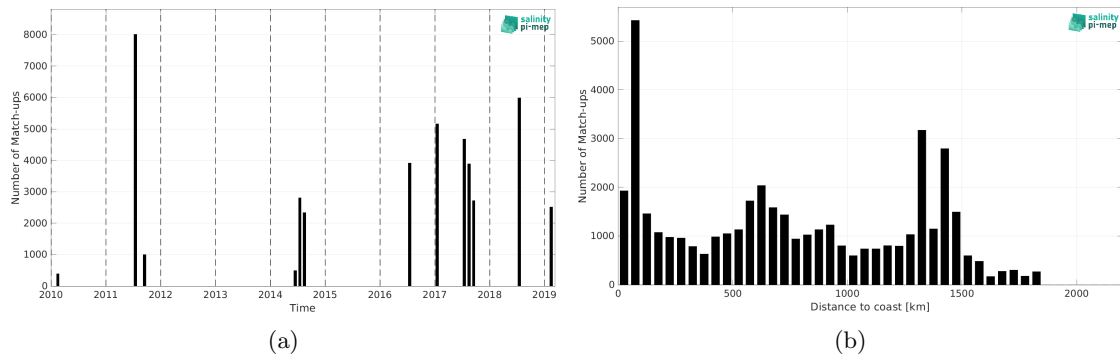
Figure 1: Number of match-ups between TSG (GOSUD-Research-vessel) and SMOS SSS L3 v8 - 9 Days (CATDS-CEC-LOCEAN) SSS as a function of time (a) and as function of the distance to coast (b) over the Gulf Stream Pi-MEP region and for the full satellite product period.
