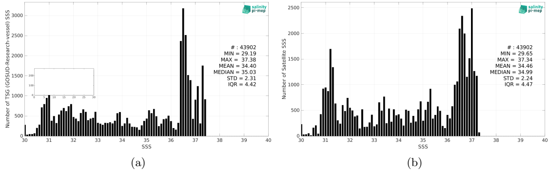
Figure 2: Histograms of SSS from TSG (GOSUD-Research-vessel) (a) and SMOS SSS L3 v8 - 9 Days (CATDS-CEC-LOCEAN) (b) considering all match-up pairs per bins of 0.1 over the Gulf Stream Pi-MEP region and for the full satellite product period.
