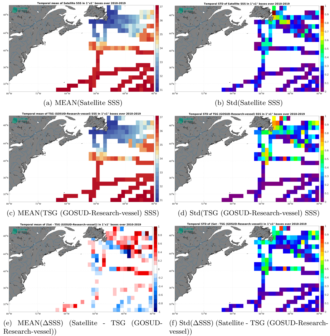
Figure 6: Temporal mean (left) and Std (right) of SSS from SMOS SSS L3 v8 - 9 Days (CATDS-CEC-LOCEAN) (top), TSG (GOSUD-Research-vessel) (middle), and of \Delta SSS (Satellite - TSG (GOSUD-Research-vessel)). Only match-up pairs are used to generate these maps.
