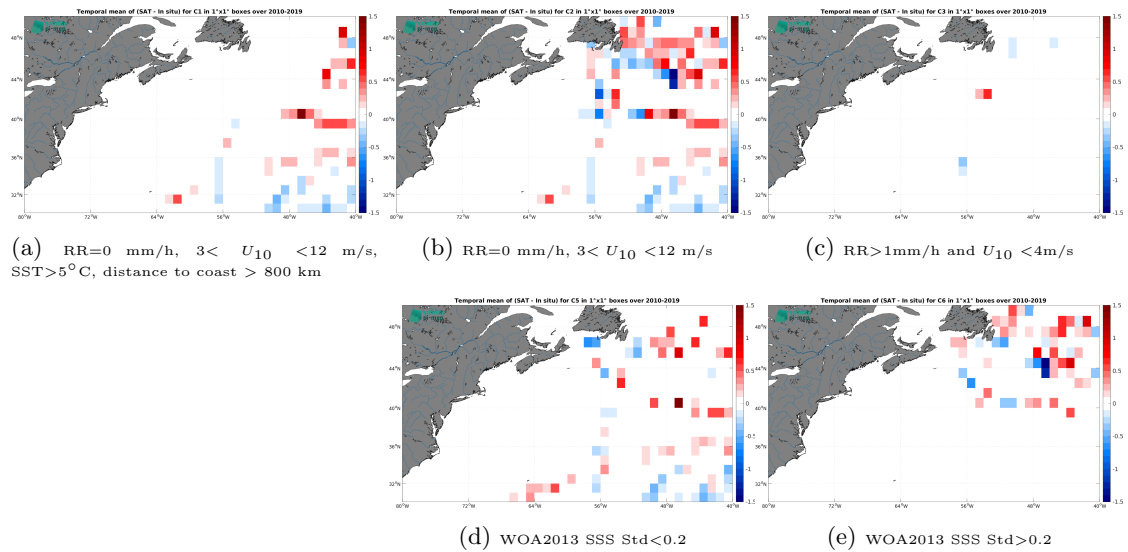
Figure 12: Temporal mean gridded over spatial boxes of size 1^\circ \times 1^\circ of \Delta SSS (SMOS SSS L3 v8 - 9 Days (CATDS-CEC-LOCEAN) - TSG (GOSUD-Research-vessel)) for 5 different subdatasets corresponding to: RR=0 mm/h, 3 < U_{10} < 12 m/s, SST > 5^\circ\text{C} , distance to coast > 800 km (a), RR=0 mm/h, 3 < U_{10} < 12 m/s (b), RR > 1 mm/h and U_{10} < 4 m/s (c), WOA2013 SSS Std < 0.2 (d), WOA2013 SSS Std > 0.2 (e).
