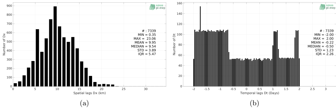
Figure 5: Histograms of the spatial (a) and temporal (b) lags between the location/time of the TSG (CSIC-UTM) measurement and the date of the corresponding SMOS SSS L3 v8 - 9 Days (CATDS-CECOS-LOCEAN) SSS pixel.
