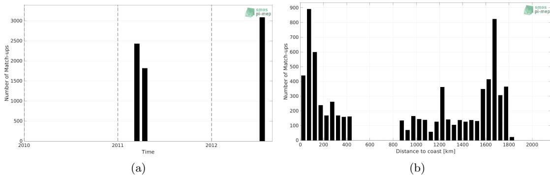
Figure 1: Number of match-ups between TSG (CSIC-UTM) and SMOS SSS L3 v8 - 9 Days (CATDS-CECOS-LOCEAN) SSS as a function of time (a) and as function of the distance to coast (b) over the Gulf Stream Pi-MEP region and for the full satellite product period.
