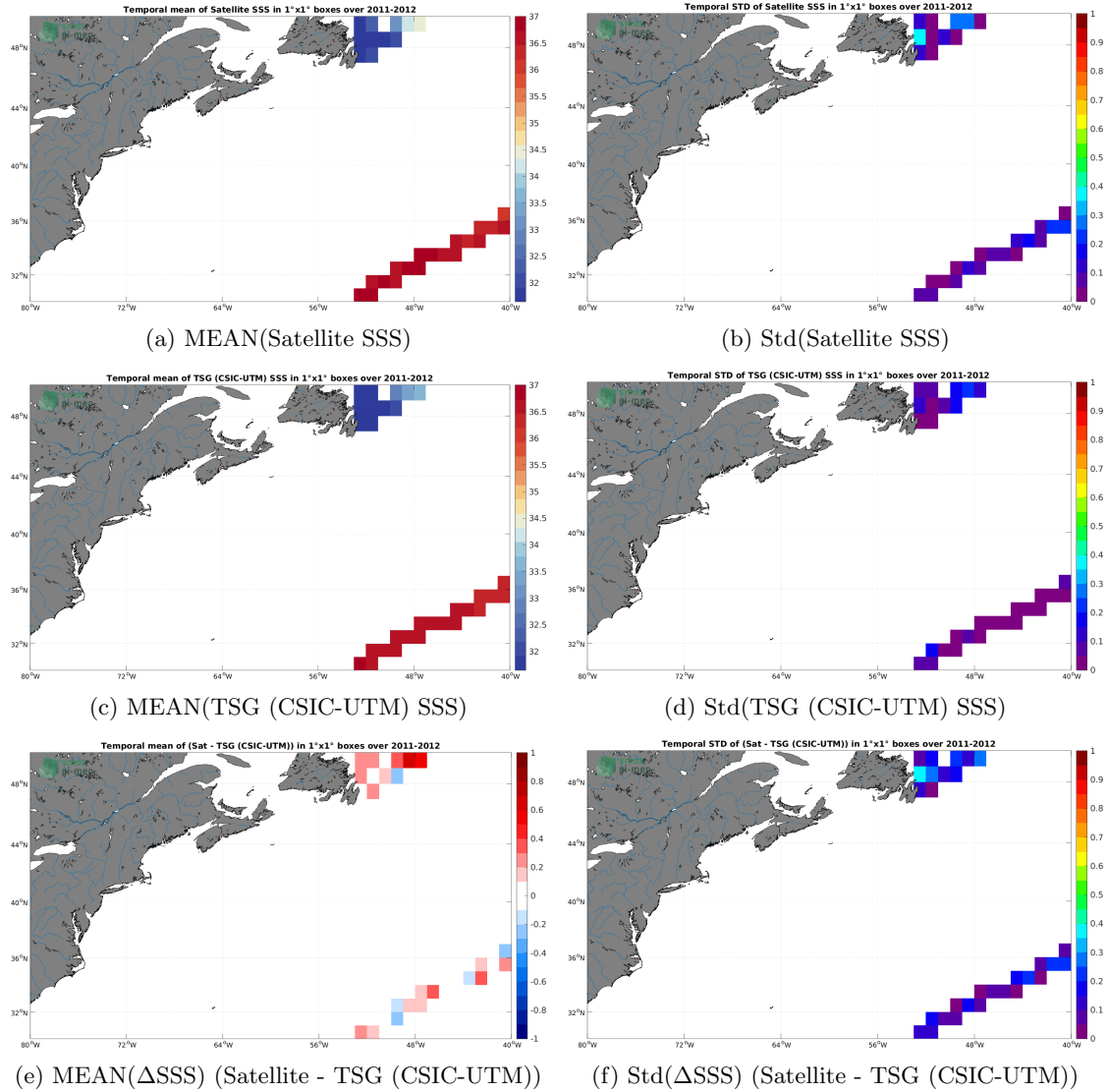
Figure 6: Temporal mean (left) and Std (right) of SSS from SMOS SSS L3 v8 - 9 Days (CATDS-CECOS-LOCEAN) (top), TSG (CSIC-UTM) (middle), and of \Delta SSS (Satellite - TSG (CSIC-UTM)). Only match-up pairs are used to generate these maps.
