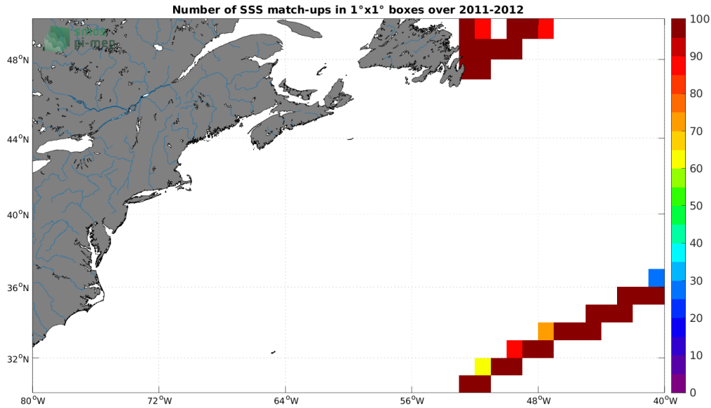
Figure 4: Number of SSS match-ups between TSG (CSIC-UTM) SSS and the SMOS SSS L3 v8 - 9 Days (CATDS-CECOS-LOCEAN) SSS product for the Gulf Stream Pi-MEP region over 1^{\circ} \times 1^{\circ} boxes and for the full satellite product period.
