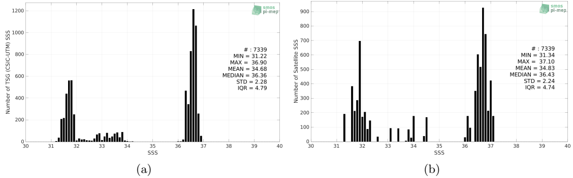
Figure 2: Histograms of SSS from TSG (CSIC-UTM) (a) and SMOS SSS L3 v8 - 9 Days (CATDS-CECOS-LOCEAN) (b) considering all match-up pairs per bins of 0.1 over the Gulf Stream Pi-MEP region and for the full satellite product period.
