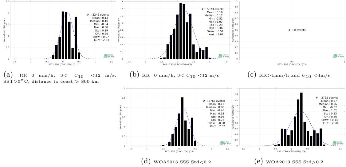
Figure 13: Normalized histogram of \Delta\text{SSS} (SMOS SSS L3 v8 - 9 Days (CATDS-CECOS-LOCEAN) - TSG (CSIC-UTM)) for 5 different subdatasets corresponding to: RR=0 mm/h, 3 < U_{10} < 12 m/s, SST > 5^\circ\text{C} , distance to coast > 800 km (a), RR=0 mm/h, 3 < U_{10} < 12 m/s (b), RR > 1\text{mm/h} and U_{10} < 4\text{m/s} (c), WOA2013 SSS Std < 0.2 (d), WOA2013 SSS Std > 0.2 (e).
