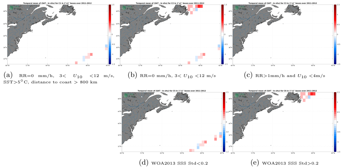
Figure 12: Temporal mean gridded over spatial boxes of size 1^{\circ}\times 1^{\circ} of \Delta\text{SSS} (SMOS SSS L3 v8 - 9 Days (CATDS-CECOS-LOCEAN) - TSG (CSIC-UTM)) for 5 different subdatasets corresponding to:RR=0 mm/h, 3 < U_{10} < 12 m/s, SST >5^{\circ}\text{C} , distance to coast > 800 km (a), RR=0 mm/h, 3 < U_{10} < 12 m/s (b), RR >1 mm/h and U_{10} < 4 m/s (c), WOA2013 SSS Std <0.2 (d), WOA2013 SSS Std >0.2 (e).
