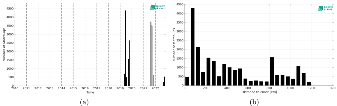
Figure 1: Number of match-ups between Saildrone and SMOS SSS L3 v8 - 9 Days (CATDS-CEC-LOCEAN) SSS as a function of time (a) and as function of the distance to coast (b) over the Gulf Stream Pi-MEP region and for the full satellite product period.
