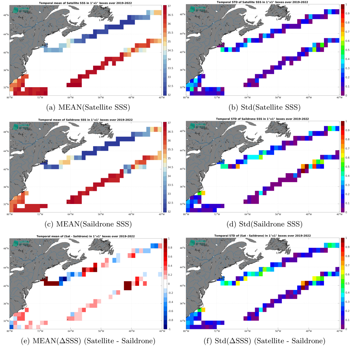
Figure 6: Temporal mean (left) and Std (right) of SSS from SMOS SSS L3 v8 - 9 Days (CATDS-CEC-LOCEAN) (top), Saildrone (middle), and of \Delta SSS (Satellite - Saildrone). Only match-up pairs are used to generate these maps.
