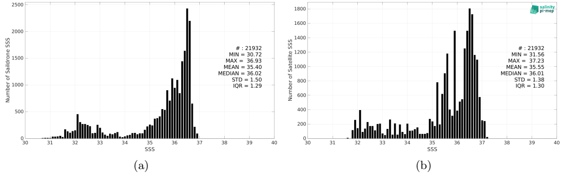
Figure 2: Histograms of SSS from Saildrone (a) and SMOS SSS L3 v8 - 9 Days (CATDS-CEC-LOCEAN) (b) considering all match-up pairs per bins of 0.1 over the Gulf Stream Pi-MEP region and for the full satellite product period.
