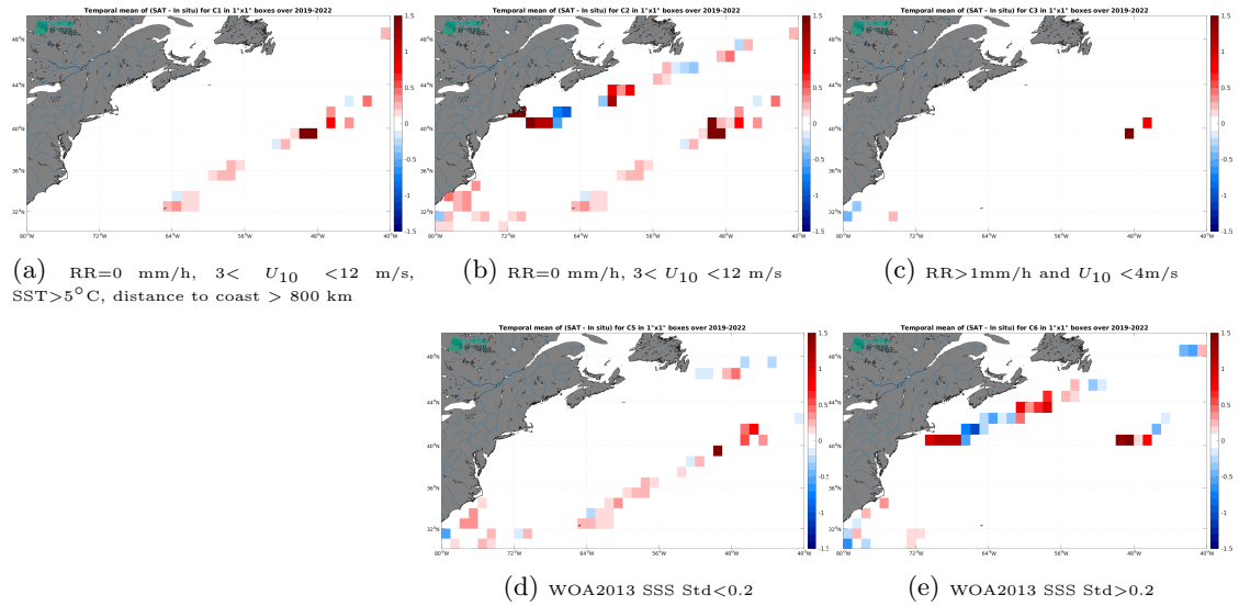
Figure 12: Temporal mean gridded over spatial boxes of size 1^\circ \times 1^\circ of \Delta SSS (SMOS SSS L3 v8 - 9 Days (CATDS-CEC-LOCEAN) - Saildrone) for 5 different subdatasets corresponding to:RR=0 mm/h, 3 < U_{10} < 12 m/s, SST >5^\circ C, distance to coast > 800 km (a), RR=0 mm/h, 3 < U_{10} < 12 m/s (b), RR >1 mm/h and U_{10} < 4 m/s (c), WOA2013 SSS Std <0.2 (d), WOA2013 SSS Std >0.2 (e).
