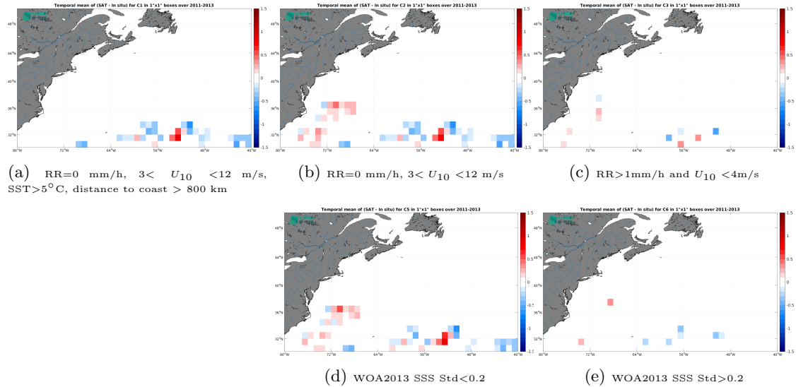
Figure 11: Temporal mean gridded over spatial boxes of size 1^{\circ}\times 1^{\circ} of \Delta\text{SSS} (SMOS SSS L3 v8 - 9 Days (CATDS-CEC-LOCEAN) - Surface drifters) for 5 different subdatasets corresponding to:RR=0 mm/h, 3 < U_{10} < 12 m/s, SST >5^{\circ}\text{C} , distance to coast > 800 km (a), RR=0 mm/h, 3 < U_{10} < 12 m/s (b), RR >1 mm/h and U_{10} < 4 m/s (c), WOA2013 SSS Std <0.2 (d), WOA2013 SSS Std >0.2 (e).
