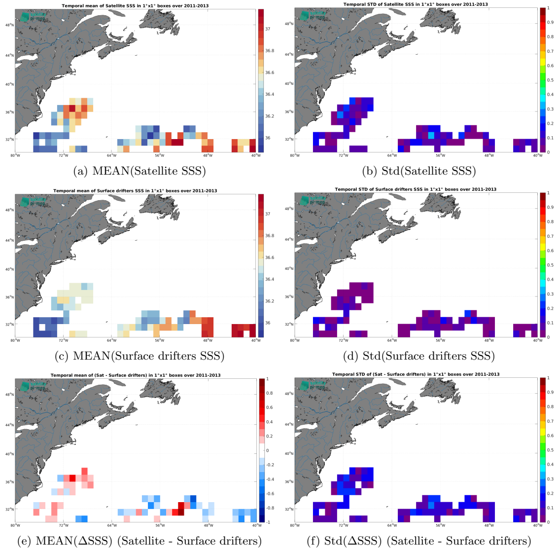
Figure 5: Temporal mean (left) and Std (right) of SSS from SMOS SSS L3 v8 - 9 Days (CATDS-CEC-LOCEAN) (top), Surface drifters (middle), and of \Delta SSS (Satellite - Surface drifters). Only match-up pairs are used to generate these maps.
