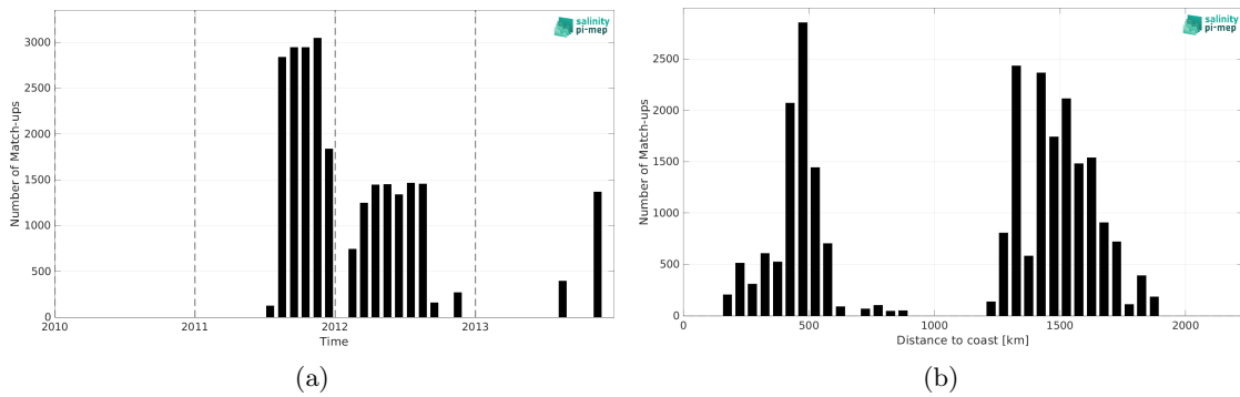
Figure 1: Number of match-ups between Surface drifters and SMOS SSS L3 v8 - 9 Days (CATDS-CEC-LOCEAN) SSS as a function of time (a) and as function of the distance to coast (b) over the Gulf Stream Pi-MEP region and for the full satellite product period.
