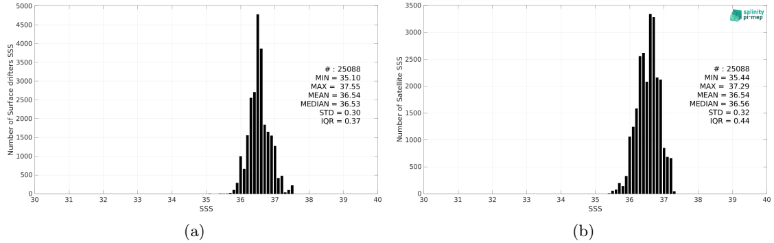
Figure 2: Histograms of SSS from Surface drifters (a) and SMOS SSS L3 v8 - 9 Days (CATDS-CEC-LOCEAN) (b) considering all match-up pairs per bins of 0.1 over the Gulf Stream Pi-MEP region and for the full satellite product period.
