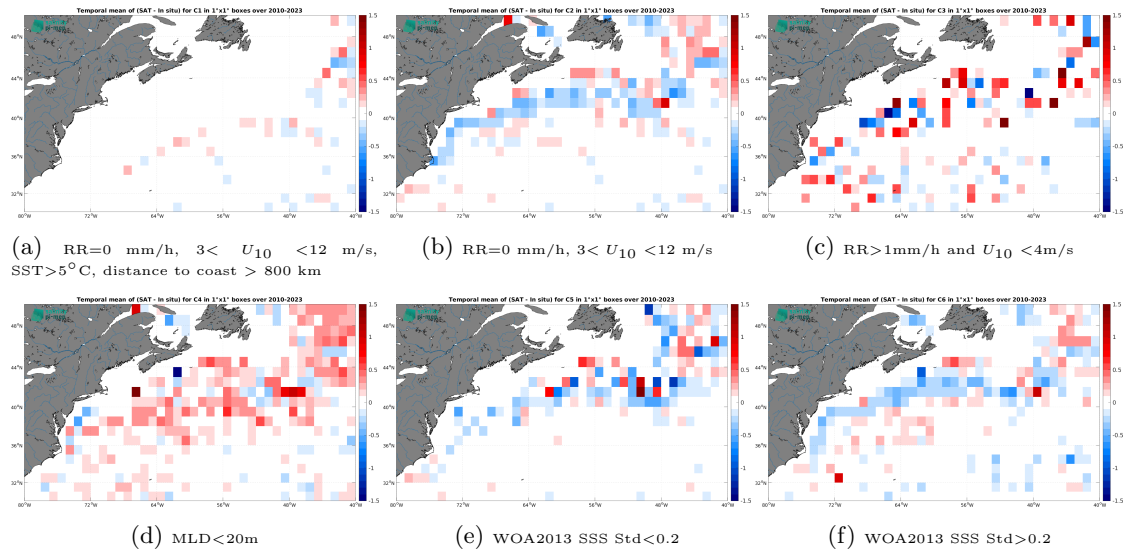
Figure 12: Temporal mean gridded over spatial boxes of size 1^\circ \times 1^\circ of \Delta SSS (SMOS SSS L3 v8 - 9 Days (CATDS-CEC-LOCEAN) - Argo) for 6 different subdatasets corresponding to:RR=0 mm/h, 3 < U_{10} < 12 m/s, SST > 5^\circ\text{C} , distance to coast > 800 km (a), RR=0 mm/h, 3 < U_{10} < 12 m/s (b), RR > 1 mm/h and U_{10} < 4 m/s (c),MLD < 20 m (d),WOA2013 SSS Std < 0.2 (e),WOA2013 SSS Std > 0.2 (f).
