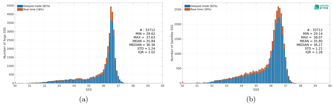
Figure 2: Histograms of SSS from Argo (a) and SMOS SSS L3 v8 - 9 Days (CATDS-CEC-LOCEAN) (b) considering all match-up pairs per bins of 0.1 over the Gulf Stream Pi-MEP region and for the full satellite product period.
