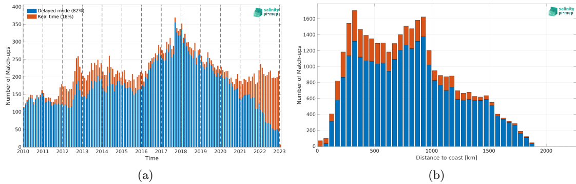
Figure 1: Number of match-ups between Argo and SMOS SSS L3 v8 - 9 Days (CATDS-CEC-LOCEAN) SSS as a function of time (a) and as function of the distance to coast (b) over the Gulf Stream Pi-MEP region and for the full satellite product period.
