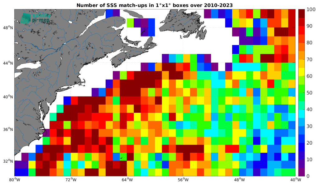
Figure 4: Number of SSS match-ups between Argo SSS and the SMOS SSS L3 v8 - 9 Days (CATDS-CEC-LOCEAN) SSS product for the Gulf Stream Pi-MEP region over 1^\circ \times 1^\circ boxes and for the full satellite product period.
