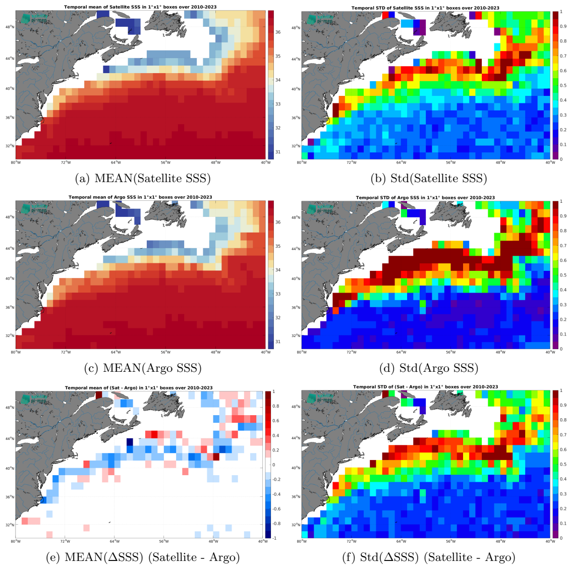
Figure 6: Temporal mean (left) and Std (right) of SSS from SMOS SSS L3 v8 - 9 Days (CATDS-CEC-LOCEAN) (top), Argo (middle), and of \Delta SSS (Satellite - Argo). Only match-up pairs are used to generate these maps.
